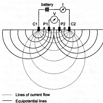
Figure 14 Schematic drawing of the Wenner electrode configuration used for EER surveys. The apparent resistivity is 2\pi a V/I , where a = distance between electrodes, V = voltage, and I = electrical current (Larson 1994).
