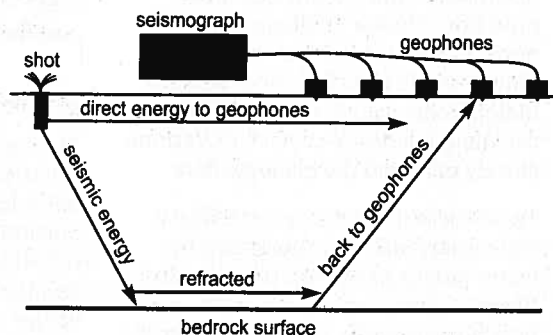
Figure 12 Schematic of the seismic refraction method.
