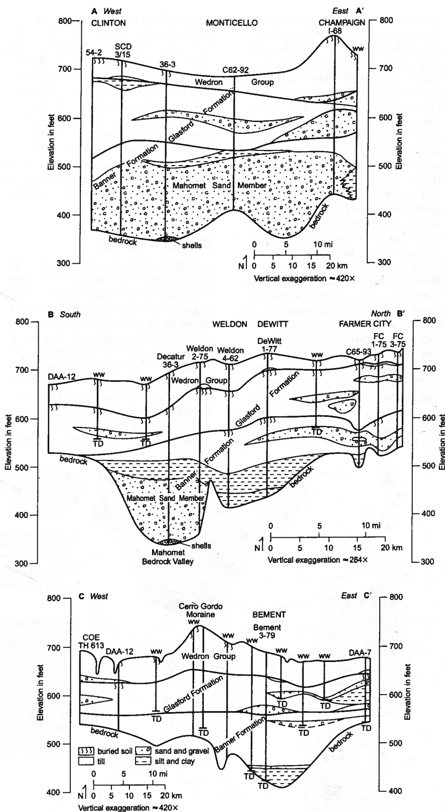
Figure 5 Three generalized cross sections of glacial deposits in the study area (Kempton and Herzog 1996). TD, total depth; ww, water well.
