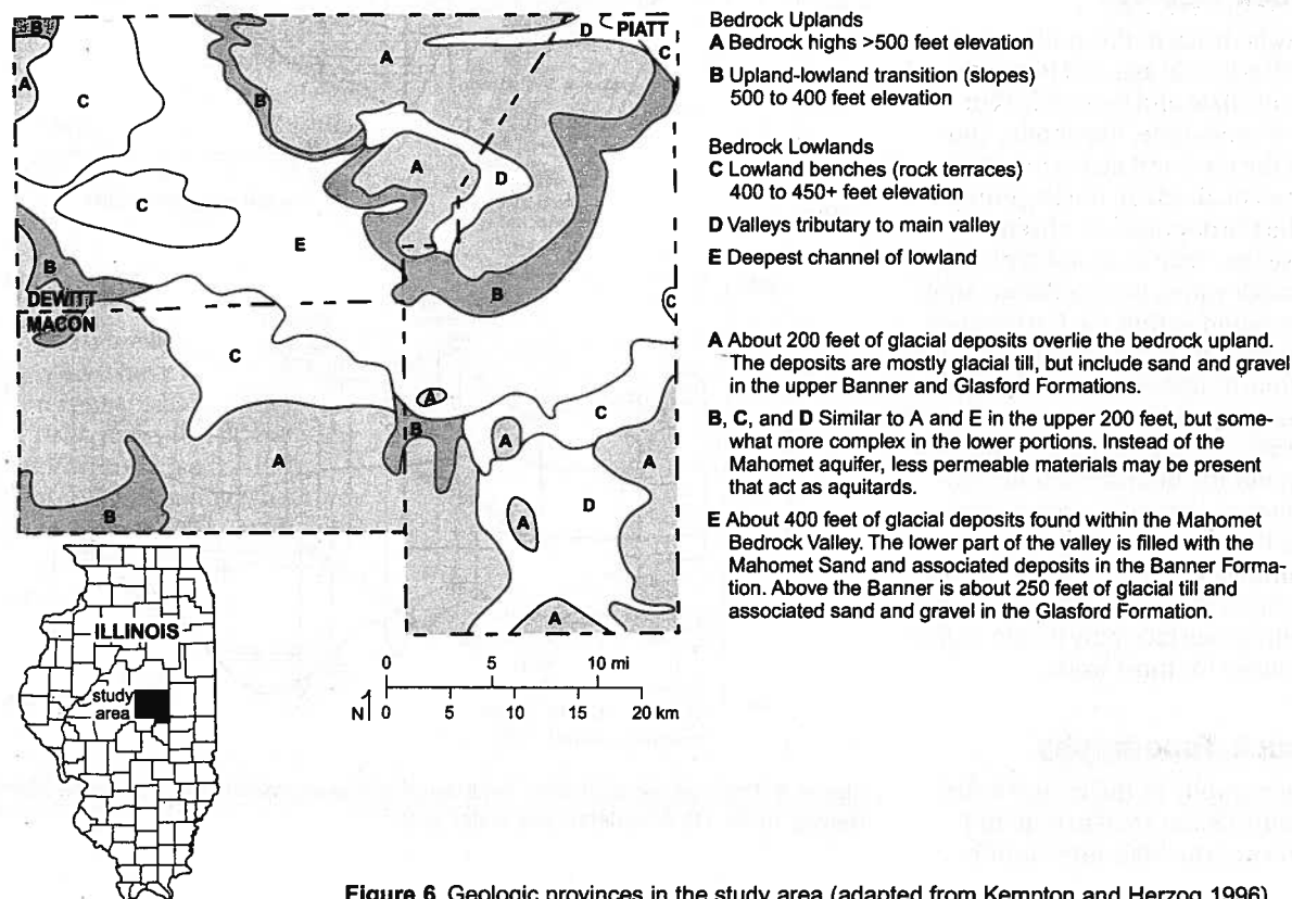
Figure 6 Geologic provinces in the study area (adapted from Kempton and Herzog 1996).
