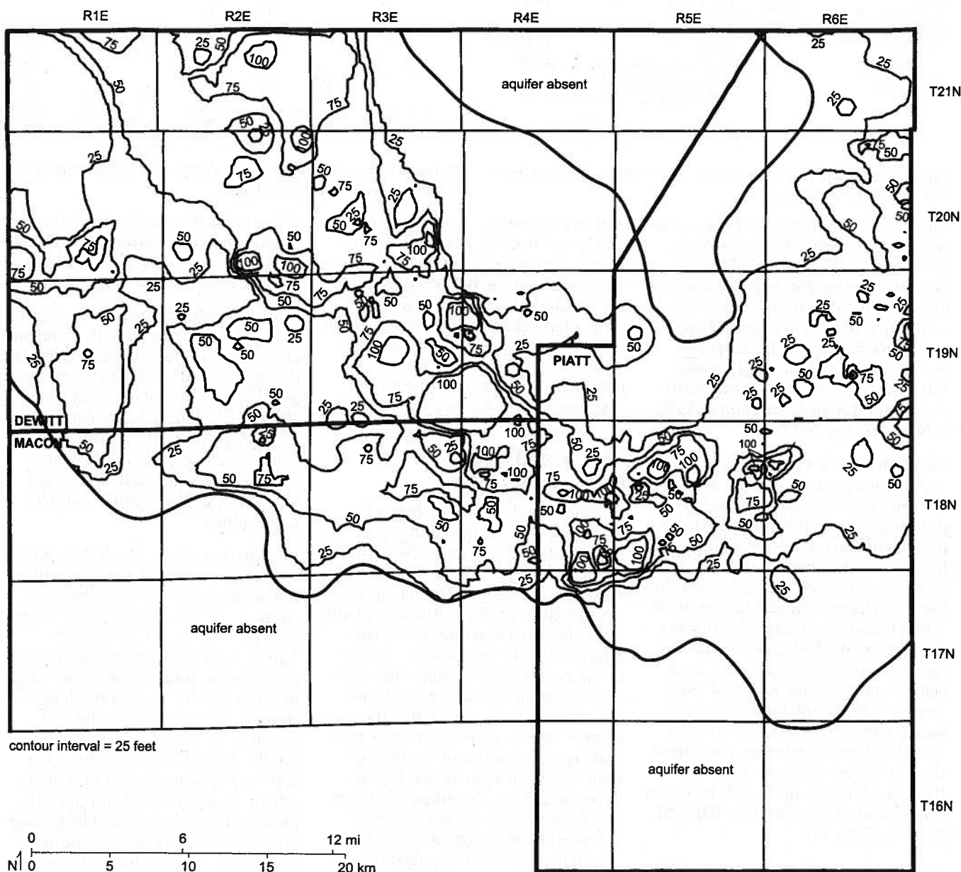
Figure 22 Thickness of the Mahomet aquifer.
