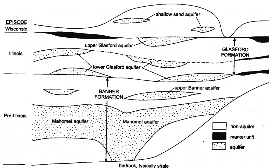
Figure 11 Classification of hydrogeologic units in the study area (modified from Herzog et al. 1995).
