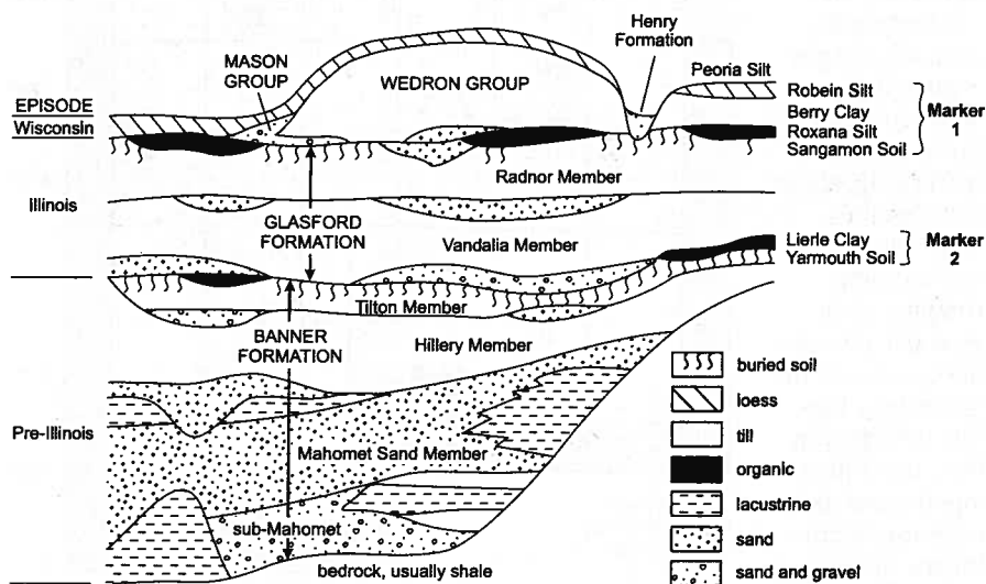
Figure 9 Schematic drawing showing stratigraphic position of Quaternary geologic materials in the study area (Herzog et al. 1995).
