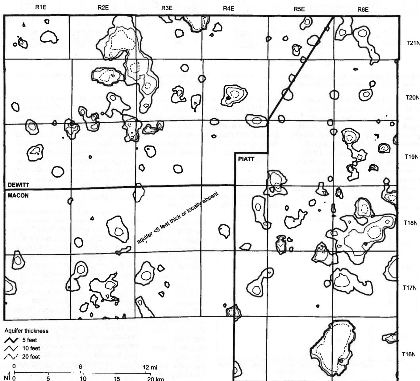
Figure 45 Thickness of the shallow sand aquifer.
