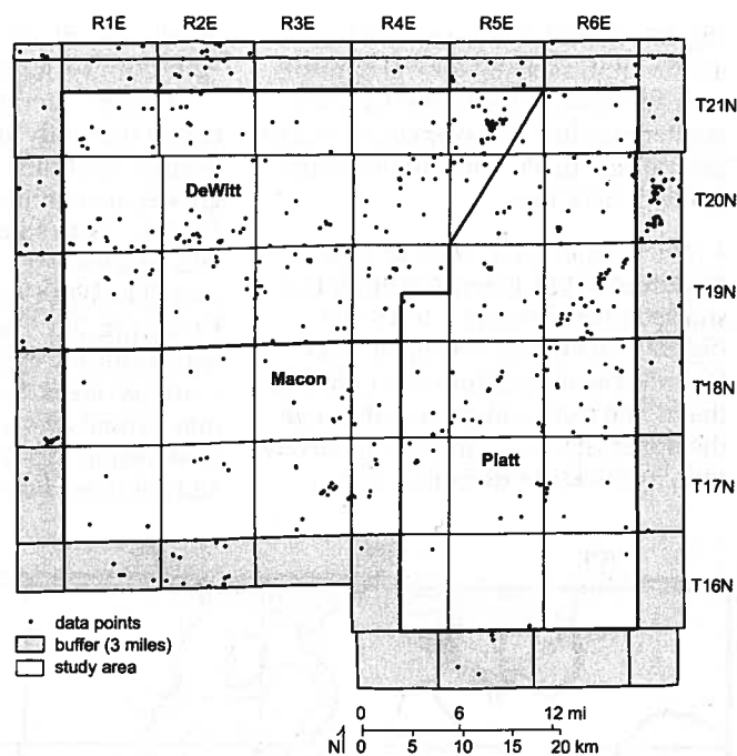
Figure 24 Distribution of data points used in determining the thickness of the upper Banner aquifer.
