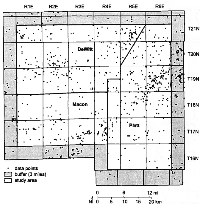
Figure 29 Distribution of data points used in determining the elevation and depth to the top of the lower Glasford aquifer.
