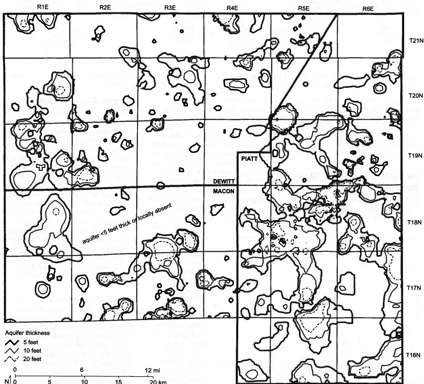
Figure 38 Thickness of the upper Glasford aquifer.
