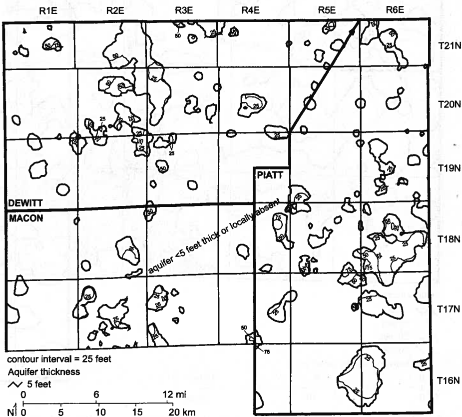
Figure 47 Depth to the top of the shallow sand aquifer.
