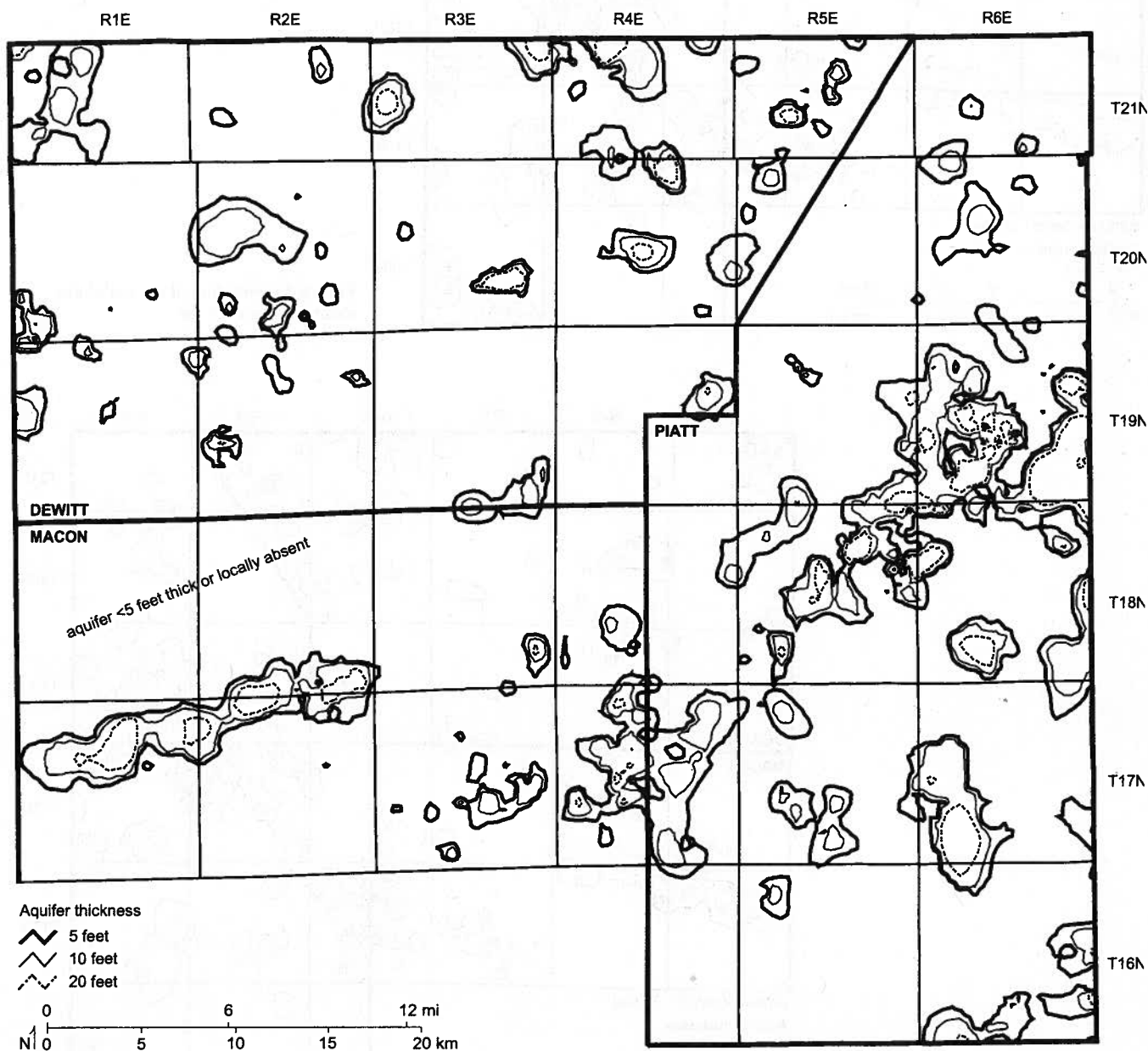
Figure 32 Thickness of the lower Glasford aquifer.
