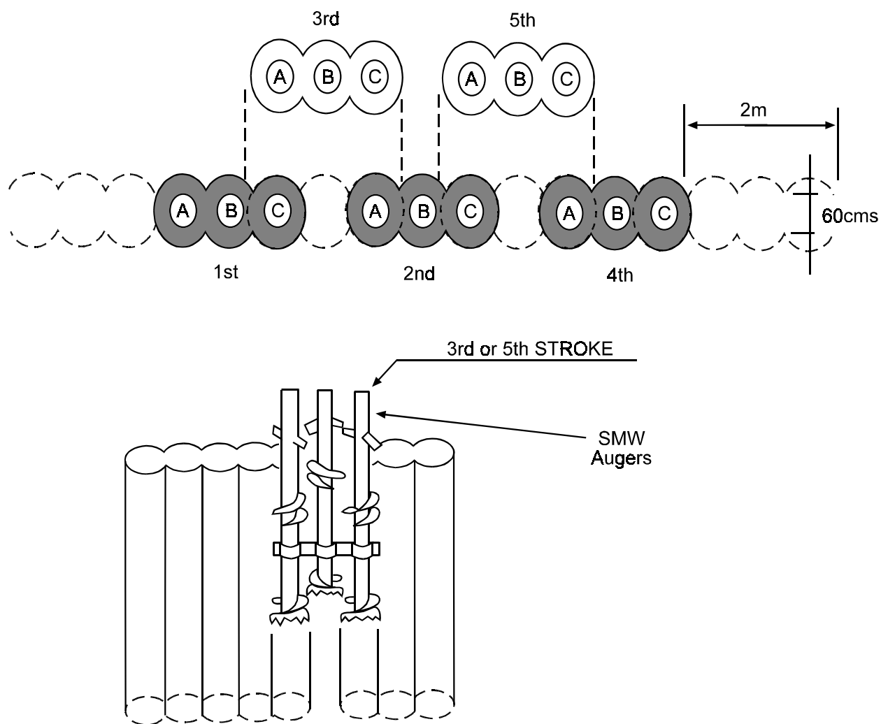
Figure A-8 Installation Sequence for a Deep Soil Mixed Barrier
