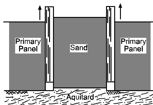
Figure 5(b) Stop ends lifted
