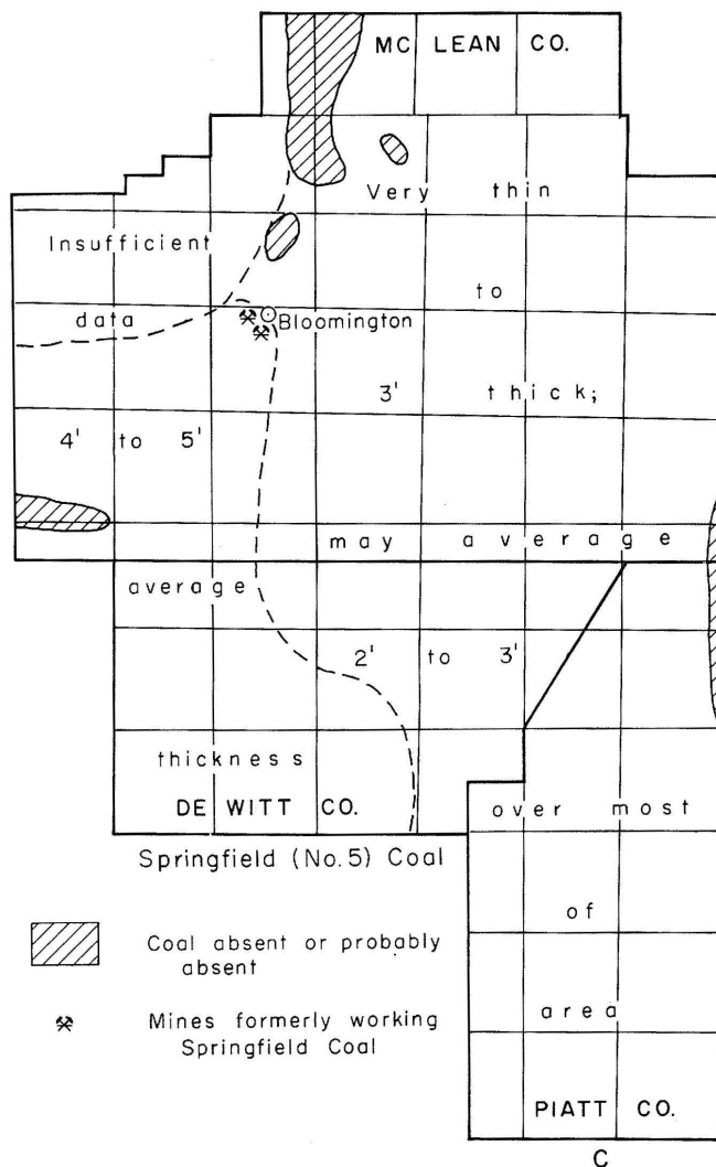
Fig. 7 - Distribution and estimated thicknesses of coals that appear to have the most likely potential as minable reserves in De Witt, McLean, and Piatt Counties.
