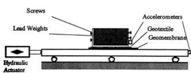
Figure 31: Test apparatus for dynamic shear properties (16)
