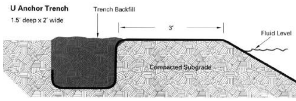
Figure 46: Anchor trench (13)
