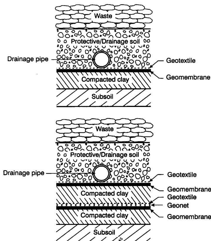
Figure 22: Cross section of single composite and double composite liners (9)
