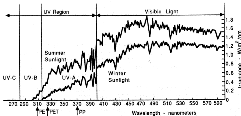
Figure 37: Wavelength Spectrum of UV radiation (12)
