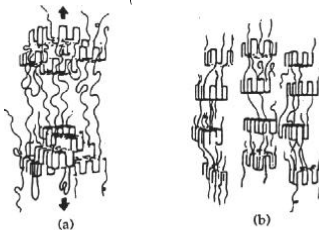
(a) Initial steps in the deformation of polyethylene
