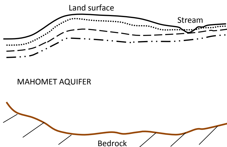
Figure 8. Simplified diagram of groundwater elevations in the unconfined Mahomet Aquifer in the Havana Lowlands. The zone between the land surface and the water table is unsaturated. The top dashed line (.....) represents the water table – the highest groundwater elevation and the top of the saturated zone. All the material between the water table and bedrock is saturated. In a drought period, groundwater elevation drops (— —). Large groundwater withdrawals for irrigation cause groundwater elevation to decline further (— · · ·). Lowering of groundwater elevation caused by drought and pumping can cause some headwater streams to go dry and reduce flow in larger streams.
