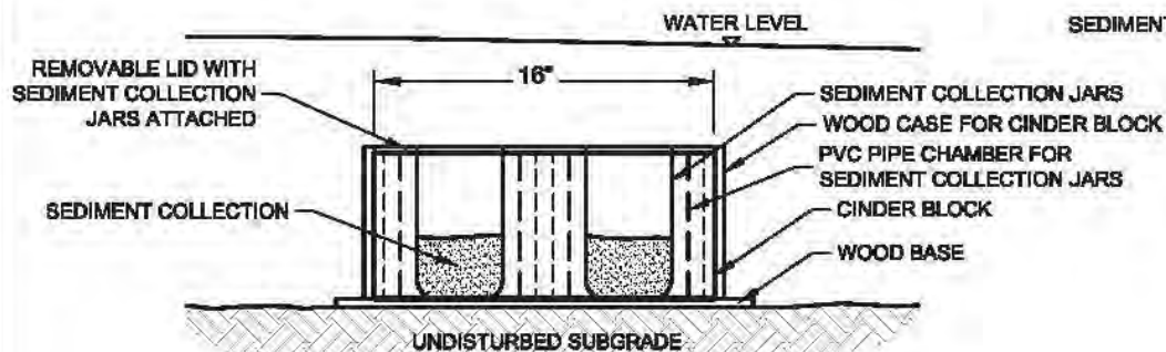
VIEW LOOKING DOWNSTREAM
