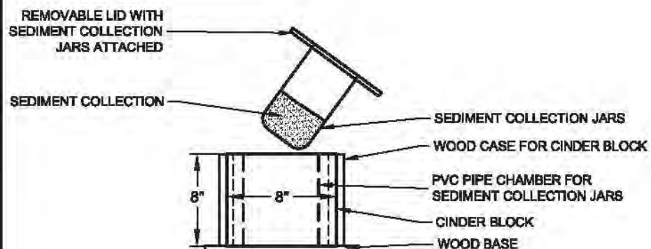
SEDIMENT MONITORING DETAIL
