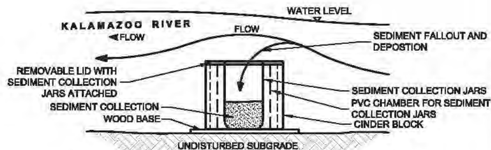
VIEW LOOKING PERPENDICULAR TO STREAM FLOW
