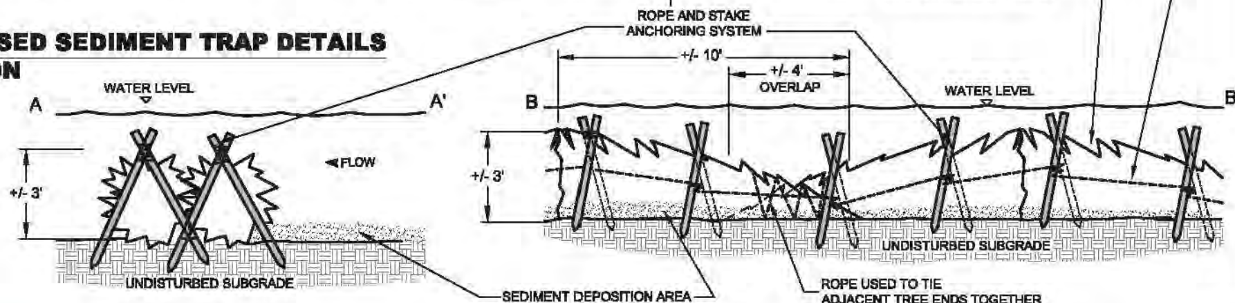
FIGURE 1 SEDIMENT TRAP DETAILS PLAN AND SECTION - TYPICAL ENBRIDGE LINE 6B MP 608 MARSHALL, MI PIPELINE RELEASE ENBRIDGE ENERGY, LIMITED PARTNERSHI P
