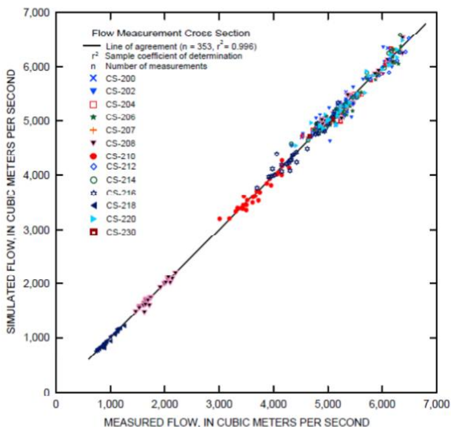
Figure 4.3.4 -- Relation between simulated flow and flow measured on the St. Clair River from 1996 to 2007 (from Holtschlag and Hoard, 2009)
