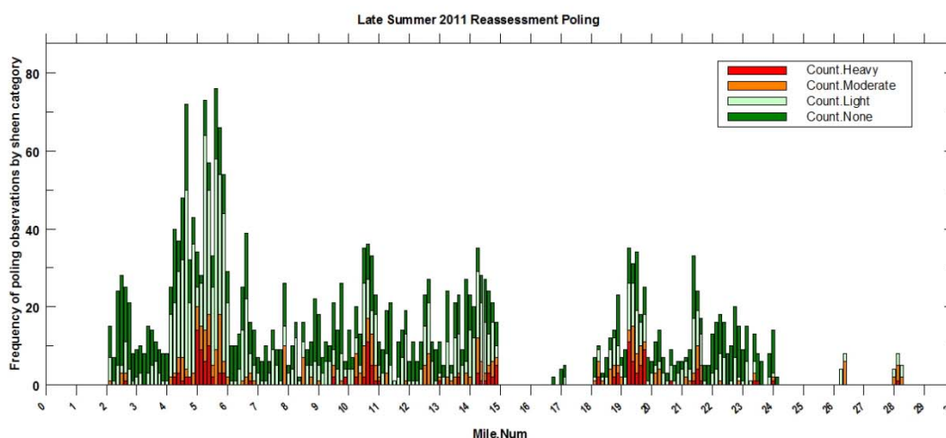
Figure 7.1. Results from the 2011 LSR poling, showing frequency of occurrence of none, light, moderate, and heavy oil indications.
