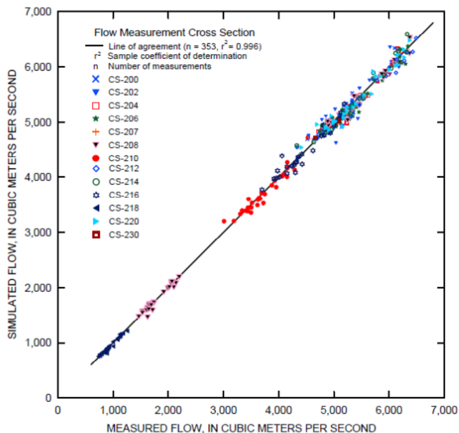
Figure 4.3.4 -- Relation between simulated flow and flow measured on the St. Clair River from 1996 to 2007 (from Holschlag and Hoard, 2009)
