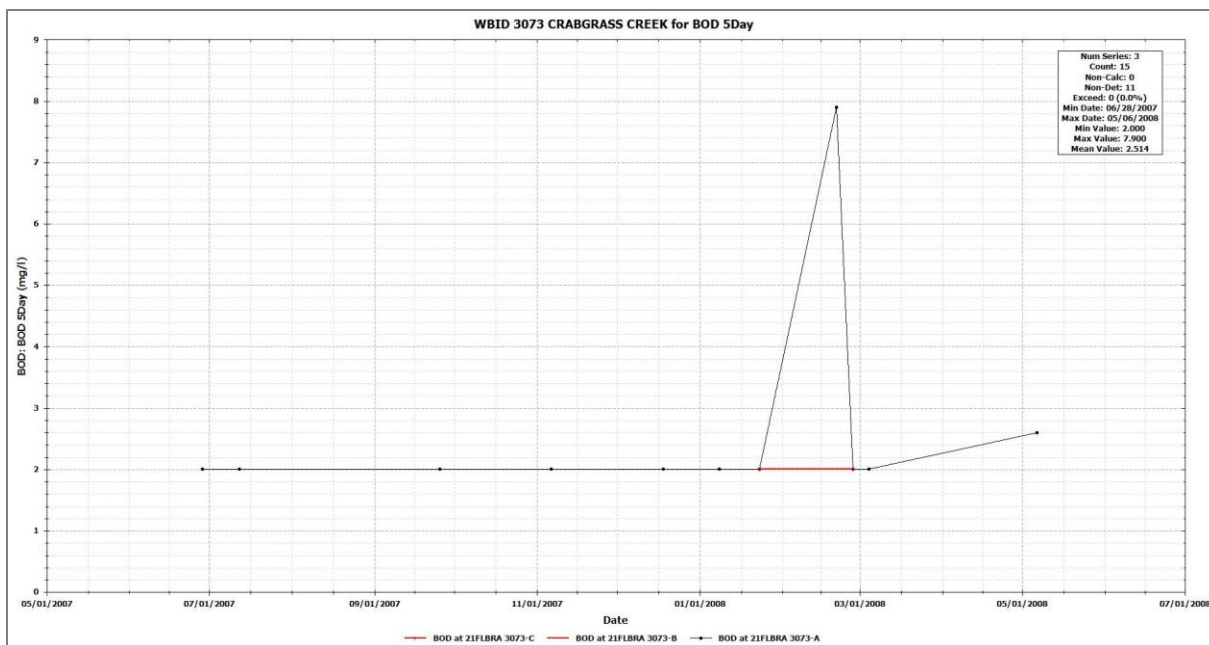
Figure 9. WBID: 3073 Crabgrass Creek Measured BOD
