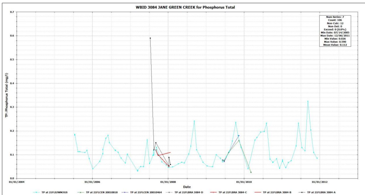
Figure 17. WBID: 3084 Jane Green Creek Measured Total Phosphorus
