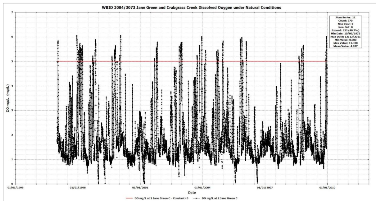
Figure 20. DO Concentration Time Series under Natural Condition
