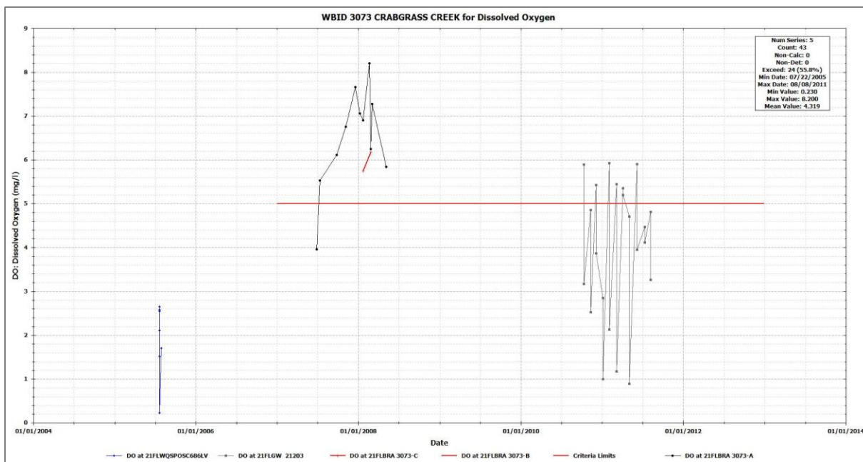
Figure 8. WBID: 3073 Crabgrass Creek Measured DO
