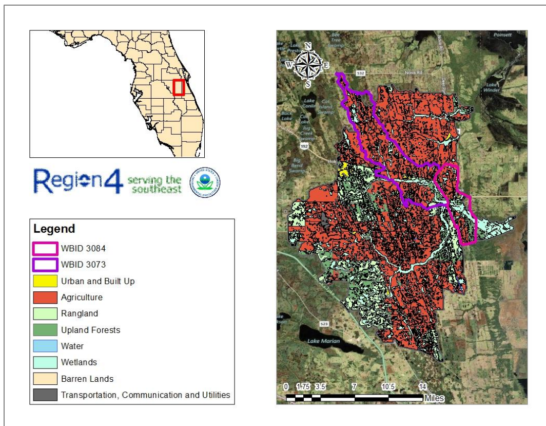
Figure 3. Landuse in the Crabgrass Creek and Jane Green Creek Watershed
