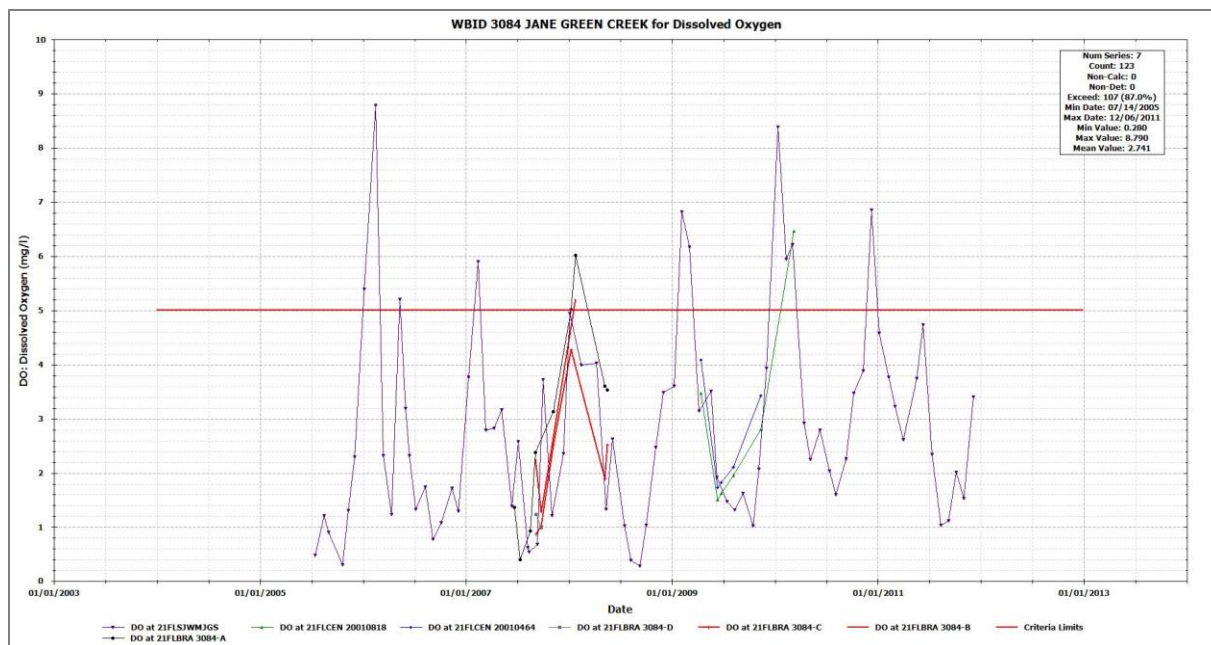
Figure 14. WBID: 3084 Jane Green Creek Measured DO
