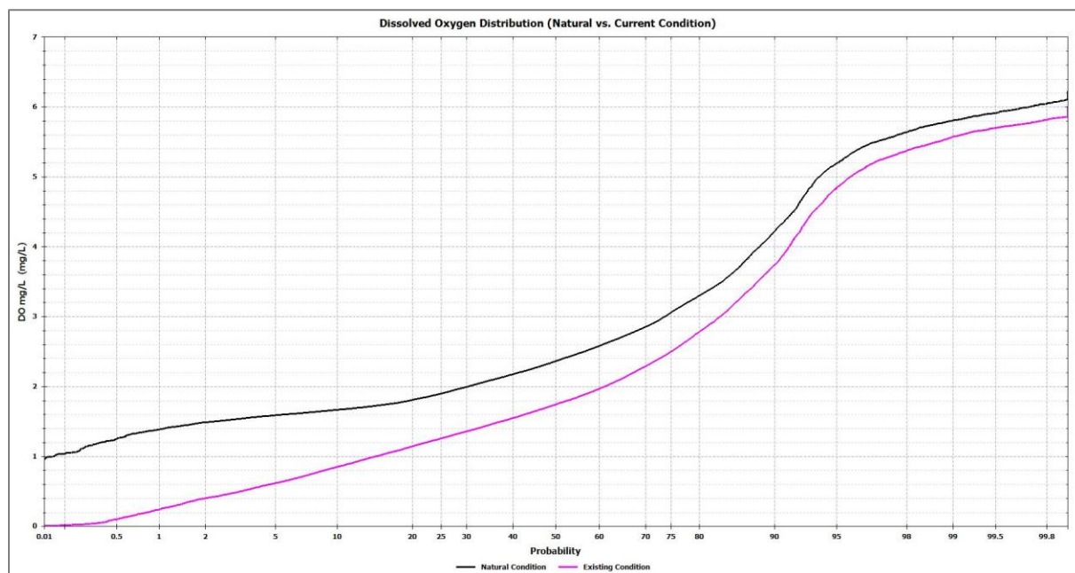
Figure 21. DO Concentration Cumulative Distribution Function Natural vs. Current Condition
