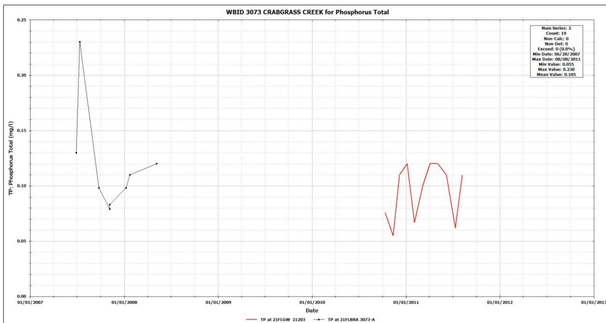
Figure 11. WBID: 3073 Crabgrass Creek Measured Total Phosphorus
