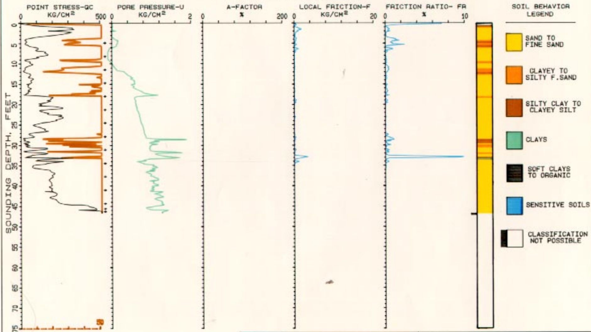
FIGURE 3-4 ECPT SOUNDING LOG, LOCATION PZ1 BRUNSWICK WOOD PRESERVING SUPERFUND SITE BRUNSWICK, GEORGIA
