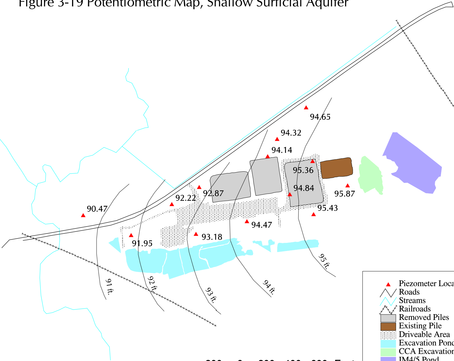
Brunswick Wood Preserving Superfund Site Figure 3-19 Potentiometric Map, Shallow Surficial Aquifer
