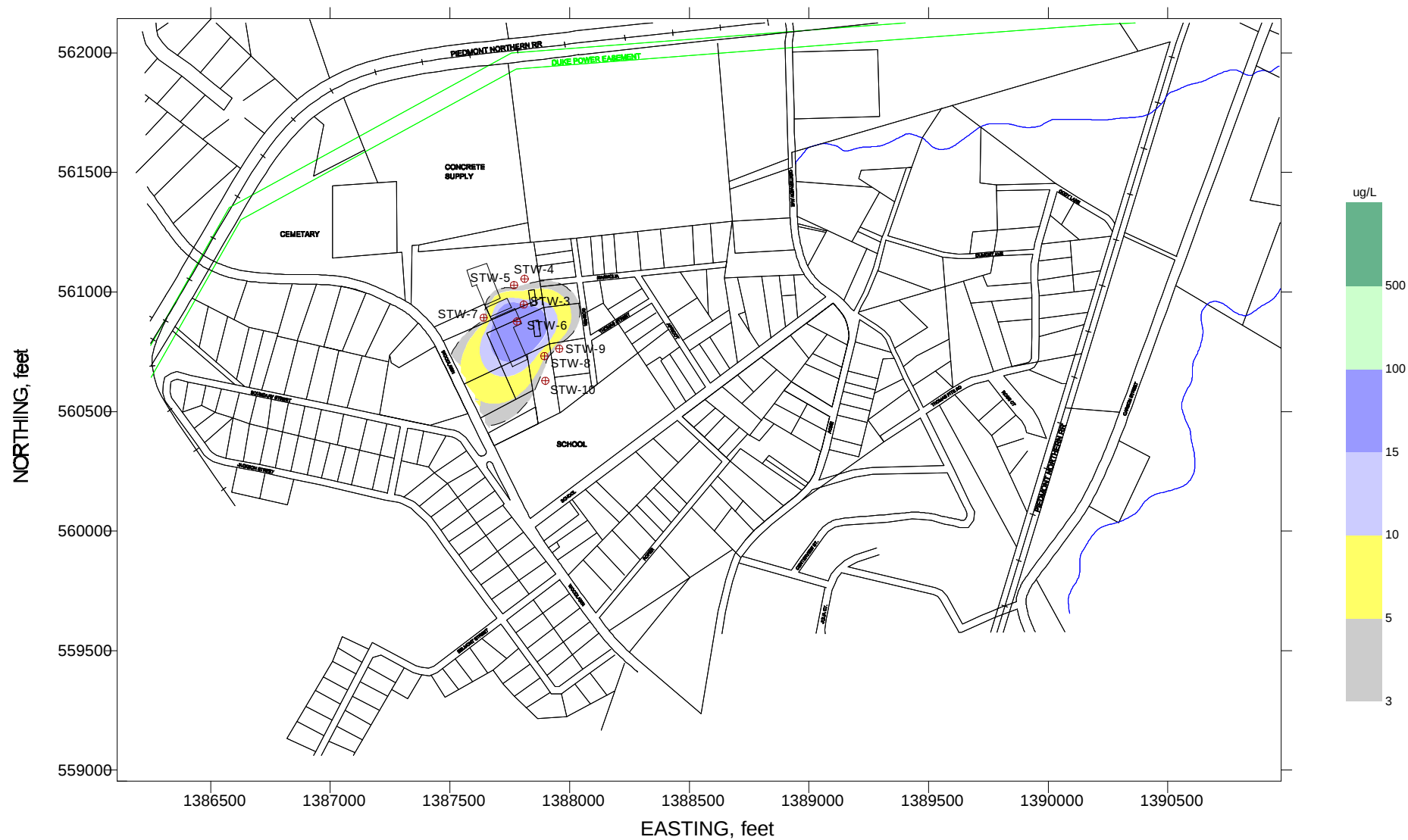
FIGURE 4-6 SHALLOW GROUNDWATER PLUME, TCE CONTAMINATION, JUNE 1996 REMEDIAL INVESTIGATION REPORT NORTH BELMONT PCE SUPERFUND SITE NORTH BELMONT, GASTON COUNTY, NC SEDS PROJECT No. 96S-058, JUNE 1997
