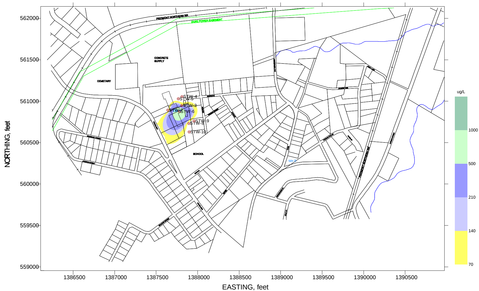
FIGURE 4-7 SHALLOW GROUNDWATER PLUME, DCE CONTAMINATION, JUNE 1996 REMEDIAL INVESTIGATION REPORT NORTH BELMONT PCE SUPERFUND SITE NORTH BELMONT, GASTON COUNTY, NC SEDS PROJECT No. 96S-058, JUNE 1997
