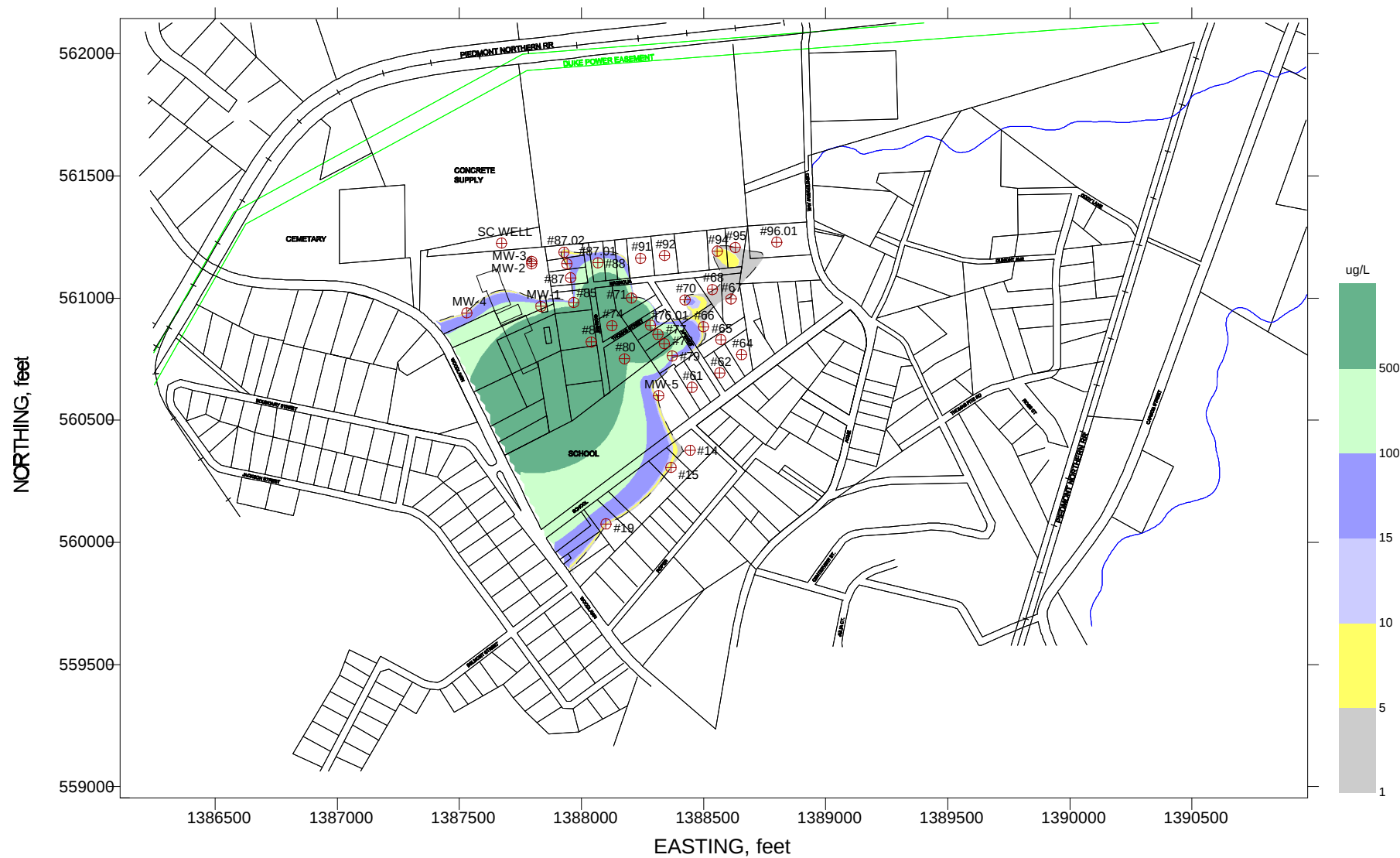
FIGURE 4-1 PCE GROUNDWATER CONTAMINATION, 1991 REMEDIAL INVESTIGATION REPORT NORTH BELMONT PCE SUPERFUND SITE NORTH BELMONT, GASTON COUNTY, NC SESD PROJECT No. 96S-058, JUNE 1997
