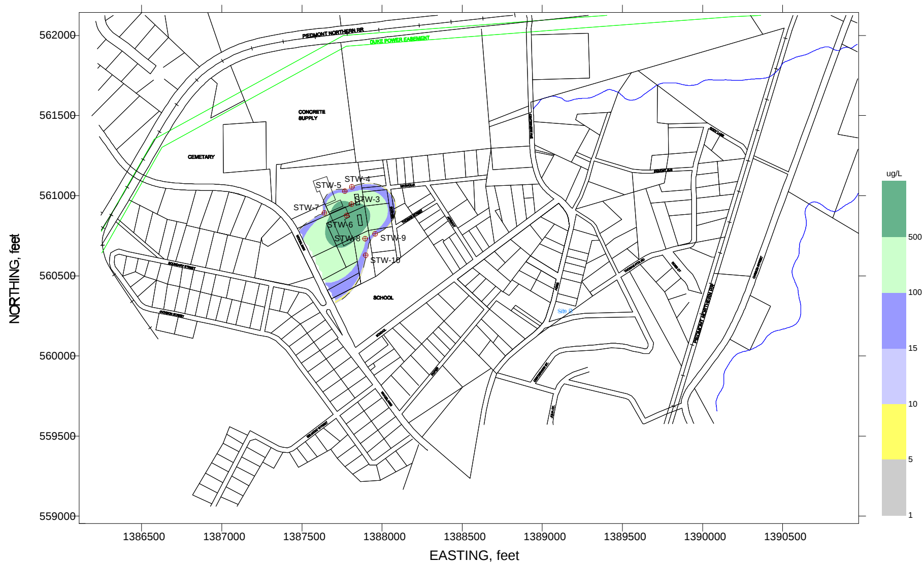
FIGURE 4-5 SHALLOW GROUNDWATER PLUME, PCE CONTAMINATION, JUNE 1996 REMEDIAL INVESTIGATION REPORT NORTH BELMONT PCE SUPERFUND SITE NORTH BELMONT, GASTON COUNTY, NC SEDS PROJECT No. 96S-058, JUNE 1997
