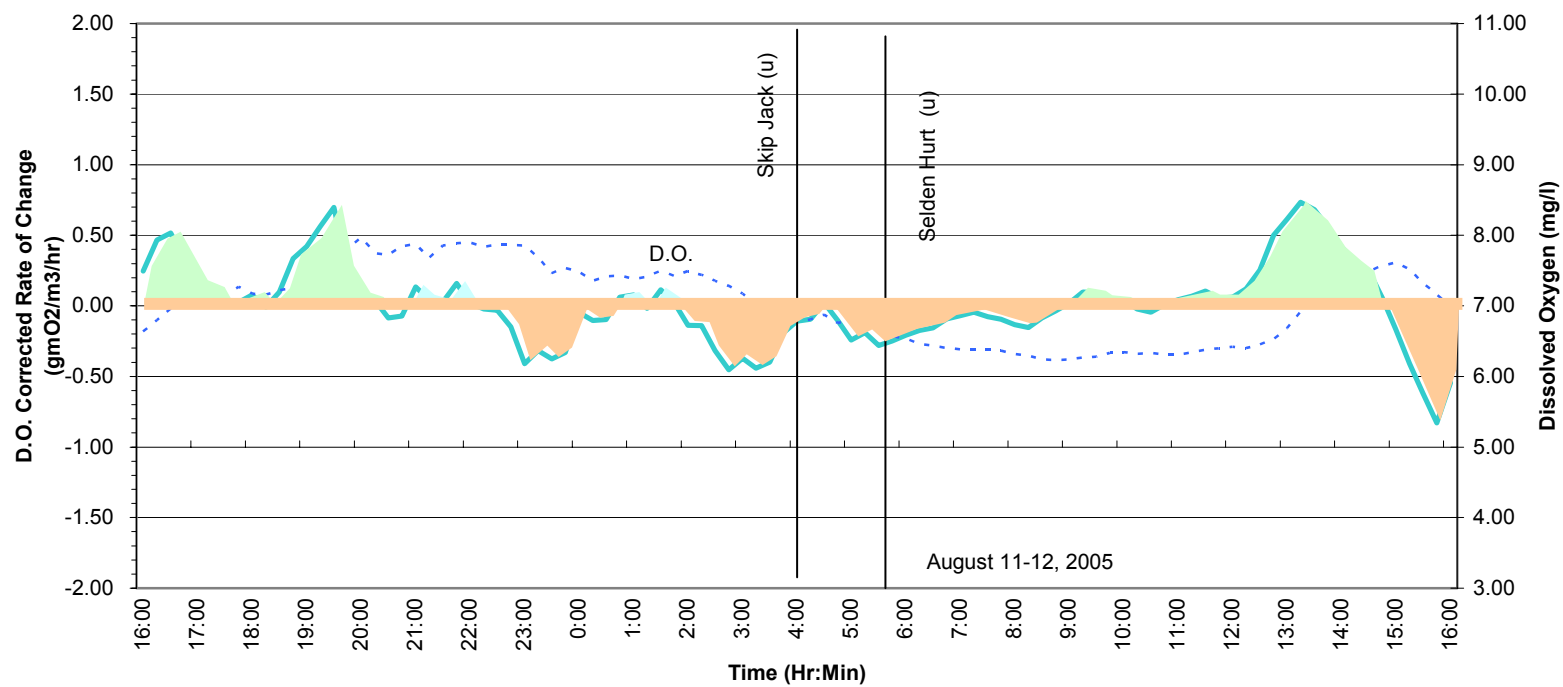
Community Metabolic Curve - TT336.3 @ 5 ft
