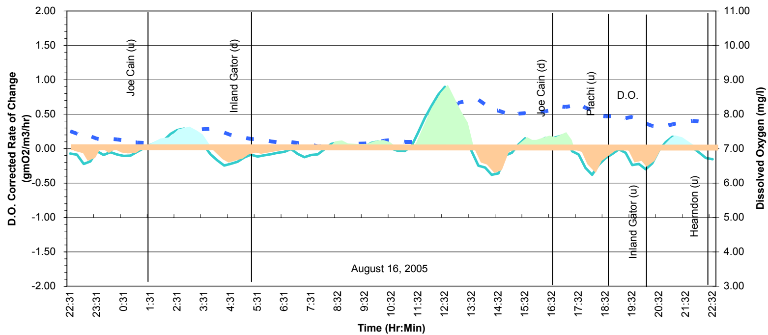
Community Metabolic Curve - TT340.0 @ 5 ft
