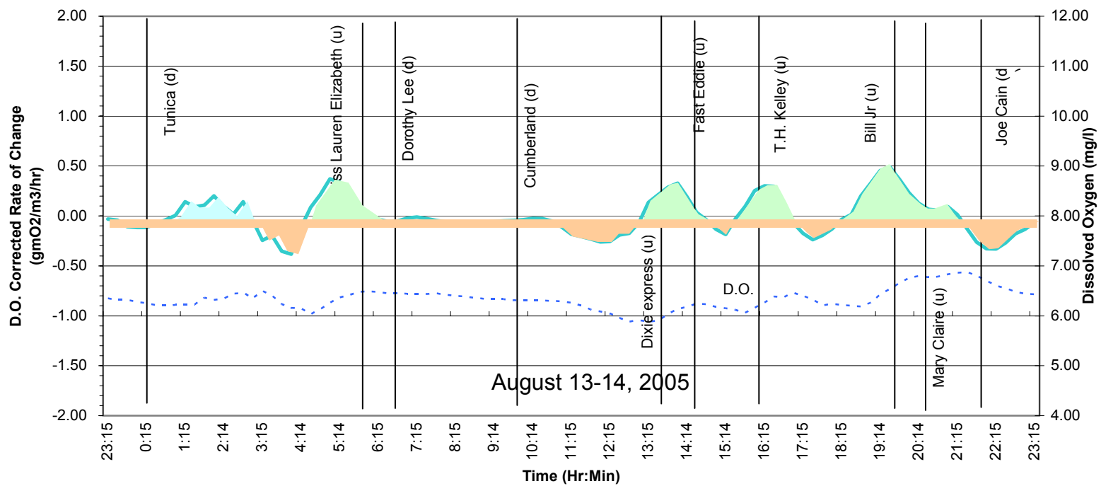
Community Metabolic Curve - TT319.6 @ 10 ft
