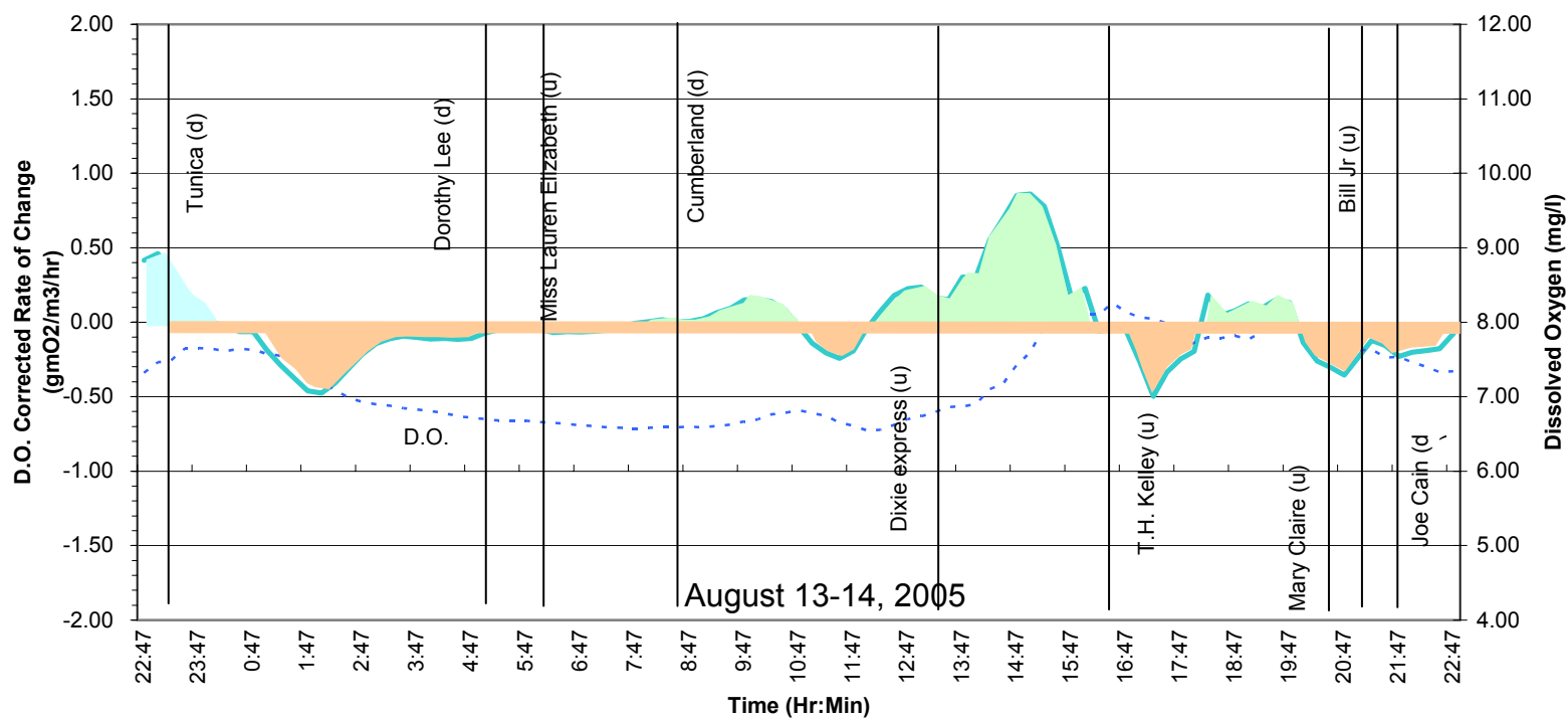
Community Metabolic Curve - TT324.4 @ 5 ft
