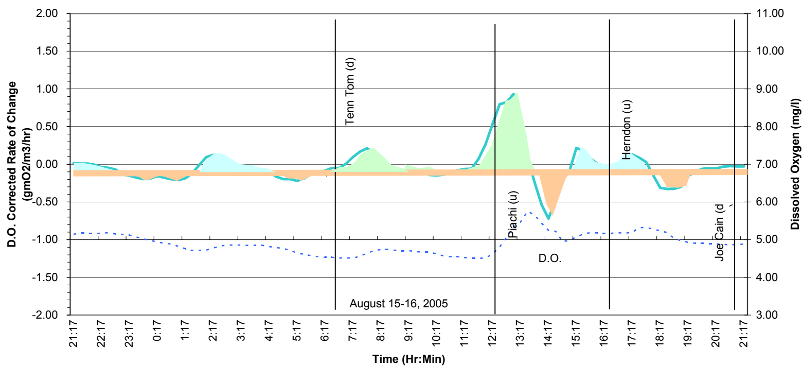
Community Metabolic Curve - TT314.7 @ 15 ft
