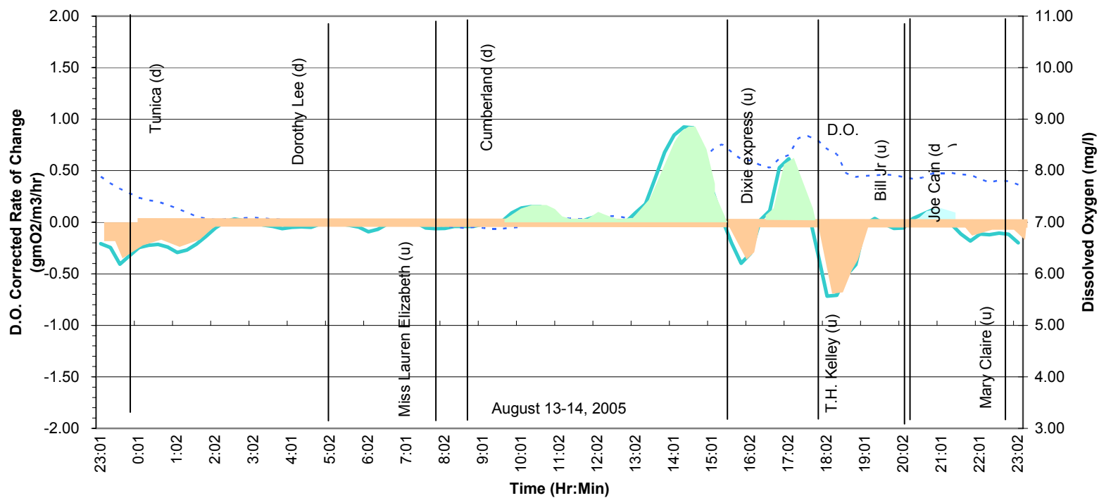
Community Metabolic Curve - TT327.7 @ 5 ft
