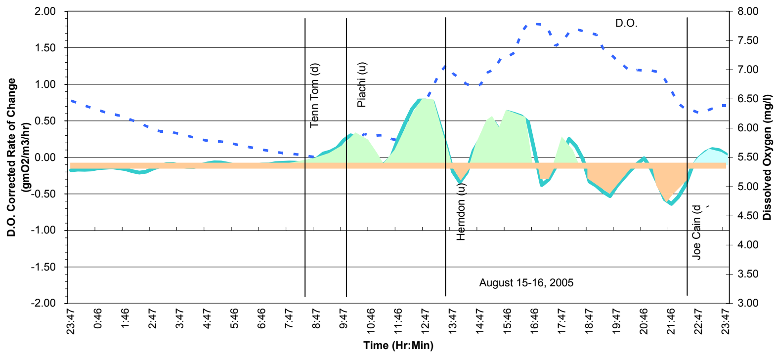
Community Metabolic Curve - TT304.5 @ 1 ft
