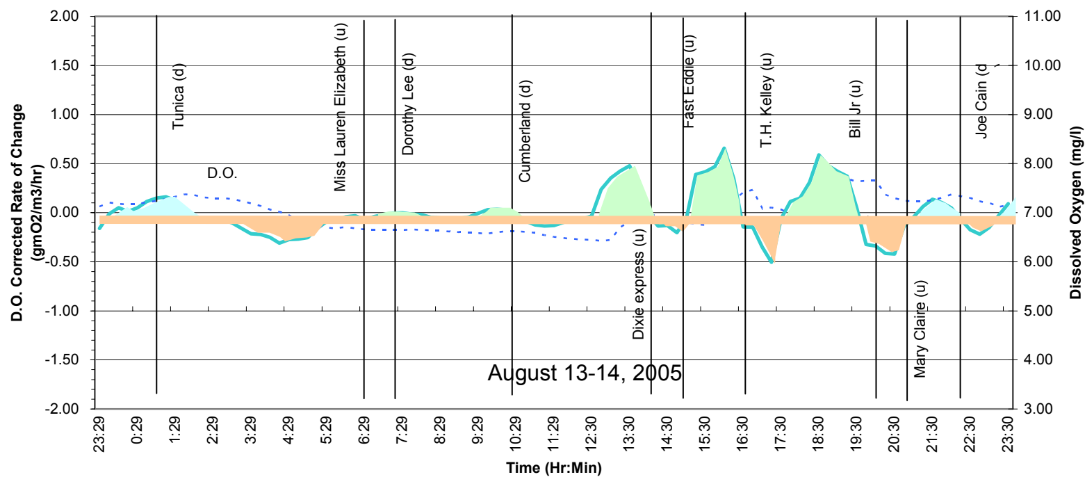
Community Metabolic Curve - TT319.6 @ 1 ft
