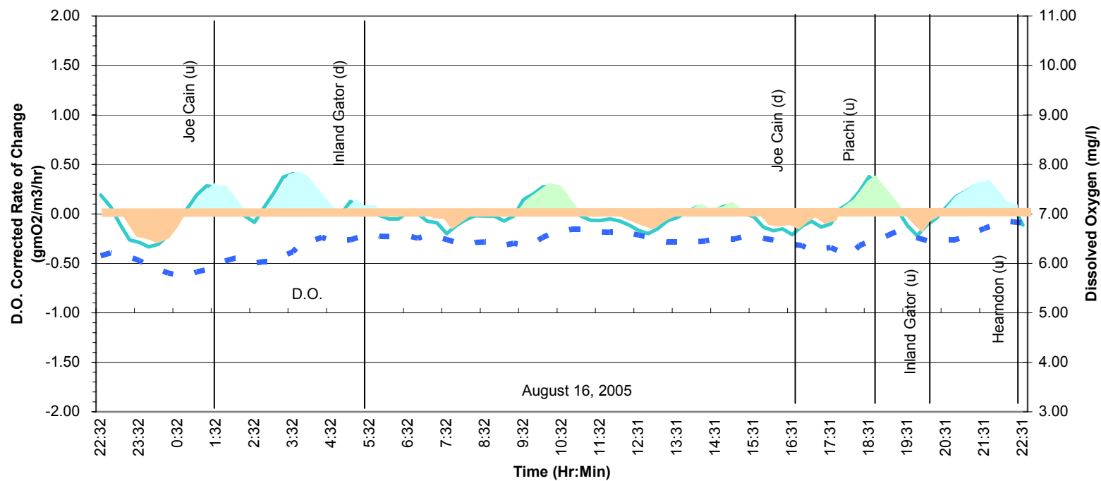
Community Metabolic Curve - TT340.0 @ 12 ft
