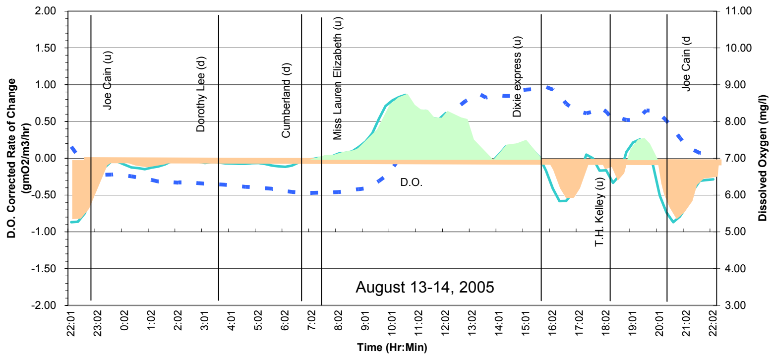
Community Metabolic Curve - TT332.4 @ 1 ft
