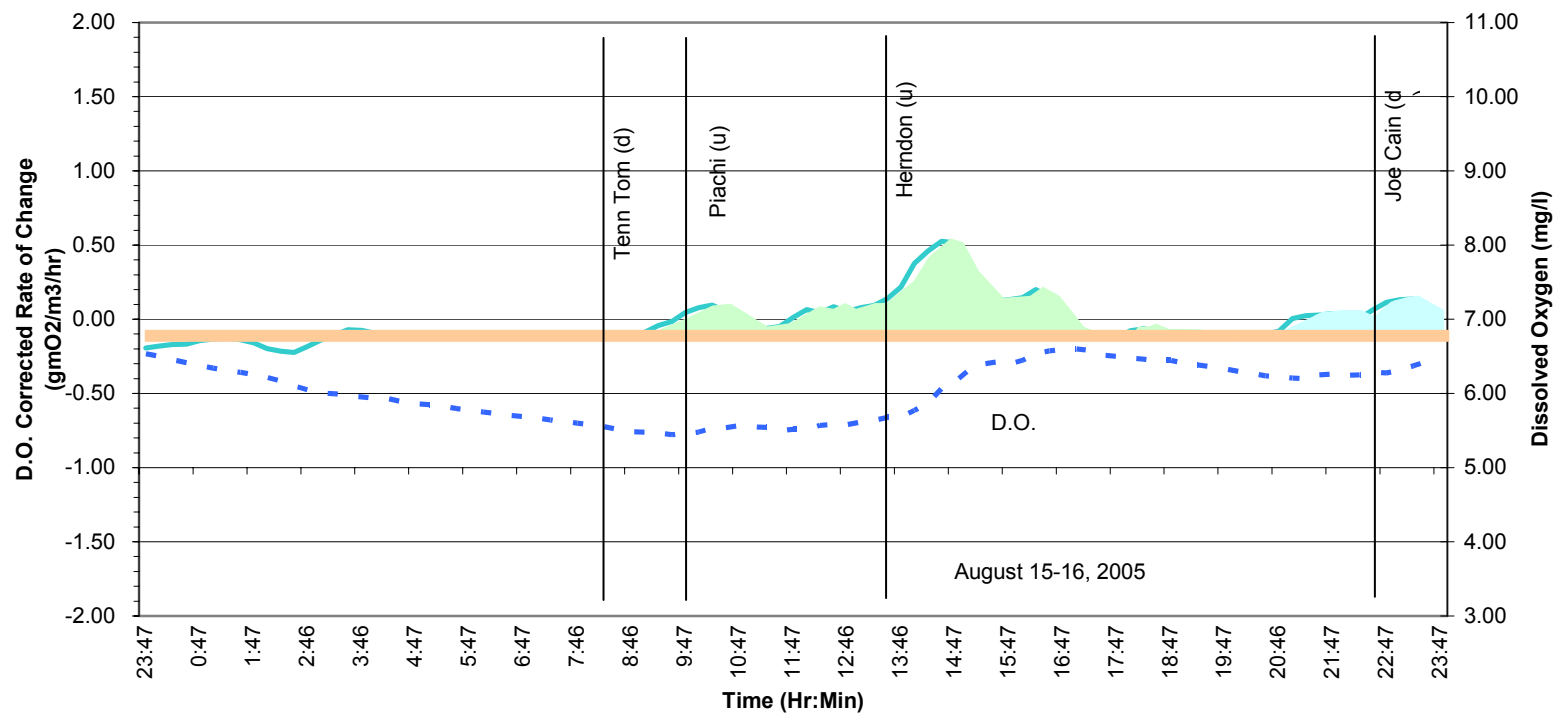
Community Metabolic Curve - TT304.5 @ 5 ft
