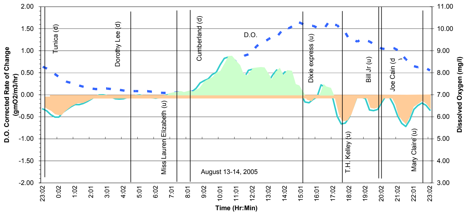
Community Metabolic Curve - TT327.7 @ 1 ft
