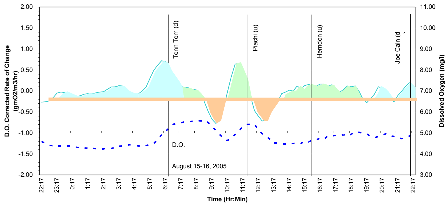
Community Metabolic Curve - TT310.0 @ 5 ft
