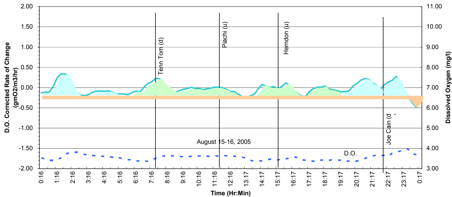
Community Metabolic Curve - TT307.3 @12.5 ft
