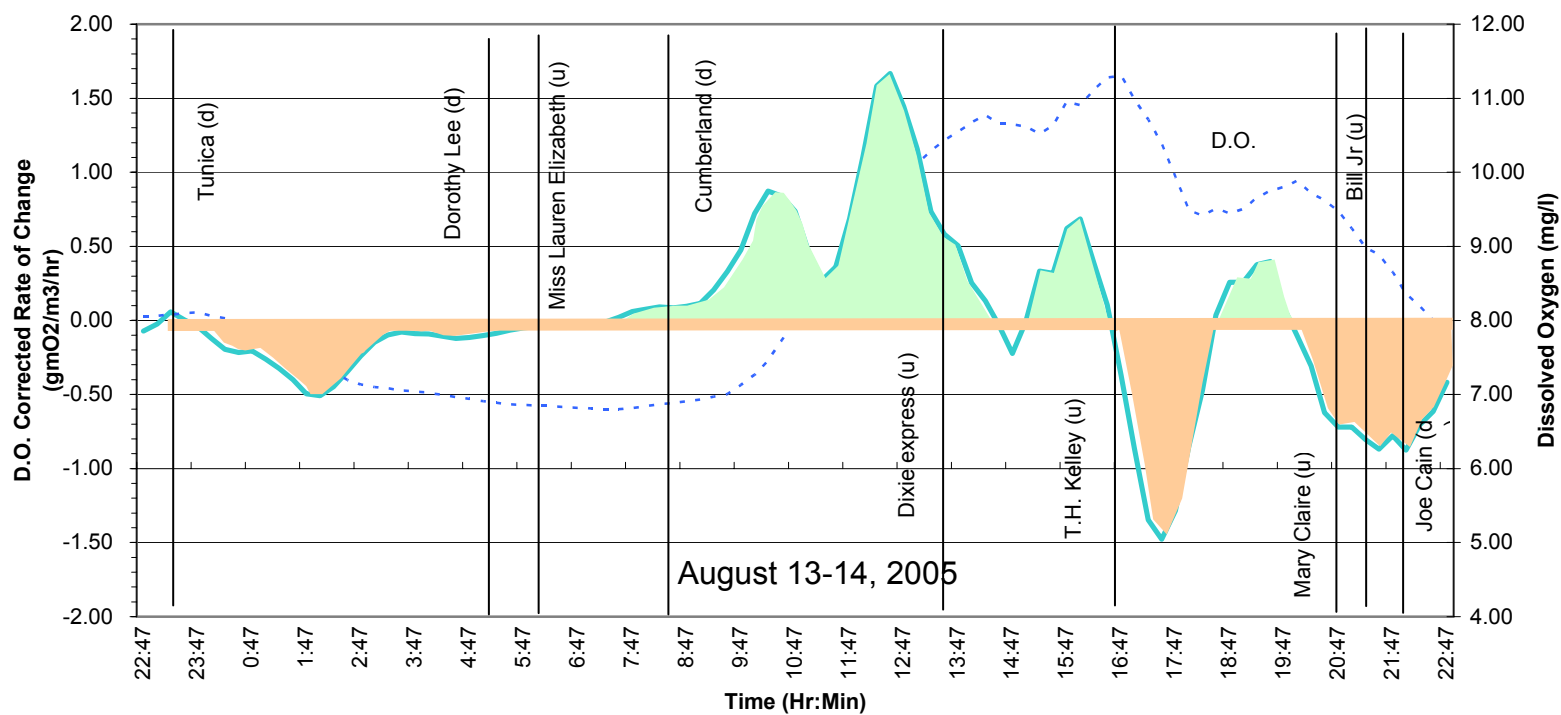
Community Metabolic Curve - TT324.4 @ 1 ft
