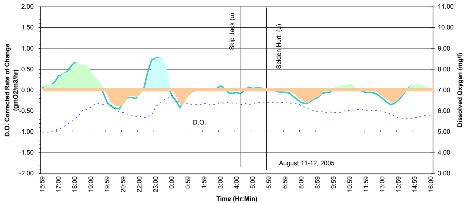
Community Metabolic Curve - TT336.3 @ 10 ft
