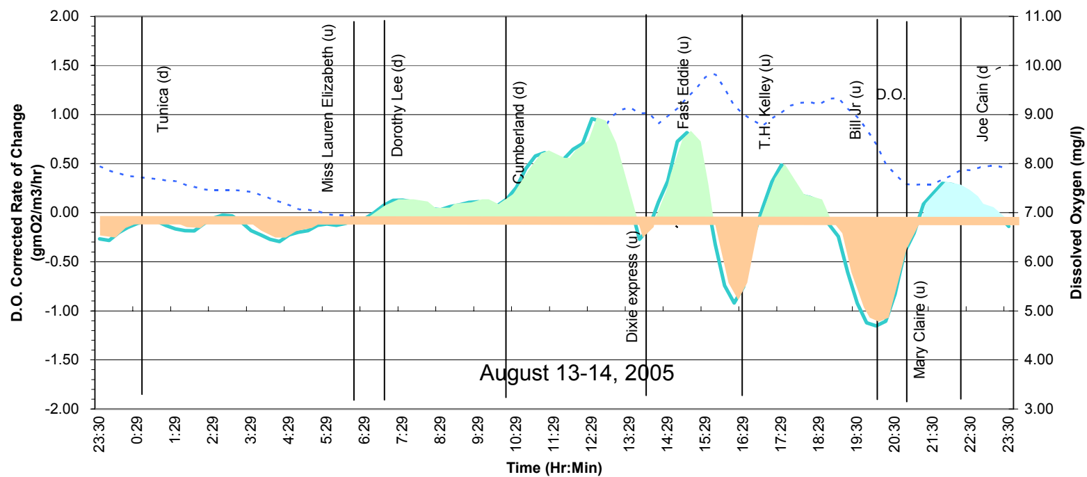
Community Metabolic Curve - TT319.6 @ 5 ft
