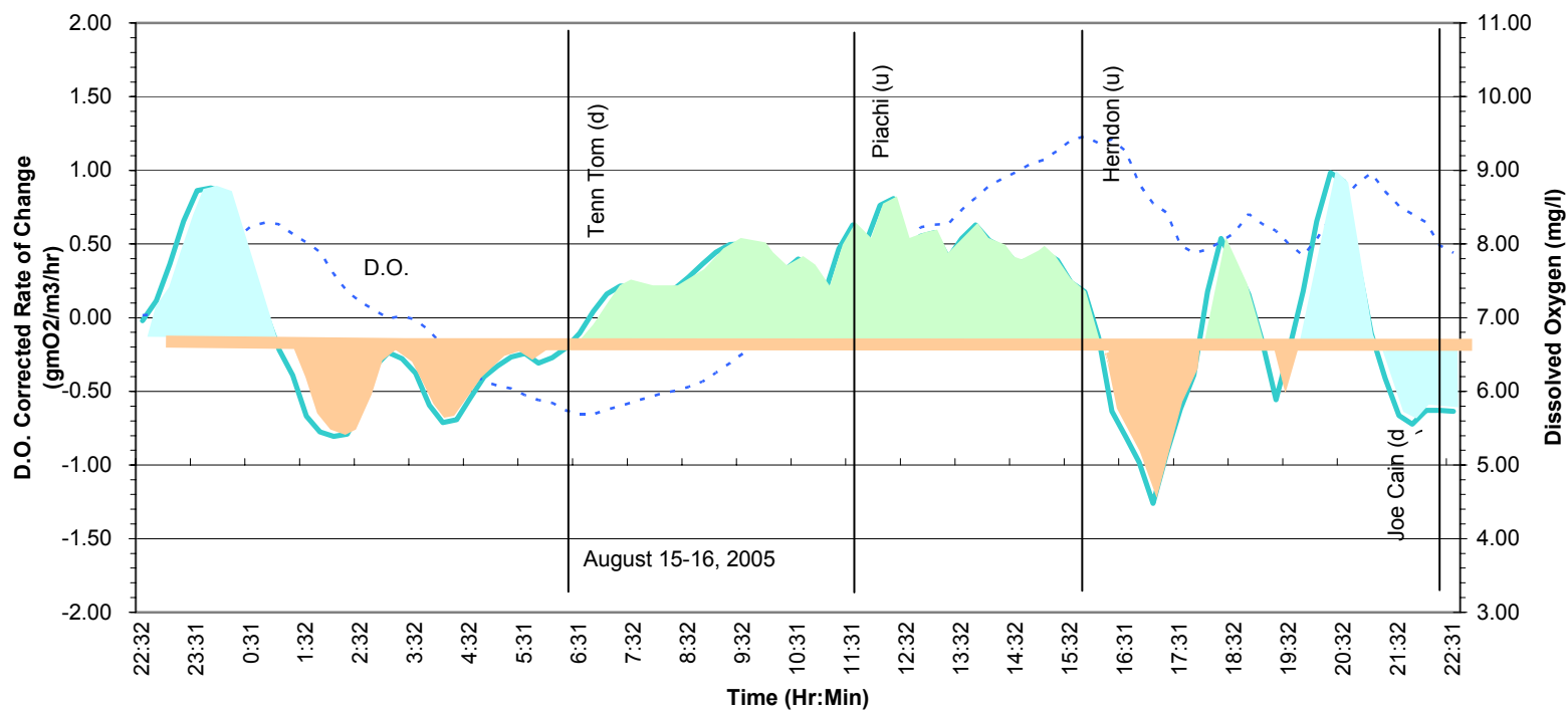
Community Metabolic Curve - TT310.0 @ 1 ft
