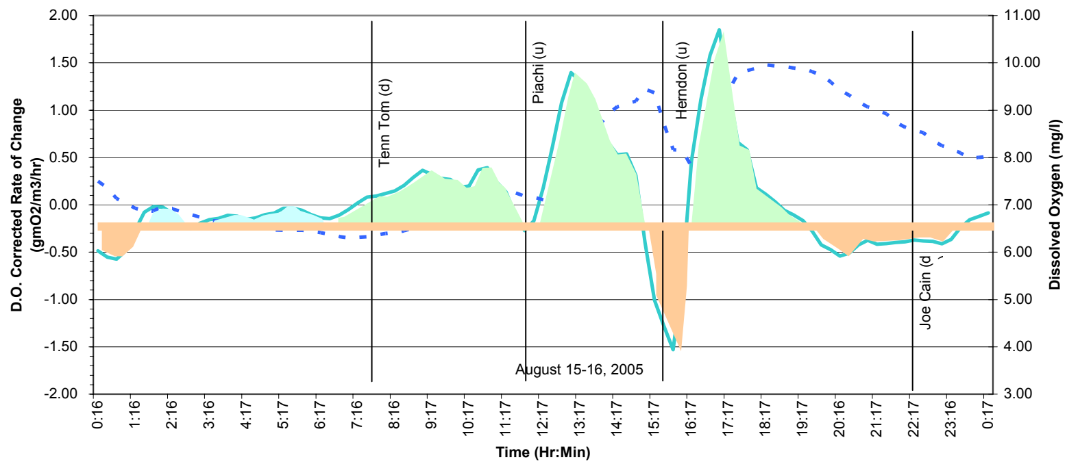
Community Metabolic Curve - TT307.3 @ 1 ft
