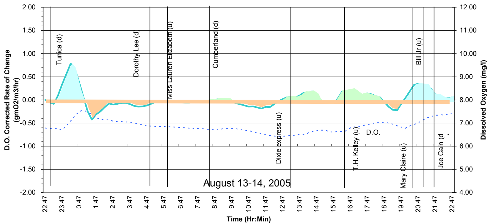
Community Metabolic Curve - TT324.4 @ 10 ft
