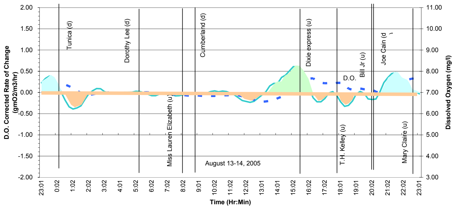
Community Metabolic Curve - TT327.7 @ 10 ft
