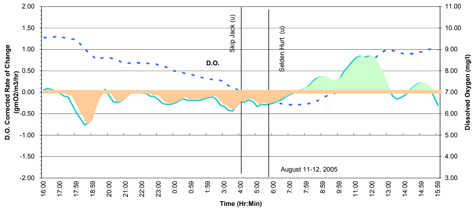
Community Metabolic Curve - TT336.3 @ 1 ft
