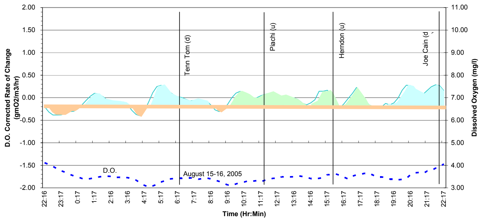
Community Metabolic Curve - TT310.0 @ 11 ft
