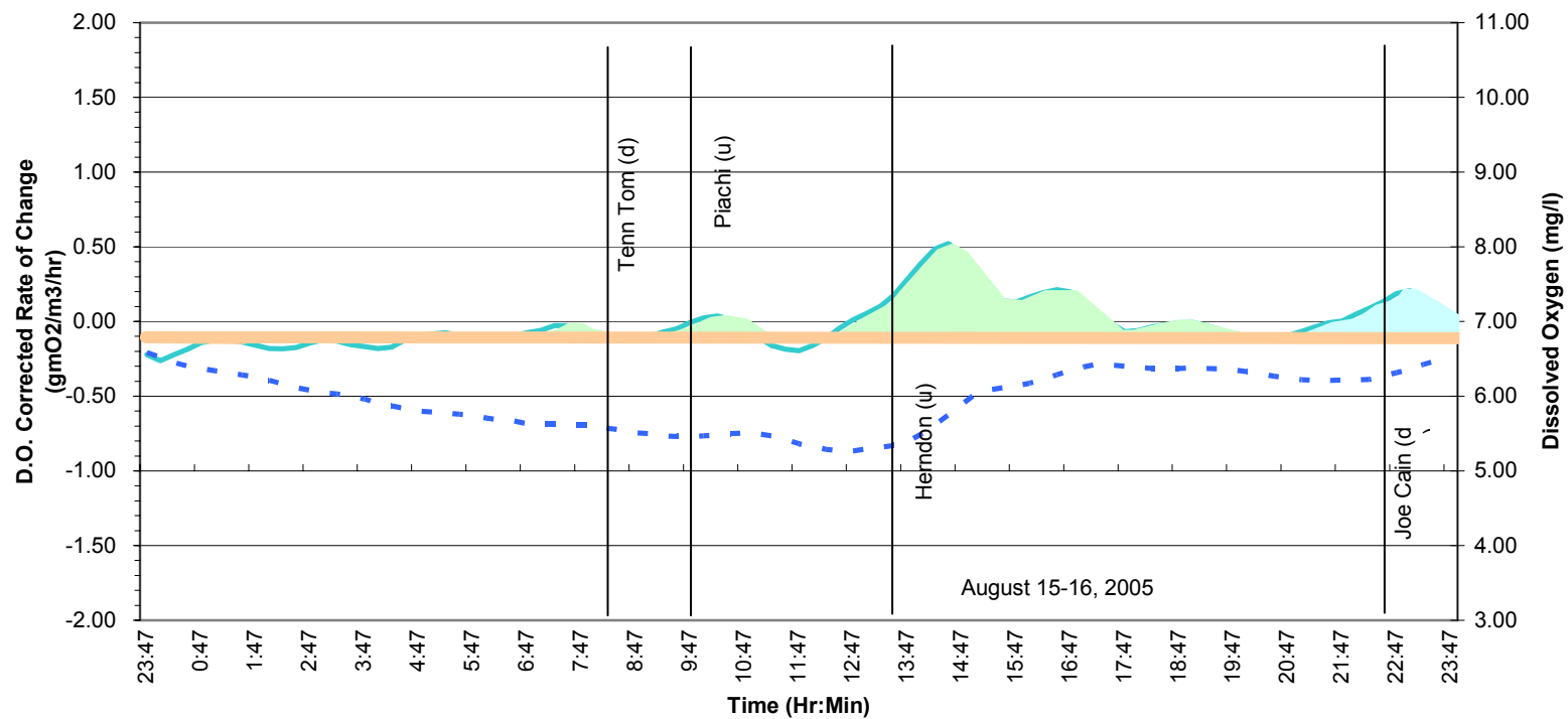
Community Metabolic Curve - TT304.5 @ 8.5 ft
