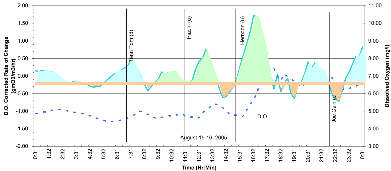
Community Metabolic Curve - TT307.3 @ 5 ft
