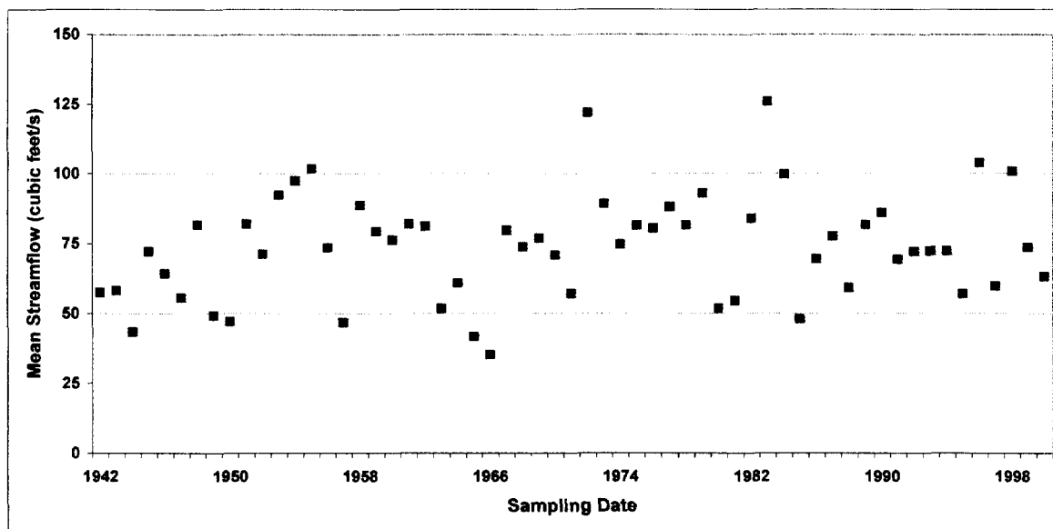
Figure 3. Annual Mean Streamflow (cfs) at the Woonasquatucket River from 1942 to 2001.
