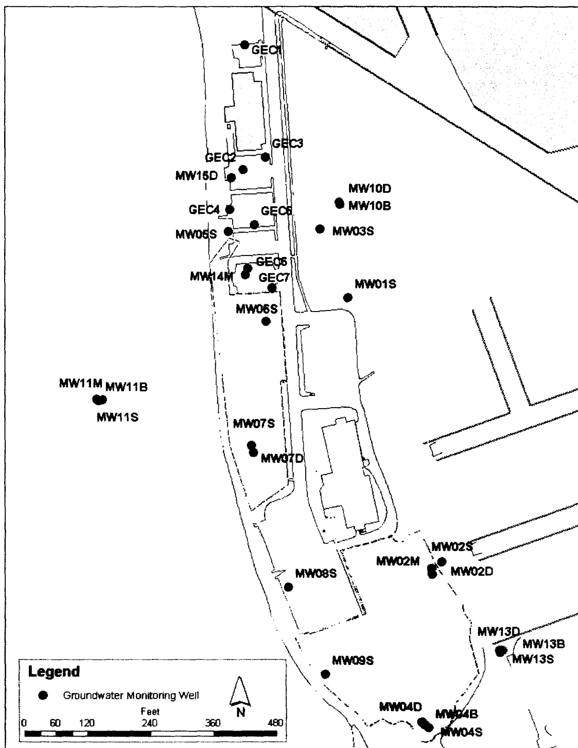
Figure 12. Monitoring Well Locations.
