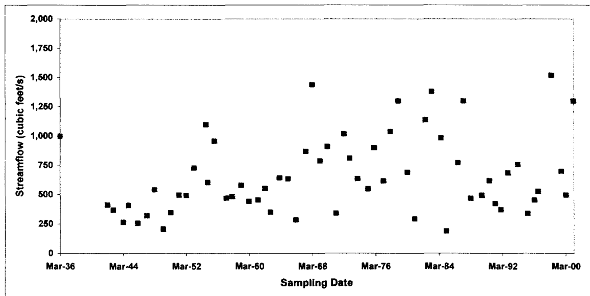
Figure 4. Peak Streamflow (cfs) at the Woonasquatucket River between 1936 and 2000.
