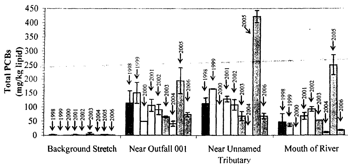
FIGURE 4-10 Lipid-normalized PCB concentration in resident spottail shiner in Grasse River, Massena, NY. Locations are from upstream (Background and Near Outfall 001) to downstream (Near Unnamed Tributary, about 2 miles downstream, and Mouth of River, about 6 miles downstream). Error bars represent \pm 2 standard errors of the mean. Dredging at the site took place June to October, 2005; the 2005 fish tissue sampling was in September, 2005. Source: L. McShea, Alcoa, unpublished data, February 27, 2007. Reprinted with permission; copyright 2007, Alcoa Incorporated.
