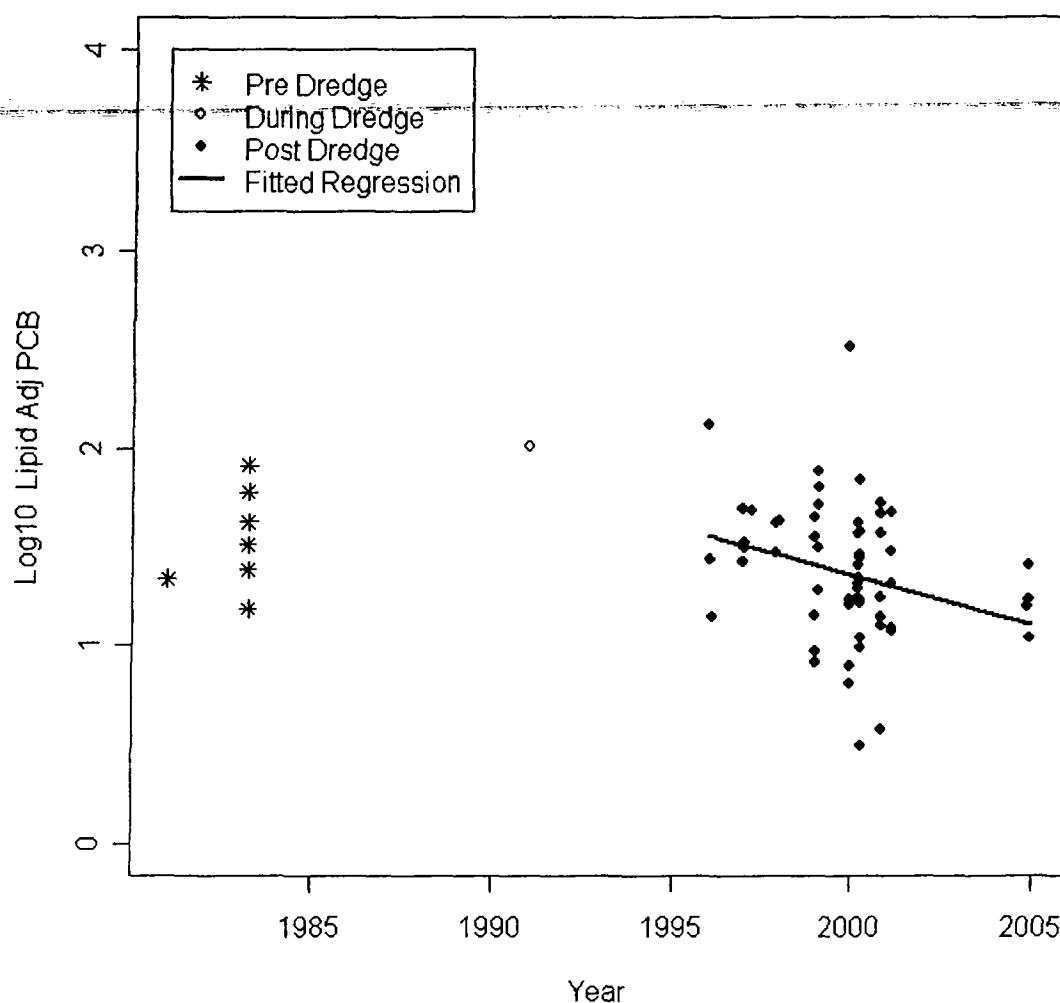
FIGURE 4-15 Lipid-normalized PCB concentrations in carp in Waukegan Harbor. Dredging was completed in 1992. See Box 4-7 for details of the regression analysis.
