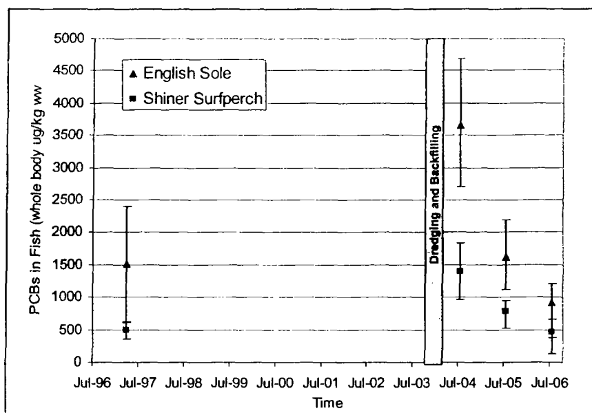
FIGURE 4-11 PCB concentrations in fish collected at the Duwamish Diagonal site pre- and post-dredging. Two trophic levels of fish (English sole and shiner surfperch) of consistent size range were collected within 1 km of the site at the time points indicated on the figure. Error bars represent the minimum and maximum values. Dredging was conducted at the site between November 14, 2003 and January 20, 2004. Capping was completed by February 29, 2004. Source: Adapted from Patmont 2006; Stern and Patmont 2006; Stern et al. 2007. Fish data were derived from King County 1999; King County, unpublished data, 2007; Windward 2005, 2006.
