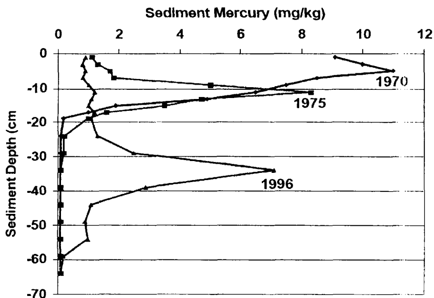
FIGURE 2-2 Historical changes in sediment core profiles of mercury concentrations collected from Bellingham Bay, WA, during natural recovery (dredging or capping was not performed). Sediment cores were taken over time (1970, 1975, 1996) from the same vicinity of Bellingham Bay in an area with a stable sediment deposit. At this site, mercury was released from a nearby facility from 1965 until controls were put in place in 1971. Sedimentation has since continued to bury the contaminants. Source: Patmont et al. 2004. Reprinted with permission from authors; copyright 2003, Battelle Press.
