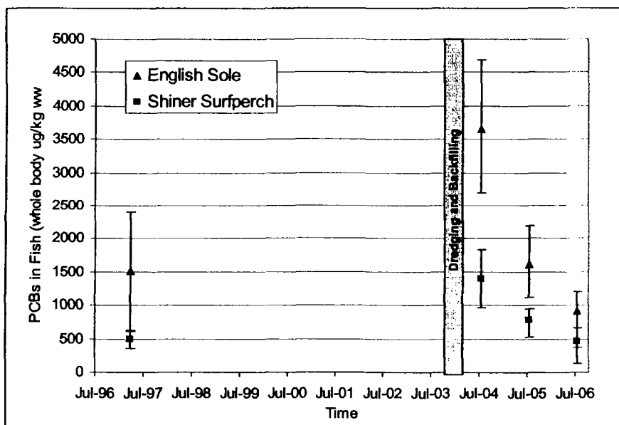
FIGURE 4-11 PCB concentrations in fish collected at the Duwamish Diagonal site pre- and post-dredging. Two trophic levels of fish (English sole and shiner surfperch) of consistent size range were collected within 1 km of the site at the time points indicated on the figure. Error bars represent the minimum and maximum values. Dredging was conducted at the site between November 14, 2003 and January 20, 2004. Capping was completed by February 29, 2004. Source: Adapted from Patmont 2006; Stern and Patmont 2006; Stern et al. 2007. Fish data were derived from King County 1999; King County, unpublished data, 2007; Woodward 2005, 2006.
