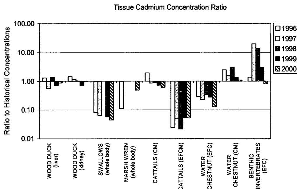
FIGURE 4-5 Ratio of cadmium body burdens in various animals and plants after dredging to pre-dredging levels for the period 1996-2000, Marathon Battery Site, NY. The data are the mean value except for the benthic invertebrates for which only one sample was collected. 10 The number of samples in each mean varies. CM = Constitution Marsh; EFCM = East Foundry Cove Marsh; EFC = East Foundry Cove. (Data source: AGC 2001). Note that only the water chestnuts (EFC) and the benthic invertebrates (EFC) were from locations where dredging alone was conducted.
