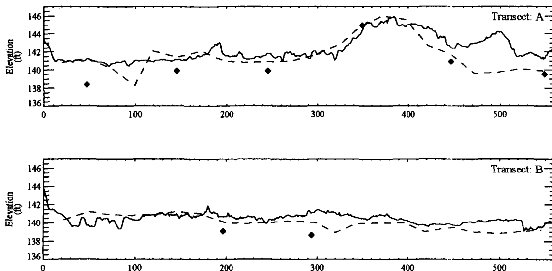
FIGURE 4-14 Upstream to downstream transects of the Grasse River remediation area showing: elevations of probing based cut line (dotted lines) based on the pre-dredging (spring 2005) estimated depth of contamination; post-dredging (fall 2005) extent of contamination (diamonds) determined by vibracore sampling; and, the post-dredging (fall 2005) bottom elevation determined by bathymetry. Source: Connolly et al. 2007. Reprinted with permission from authors; copyright 2006, Quantitative Environmental Analysis.
