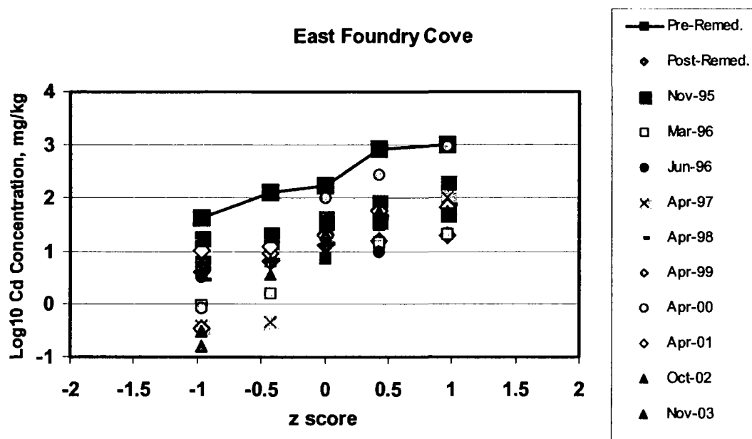
FIGURE 4-4 Log probability plot of sediment cadmium concentrations, East Foundry Cove, Marathon Battery, NY. The z score indicates the distance from the mean in standard deviations; z scores greater than 0 exceed the mean. The source of these data is described in Figure 4-3.
