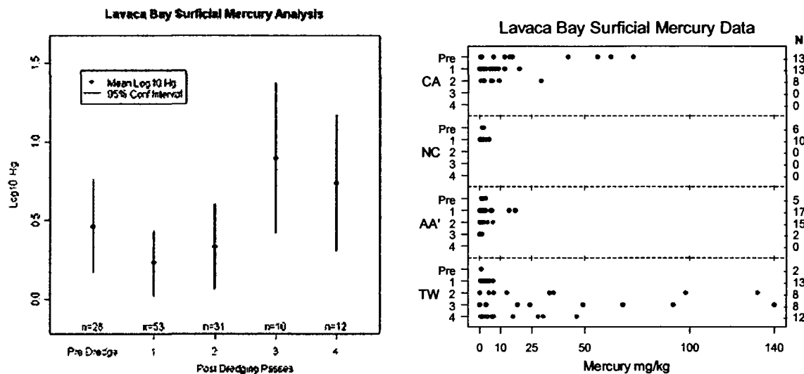
FIGURE 4-12 Left, mean and 95% confidence intervals of surficial mercury concentrations (mg/kg) (log base 10 scale) for each dredging time (before dredging and after each of four passes). Right, concentration distribution and sample sizes (N) of surficial mercury stratified by geographic region—Capa (CA), North Capa (NC), AA', and the Trench Wall (TW)—and dredging pass (Pre, 1, 2, 3, 4; pre = pre-dredging).
