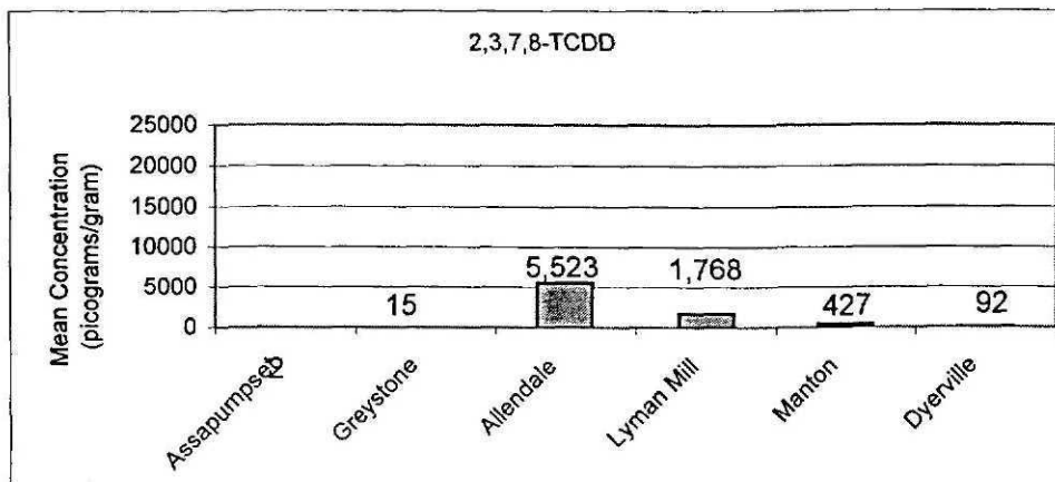
Figure 49 2,3,7,8-TCDD, HCX, and PCB-77 Concentrations in Sediment Baseline Human Health Risk Assessment Centredale Manor Restoration Project Superfund Site North Providence, Rhode Island
