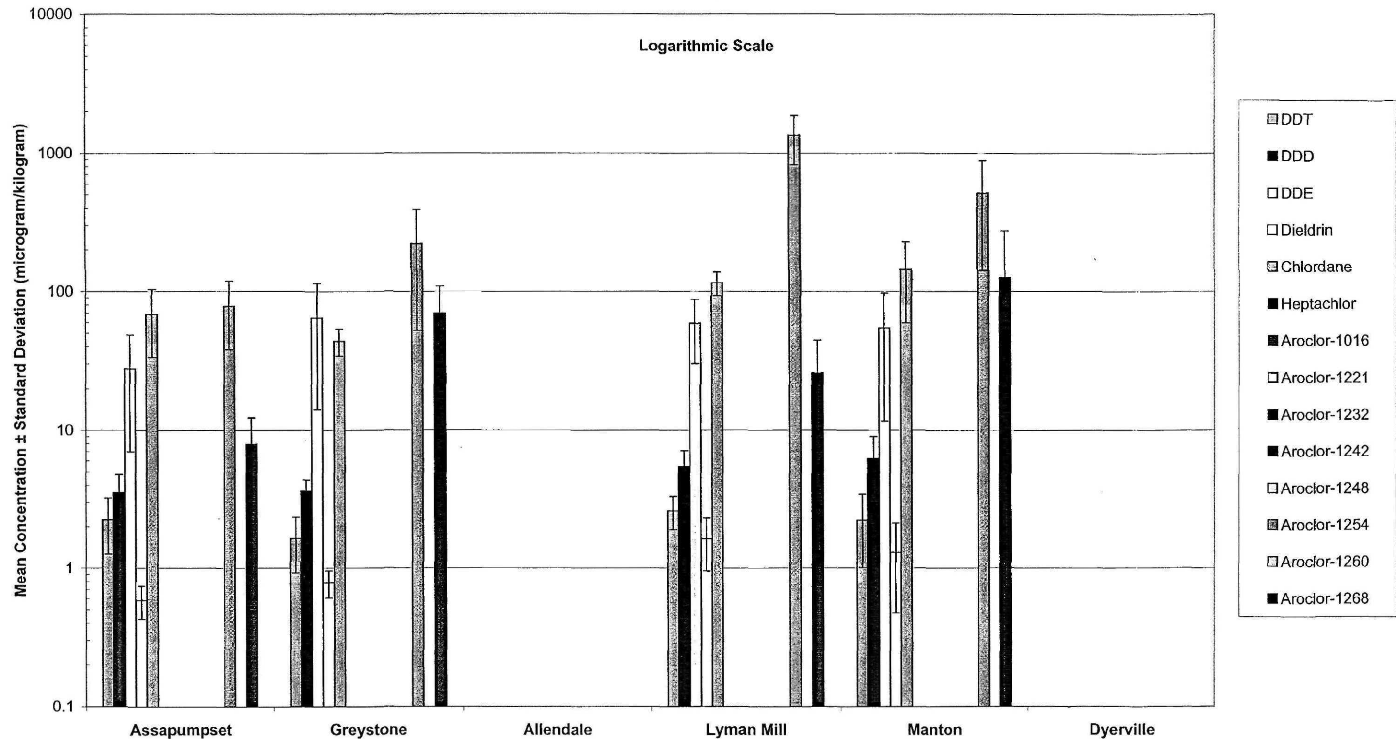
Figure 32 Select Pesticide and PCB Aroclor Concentrations in Largemouth Bass Baseline Ecological and Human Health Risk Assessment Centredale Manor Restoration Project Superfund Site North Providence, Rhode Island
