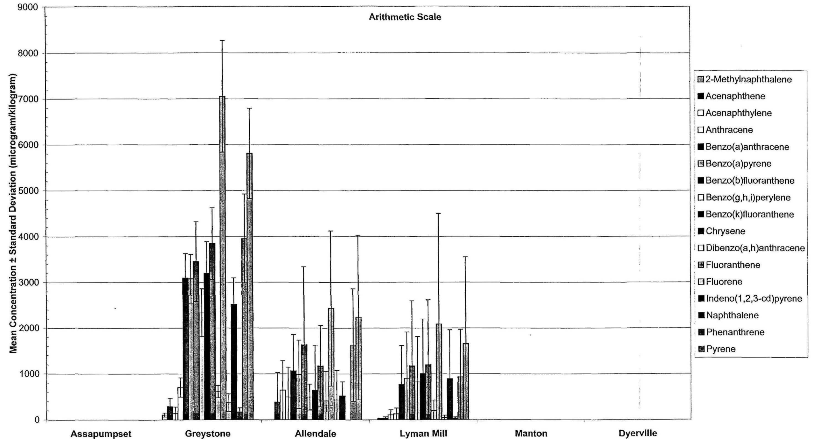
Figure 23 Select PAH Concentrations in Floodplain and Bank Soil Baseline Ecological and Human Health Risk Assessment Centredale Manor Restoration Project Superfund Site North Providence, Rhode Island
