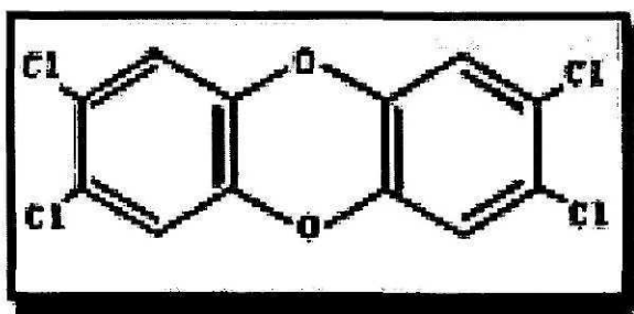
2,3,7,8-Tetrachlorodibenzo-p-dioxin
