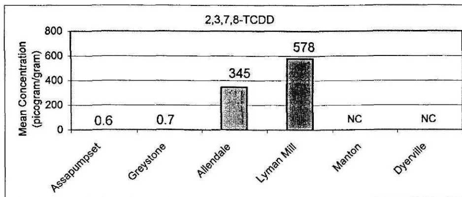
Figure 50 2,3,7,8-TCDD, HCX, and PCB-77 Concentrations in White Sucker Baseline Human Health Risk Assessment Centredale Manor Restoration Project Superfund Site North Providence, Rhode Island
