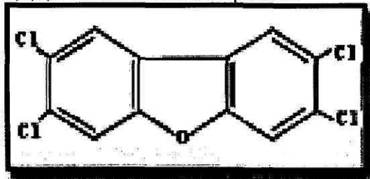
2,3,7,8-Tetrachlorodibenzofuran
