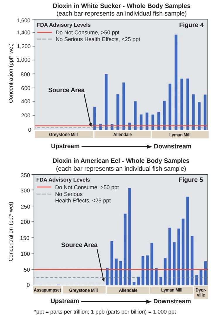
Figures 4 and 5 Concentrations of dioxin in white sucker (Figure 4) and American eel (Figure 5) frequently exceeded the FDA "Do Not Consume" levels in areas immediately downstream of the project. Dioxin was either not detected or found at very small concentrations in fish caught at the reference locations.
