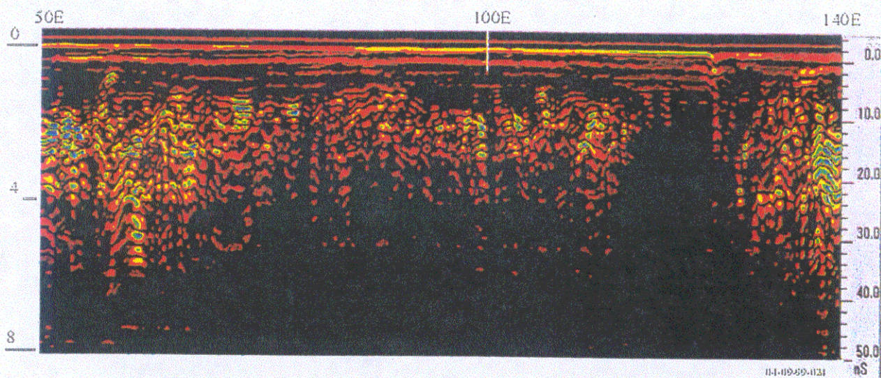
Transect: 125S
