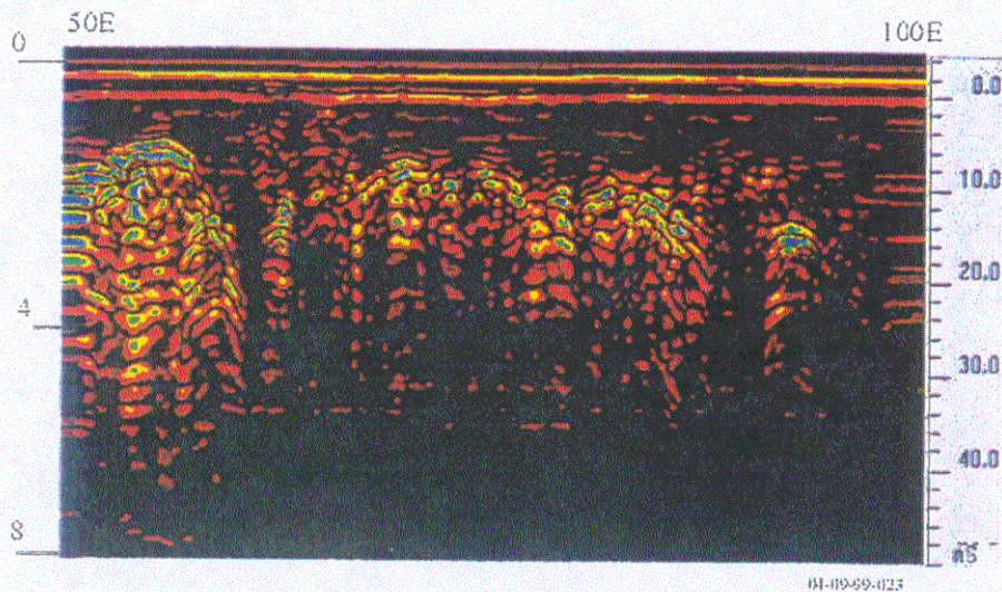
Transect: 125S
