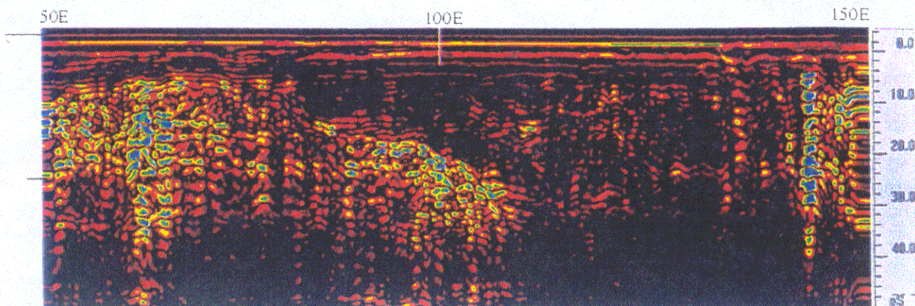
Transect: 175S
