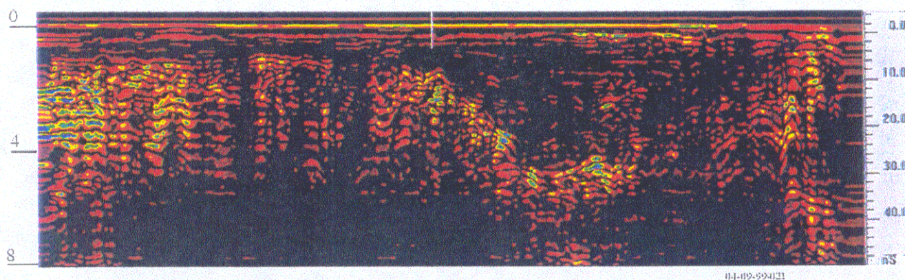
Transect: 175S
