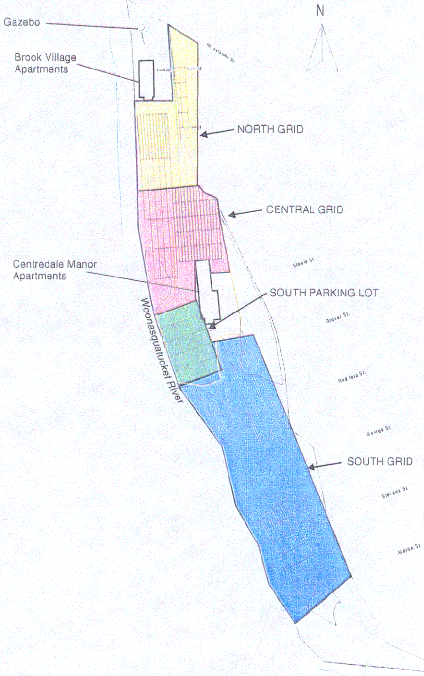
FIGURE 1 GEOPHYSICAL SURVEY GRID CENTREDALE MANOR SITE PROVIDENCE, R.I. APRIL, 1999
