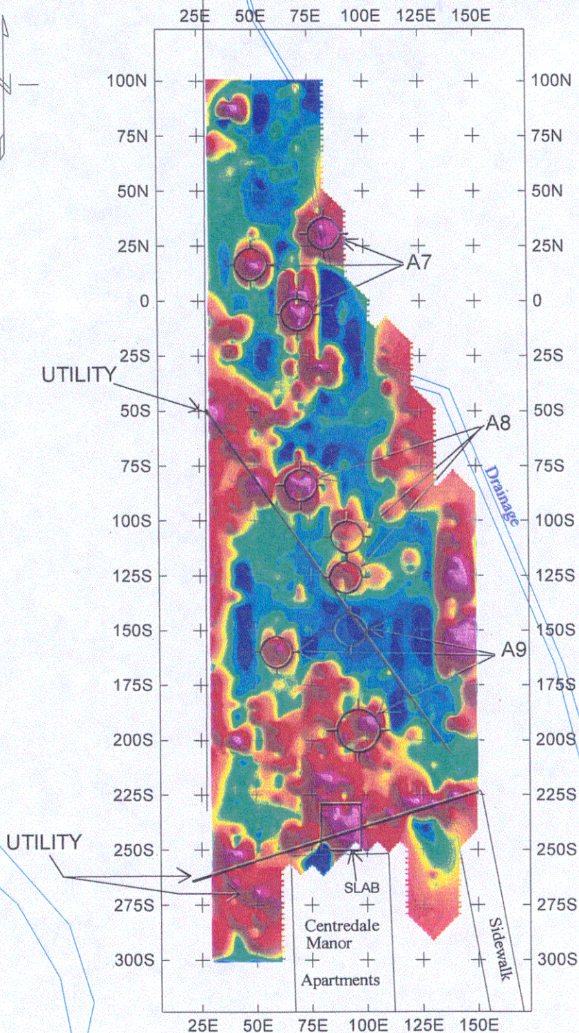
Figure 9 - EM-61 Survey (Bottom Channel)
