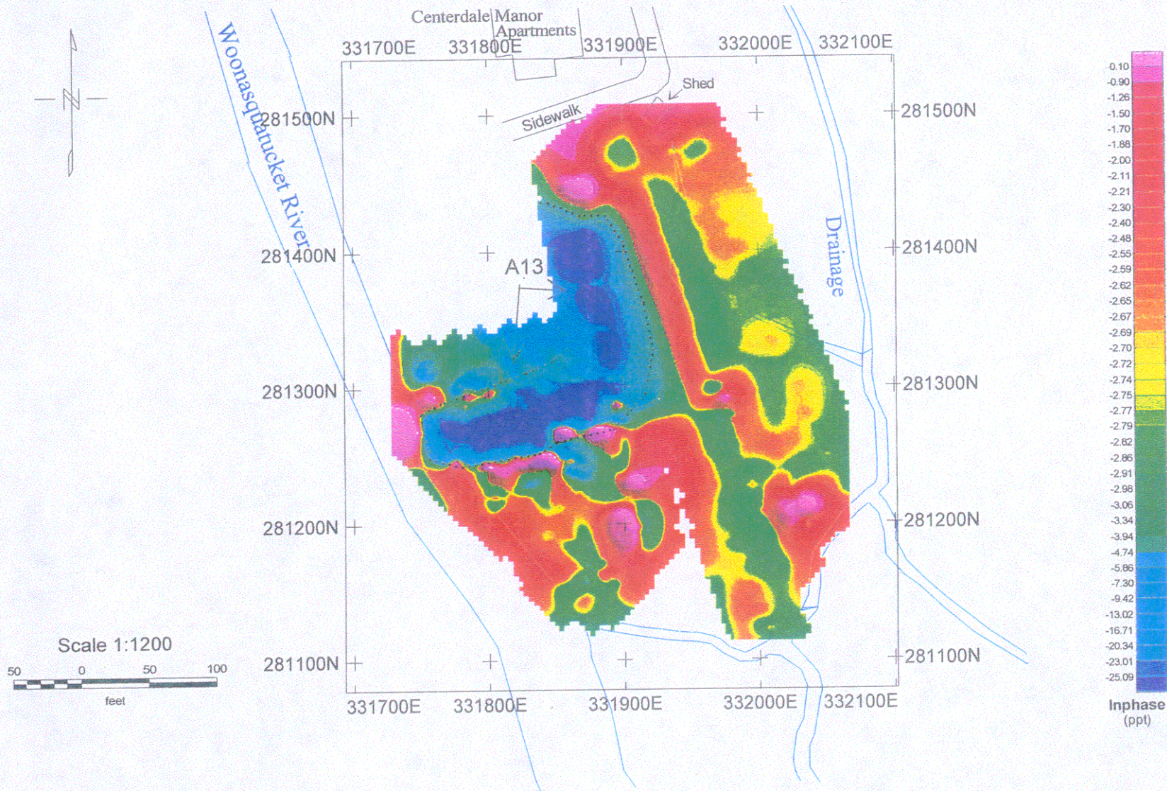
Figure 15 - EM-31 Survey (Inphase Plot)
