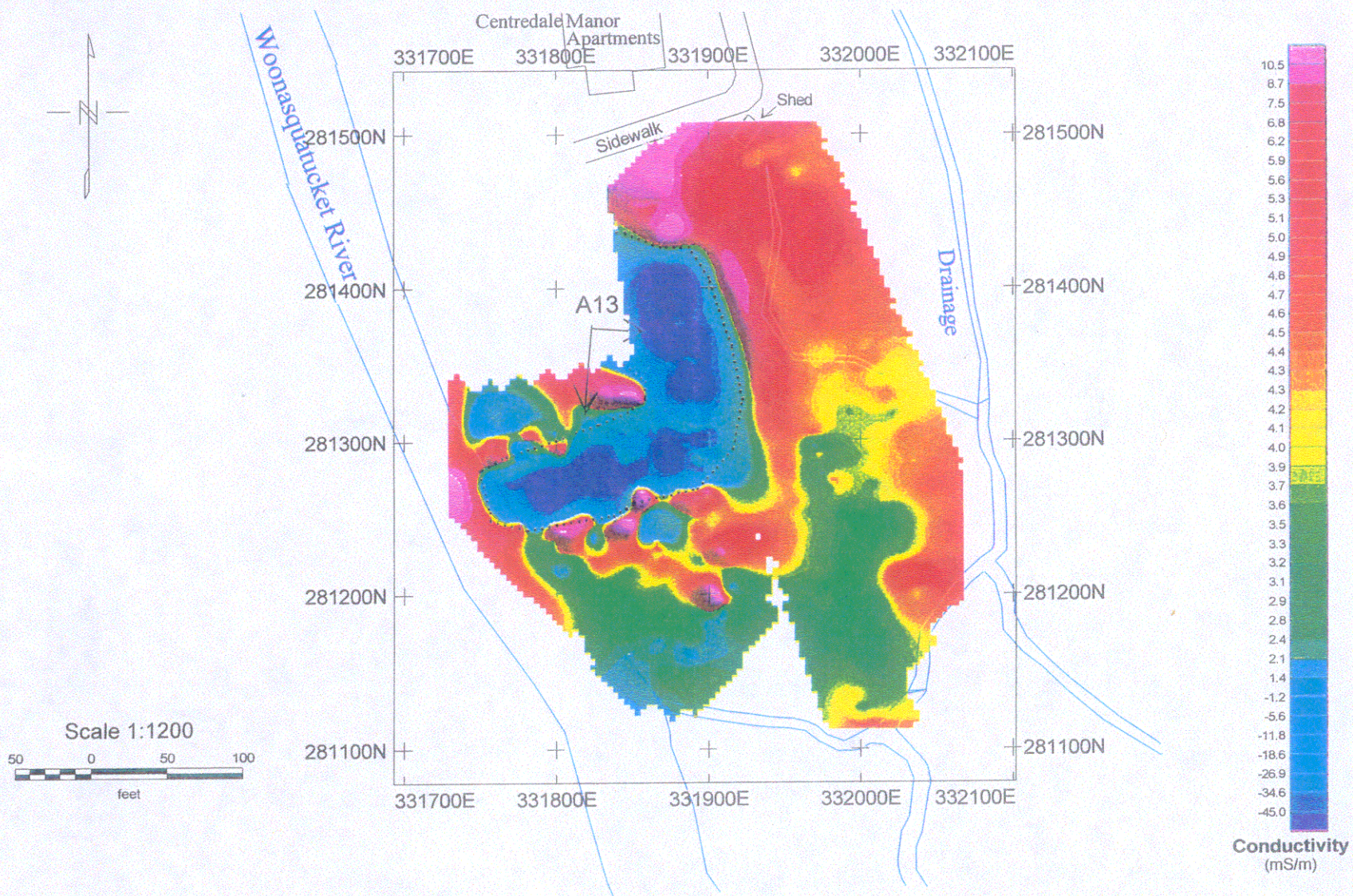
Figure 14 - EM-31 (Conductivity Plot)
