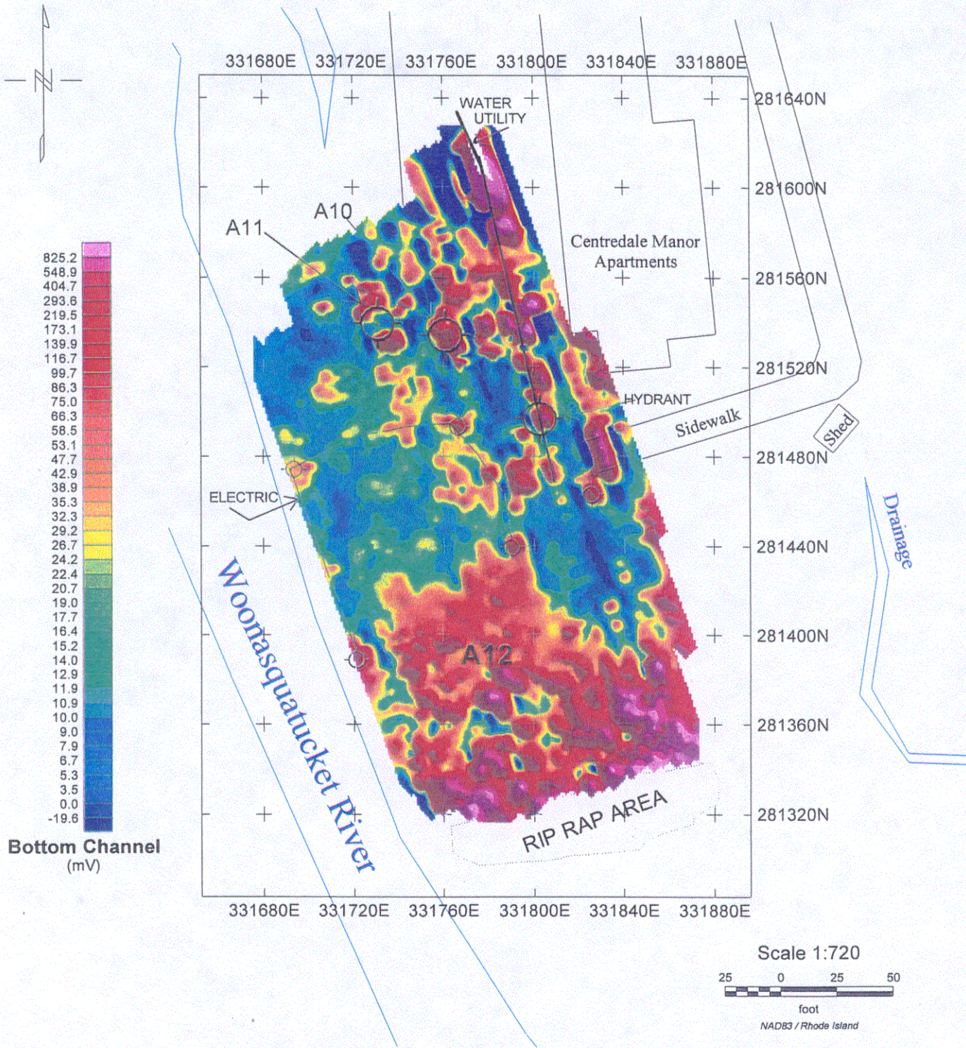
Figure 12 - EM-61 Survey (Bottom Channel)
