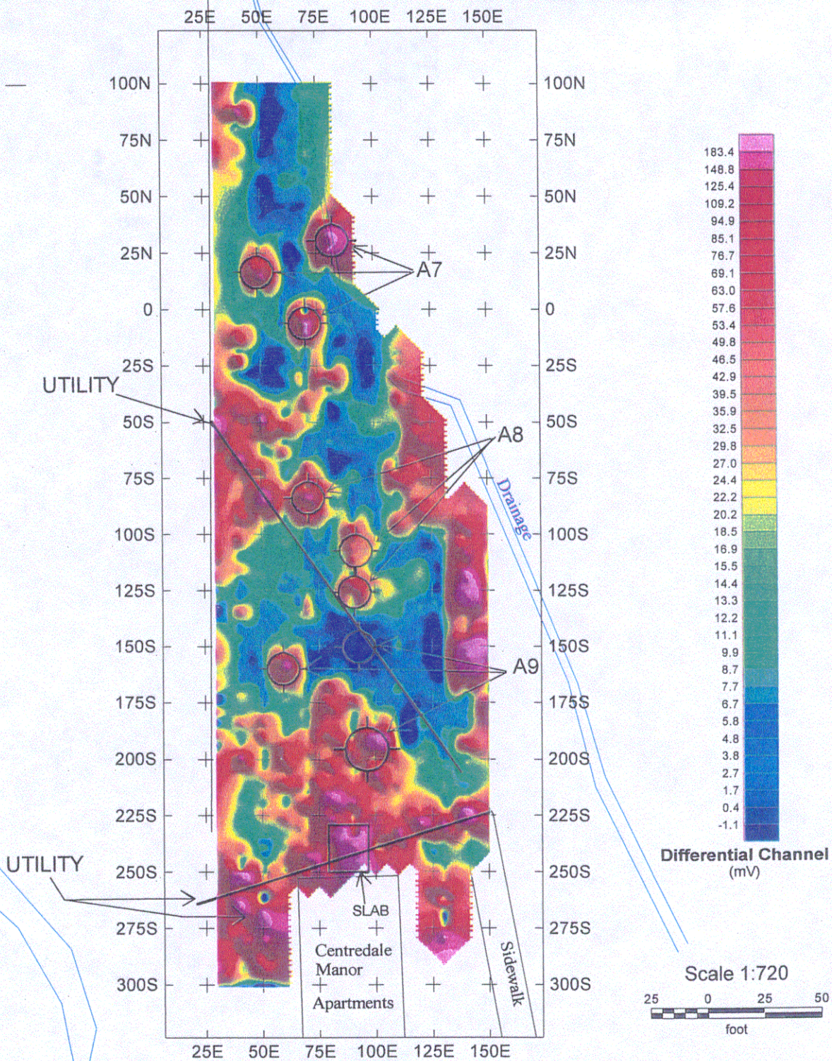
Figure 10 - EM-61 Survey (Differential Channel)
