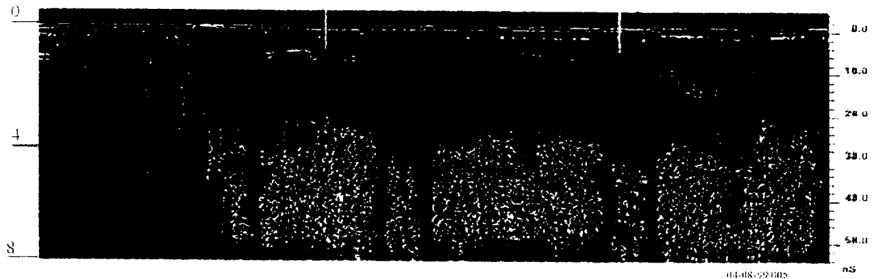
Transect: 50W
