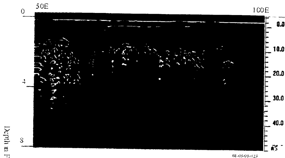
Transect: 125S
