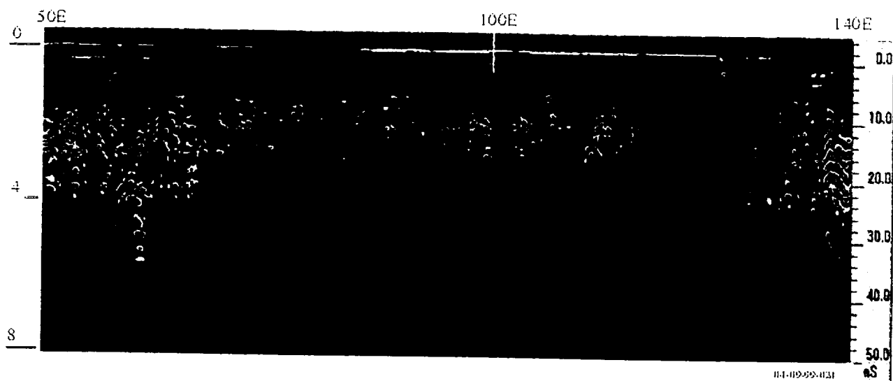
Transect: 125S
