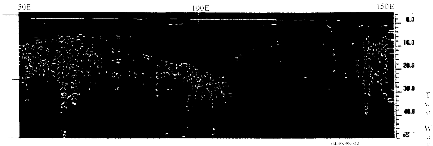
Transect: 175S
