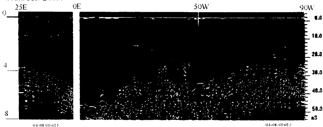
Transect: 200N
