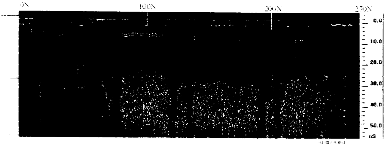
Transect: 50W
