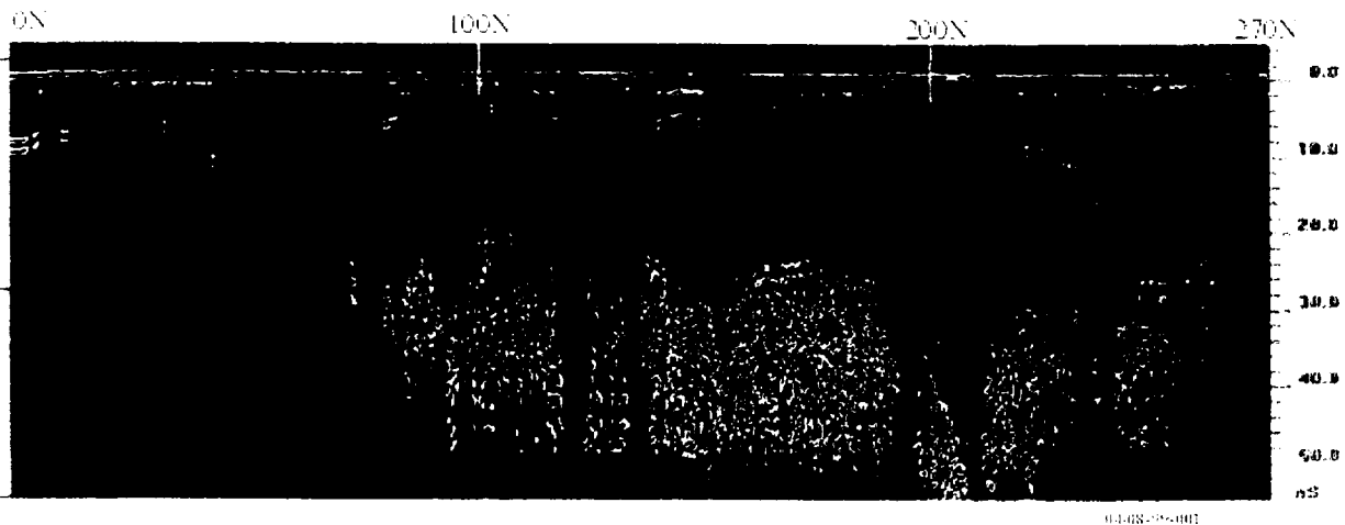
Transect: 20W
