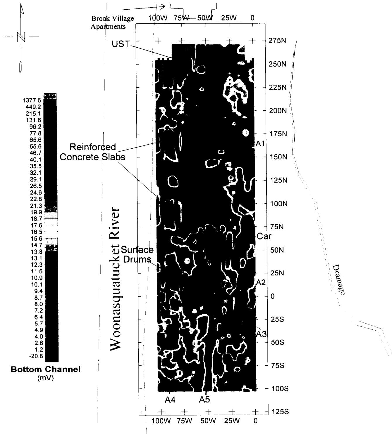
Figure 6 - EM-61 Survey (Bottom Channel)
