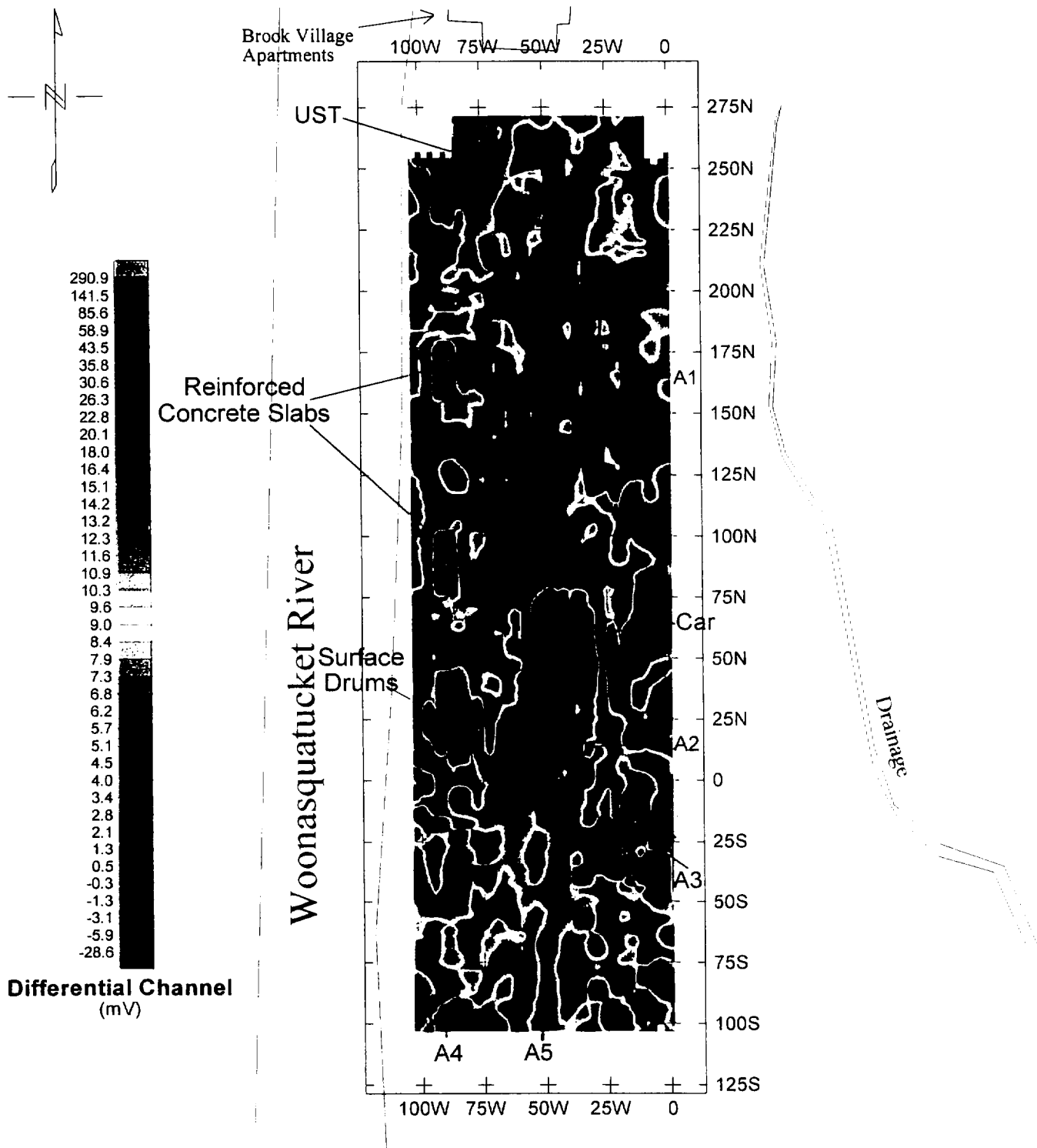
Figure 7 - EM-61 Survey (Differential Channel)
