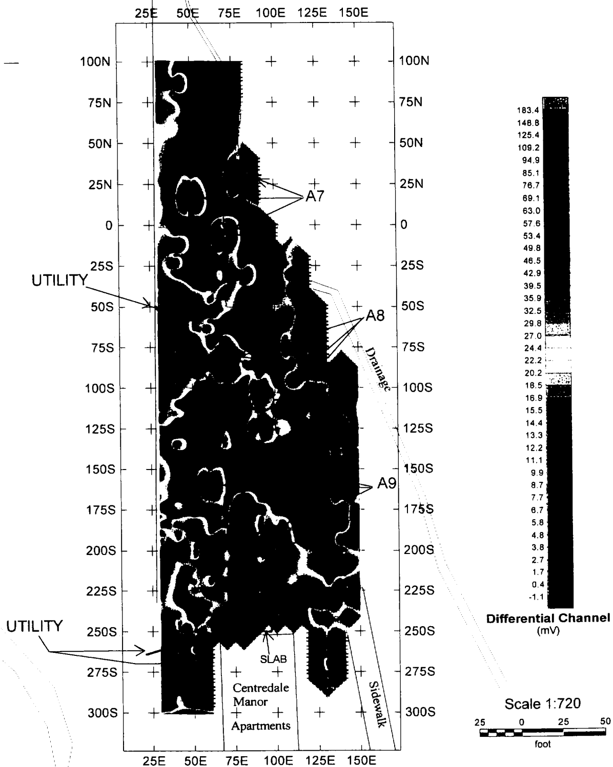
Figure 10 - EM-61 Survey (Differential Channel)
