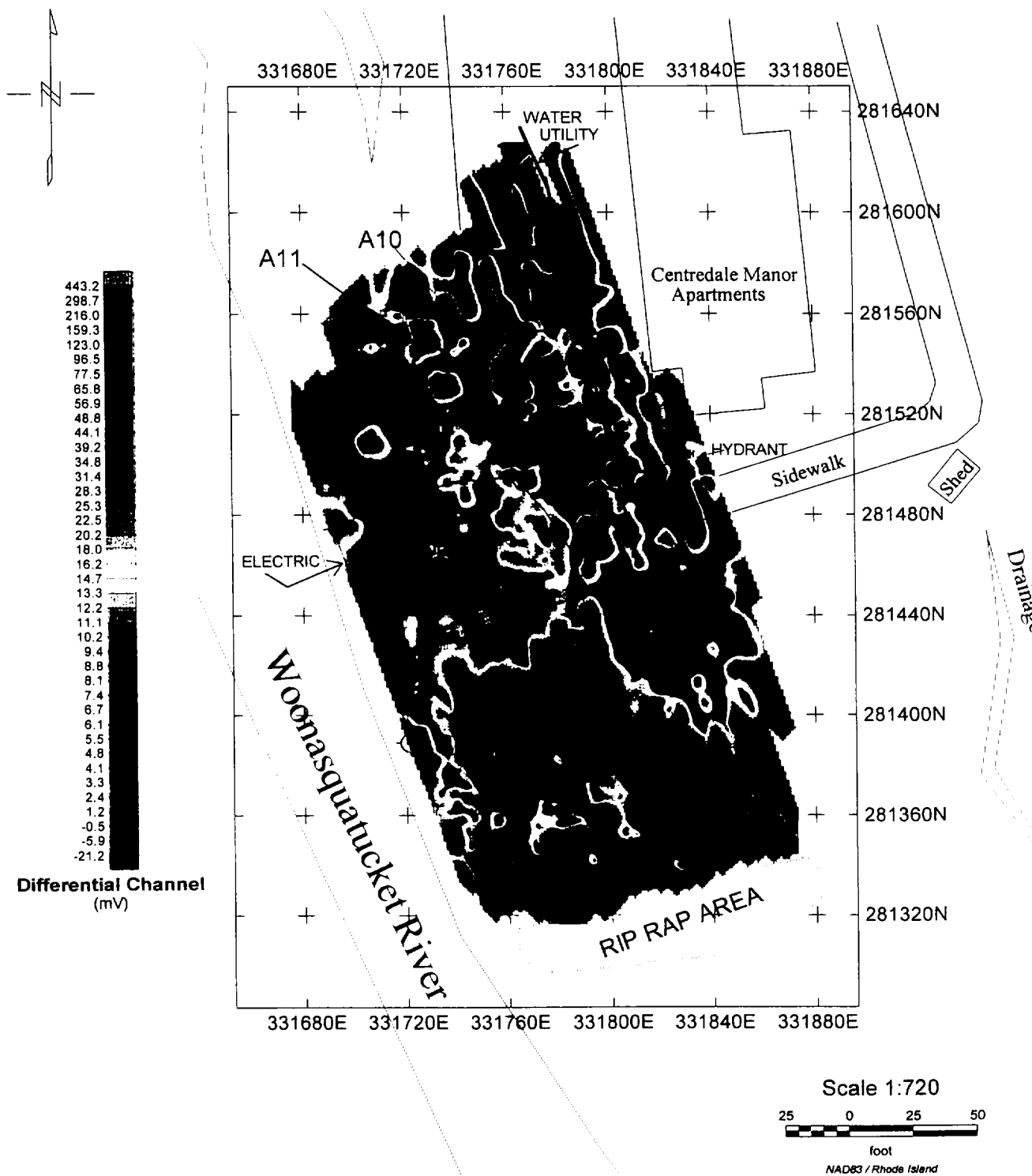
Figure 13 - EM-61 Survey (Differential Channel)
