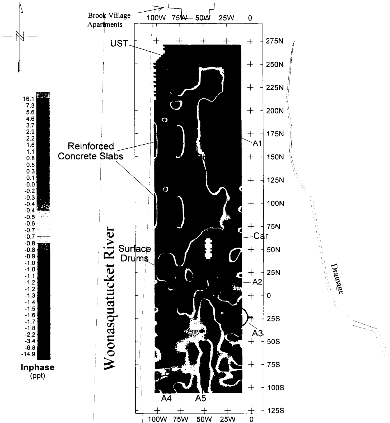
Figure 5 - EM-31 Survey (Inphase Plot)
