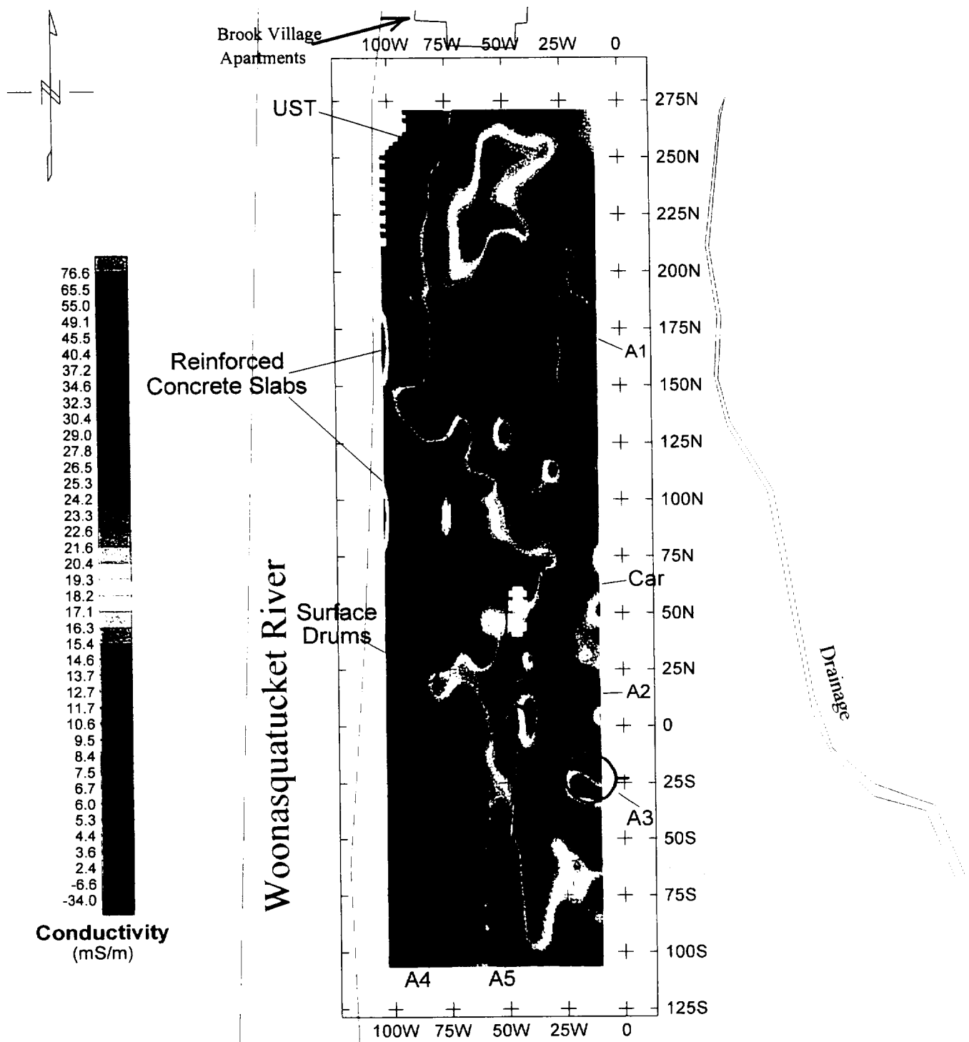
Figure 4 - EM-31 Survey (Conductivity Plot)
