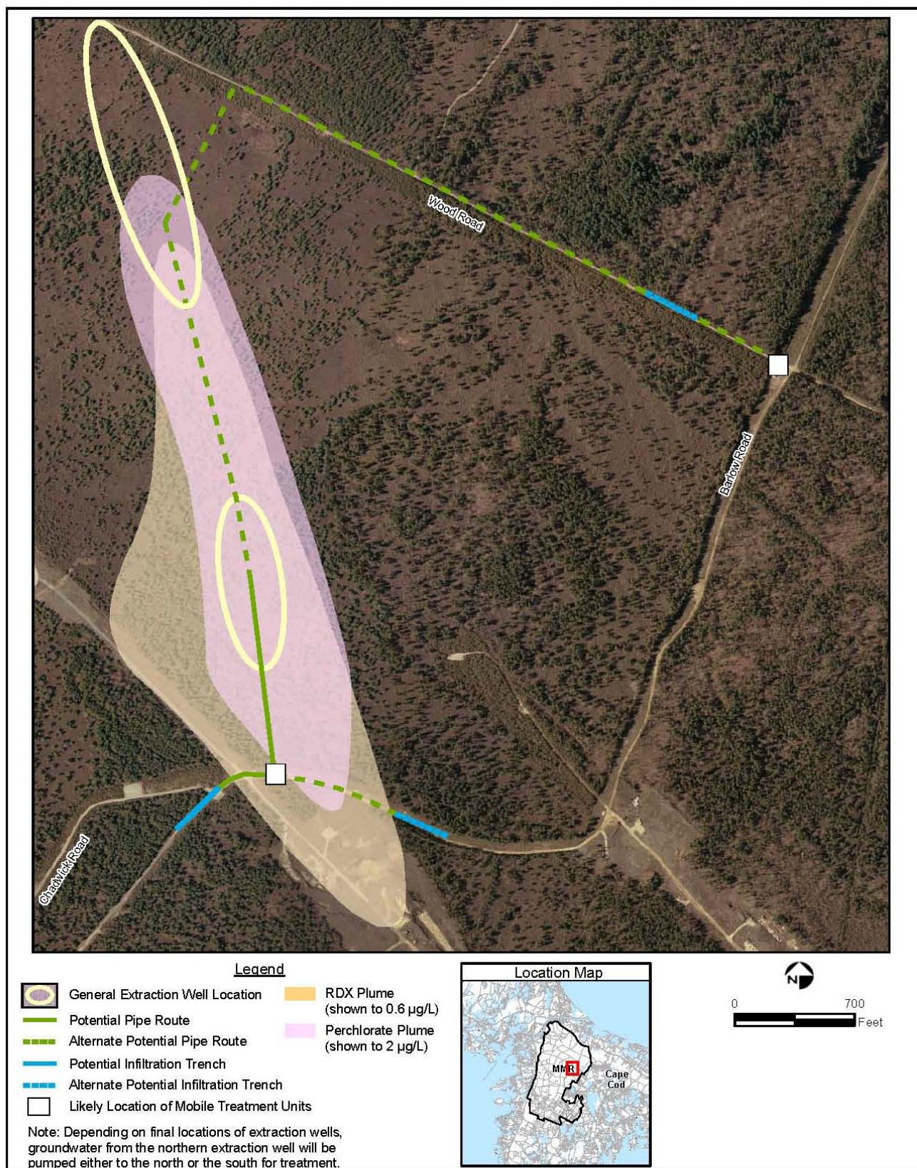
Conceptual J-1 Northern Extraction Well Locations and Pipelines
