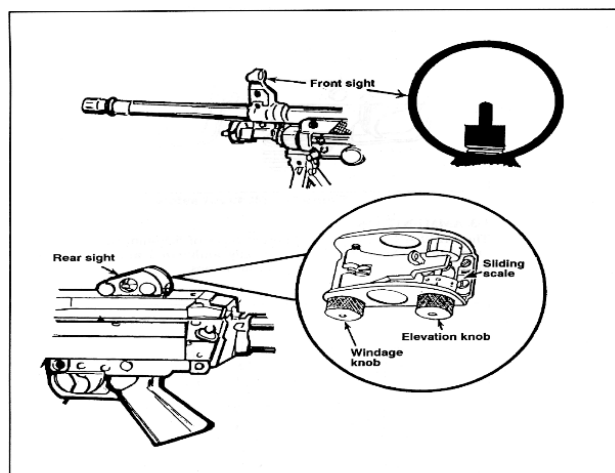
Figure 2-3. Front and Rear Sights
