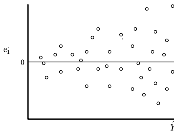
Figure 10.9 Heteroscedastic data.
