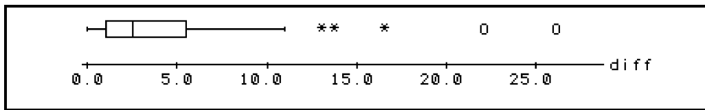
Figure 6.2 Boxplot of asymmetric D_i = x_i - y_i
