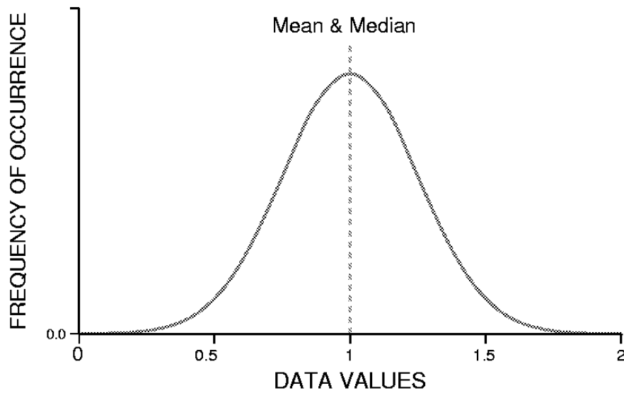
Figure 1.2 Density Function for a Normal Distribution
