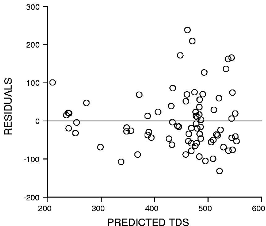
Figure 9.9 Residuals plot of the Cuyahoga data.
