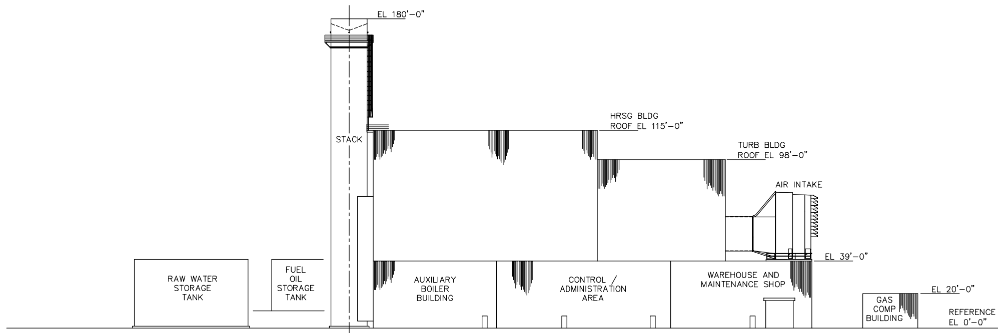
SECTION A-A (LOOKING EAST)
