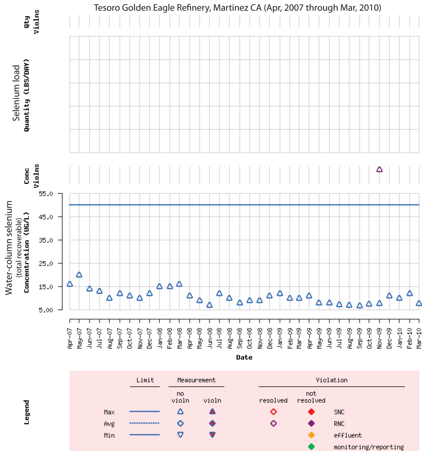
Figure C3. Water-column selenium concentrations, Tesoro Golden Eagle Refinery, Martinez, California.
