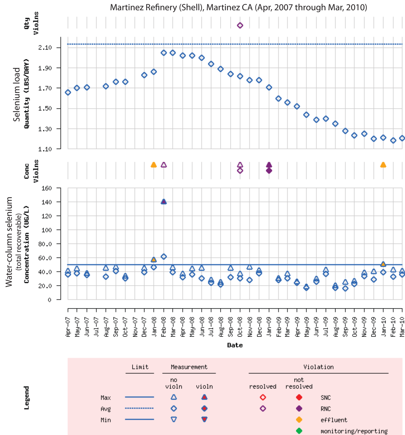
Figure C2. Water-column selenium concentrations and selenium loads, Martinez Refinery (Shell), Martinez, California.
