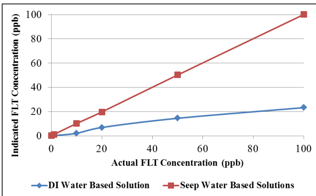
Figure 3-10: Turner 10AU response to DI water based and submarine spring water based FLT solutions.
