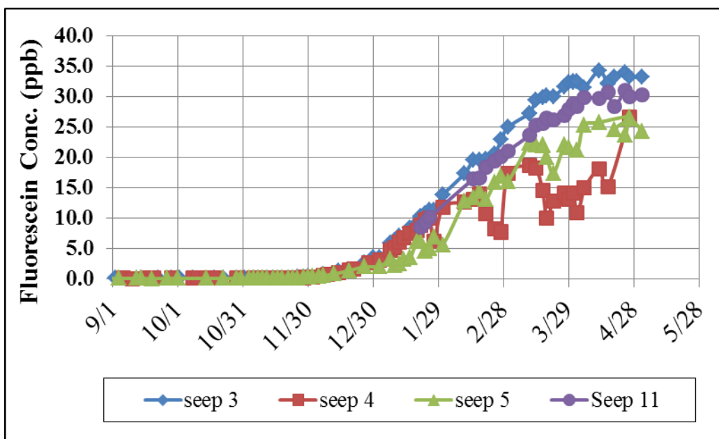
Figure 3-14: Fluorescein breakthrough curve for the SSG.
