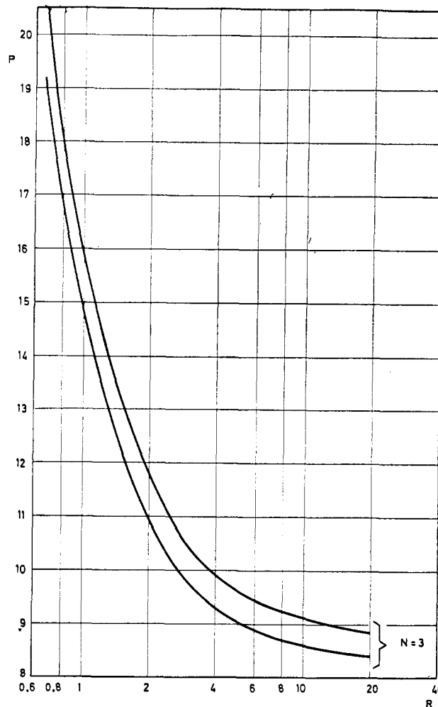
Figure 3. Influence of range ( R ) on the decision limit, in the case of three standards, with \alpha = 5\% ; P is in ordinates
