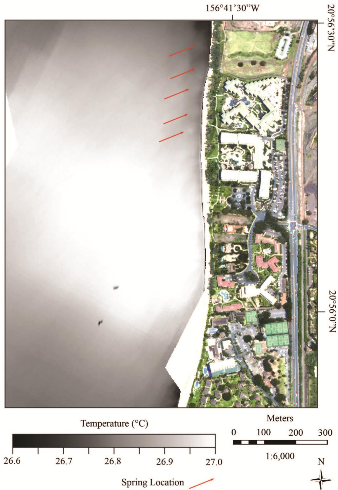
Figure 4-5: Submarine spring locations. Data are displayed on a gray-scale sea-surface temperature map.
