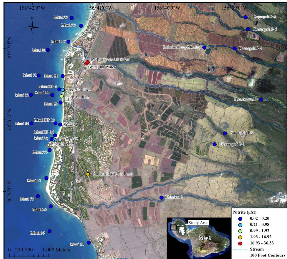
Figure E-23: September, 2011 \text{NO}_2^- distribution.
