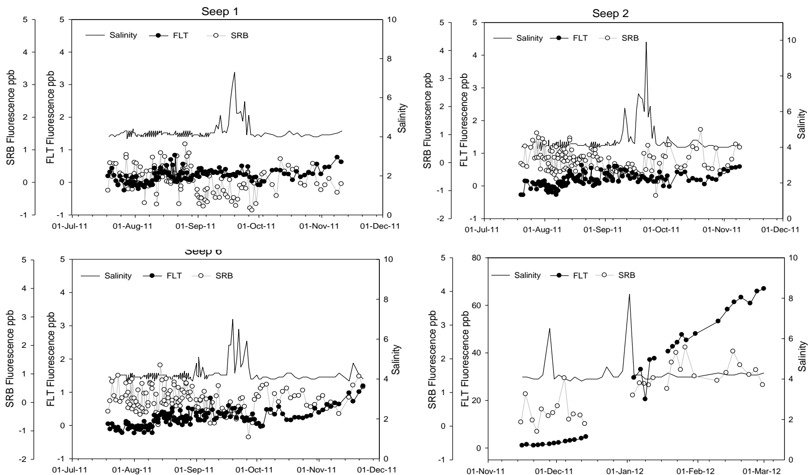
Figure 2-9: North Seep Group salinity and fluorescence (Seeps 1, 2, 6, 7).
