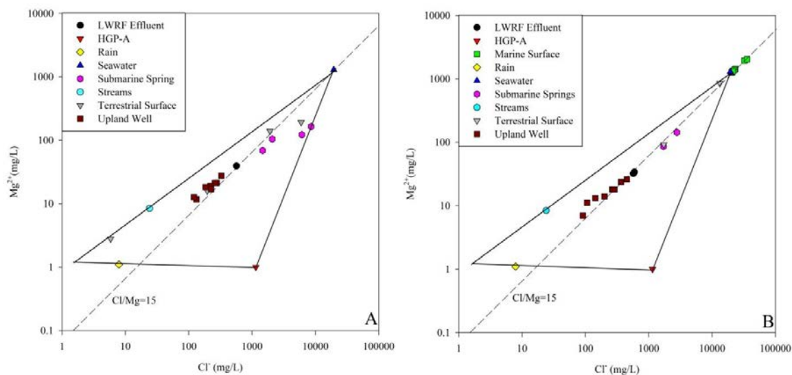
Figure 4-6: Log-Log plot of magnesium versus chloride ion concentrations.
