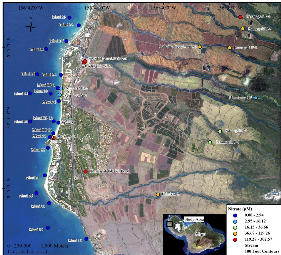
Figure E-24: September, 2011 \text{NO}_3^- distribution.
