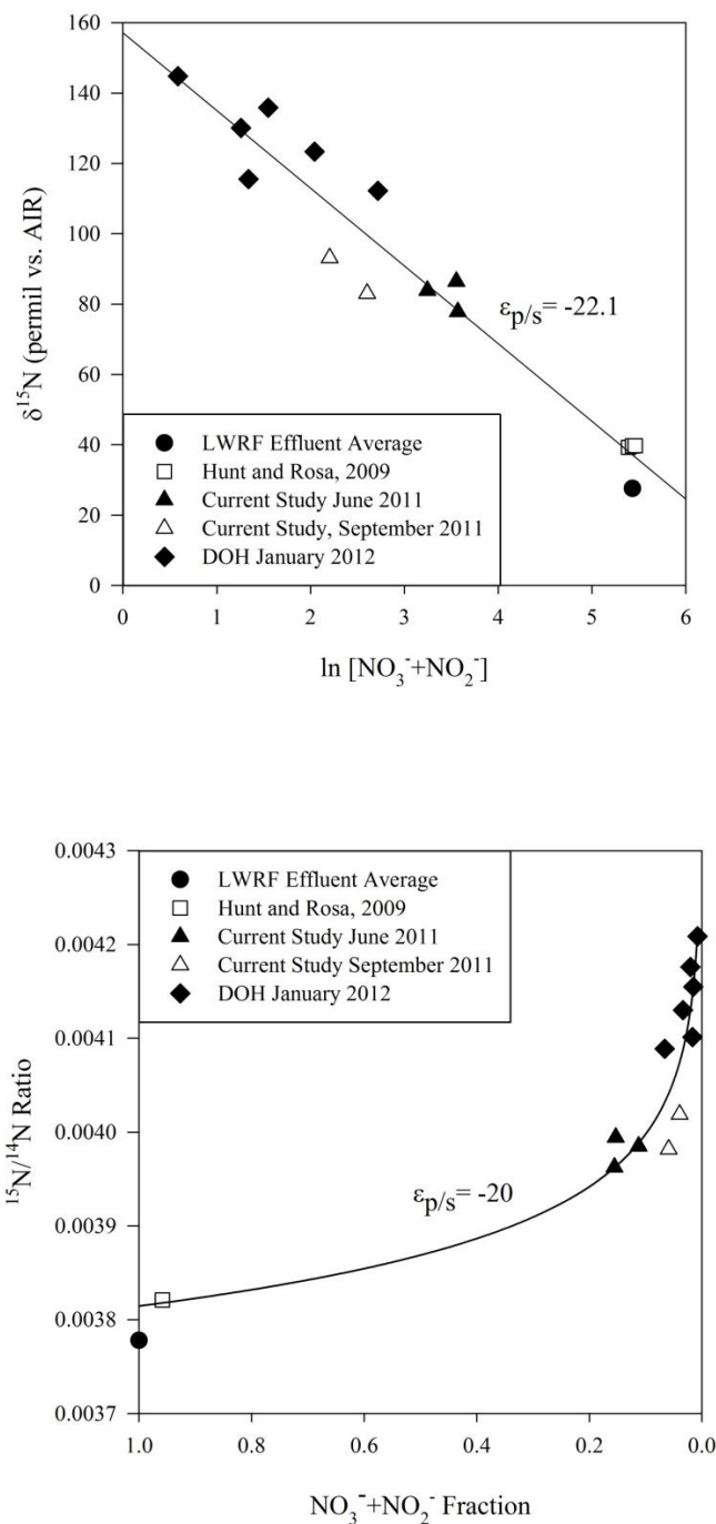
Figure 6-24: Historical data plots of \ln[\text{NO}_3^- + \text{NO}_2^-] with \delta^{15}\text{N} values (top) and \text{NO}_3^- + \text{NO}_2^- fraction with ^{15}\text{N}/^{14}\text{N} ratio (bottom).
