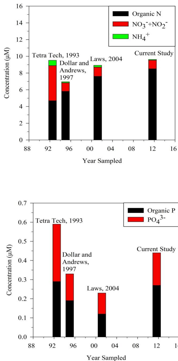
Figure 6-20: Chronology of N (top) and P (bottom) in coastal marine samples in the study area.
