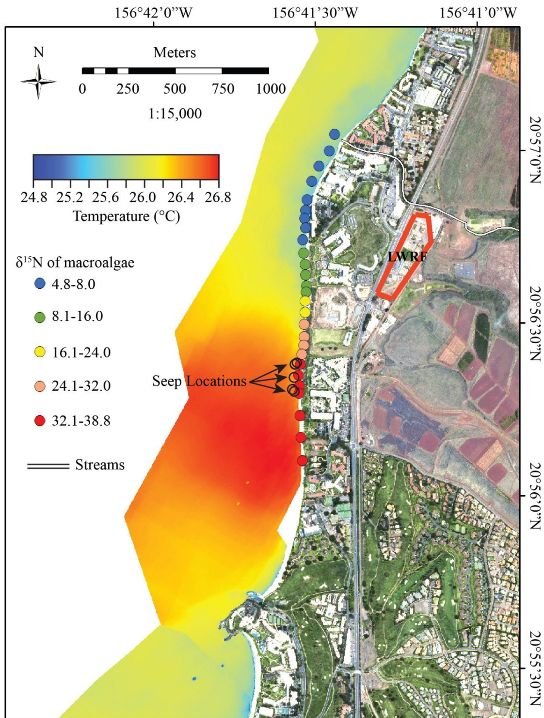
Figure 4-7: \delta^{15}\text{N} (macroalgae) overlain on the sea-surface temperature map. Nitrogen isotopic data of macroalgae from Dailer et al. (2010); the highest \delta^{15}\text{N} values of macroalgae occur near submarine spring locations and within the thermal anomaly.
