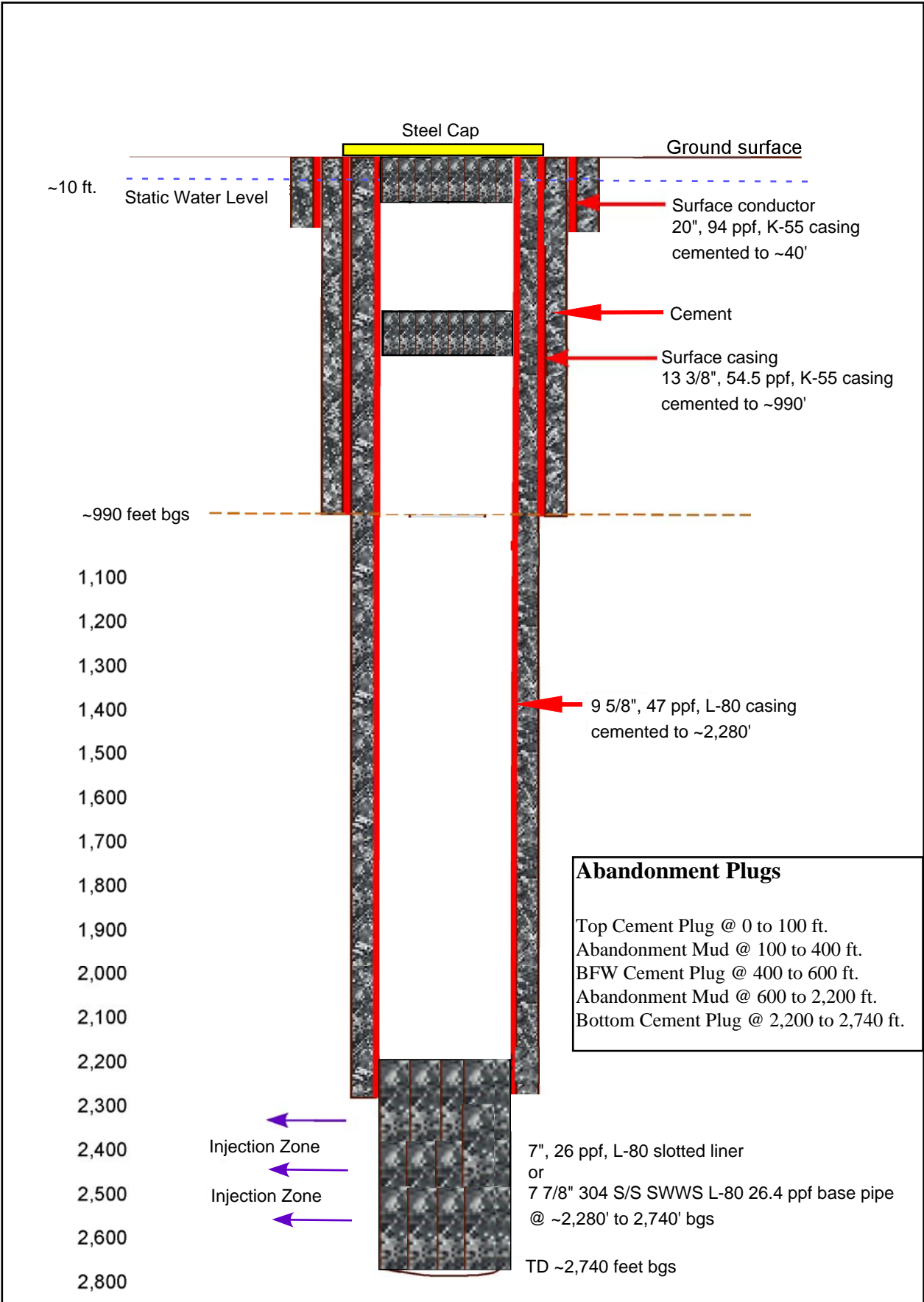
General Abandonment Plan for All Wells El Centro Generating Station Imperial Irrigation District Figure Q1
