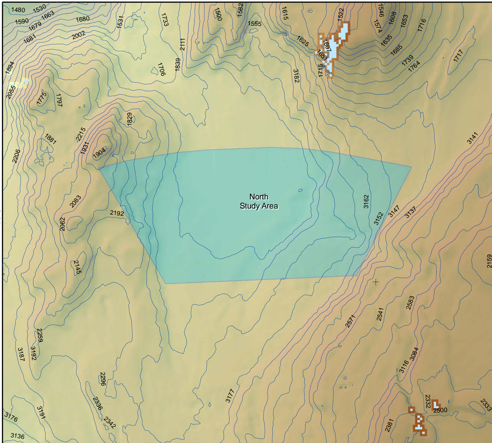
Figure 3-24 North Study Area Bathymetry
