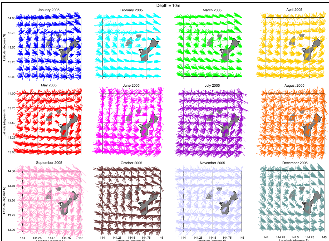
Figure 3-2. Vector Plots of Daily Averaged Current Velocities by Month for Each Location at 33 ft (10 m) Depth
