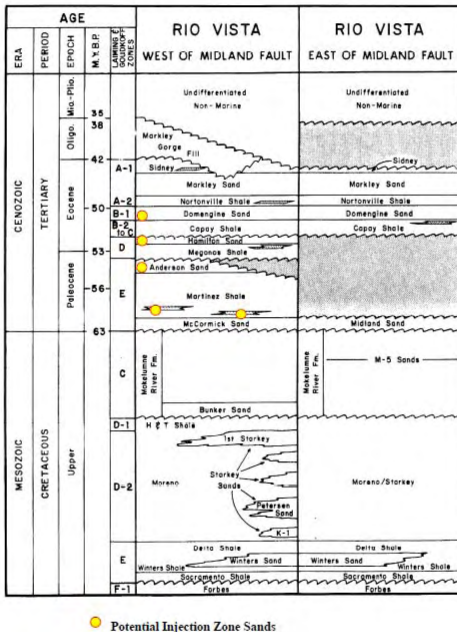
Figure 4. Stratigraphic column for the Rio Vista Field showing potential injection zone sand formations (from Attachment F of the Permit Application).
