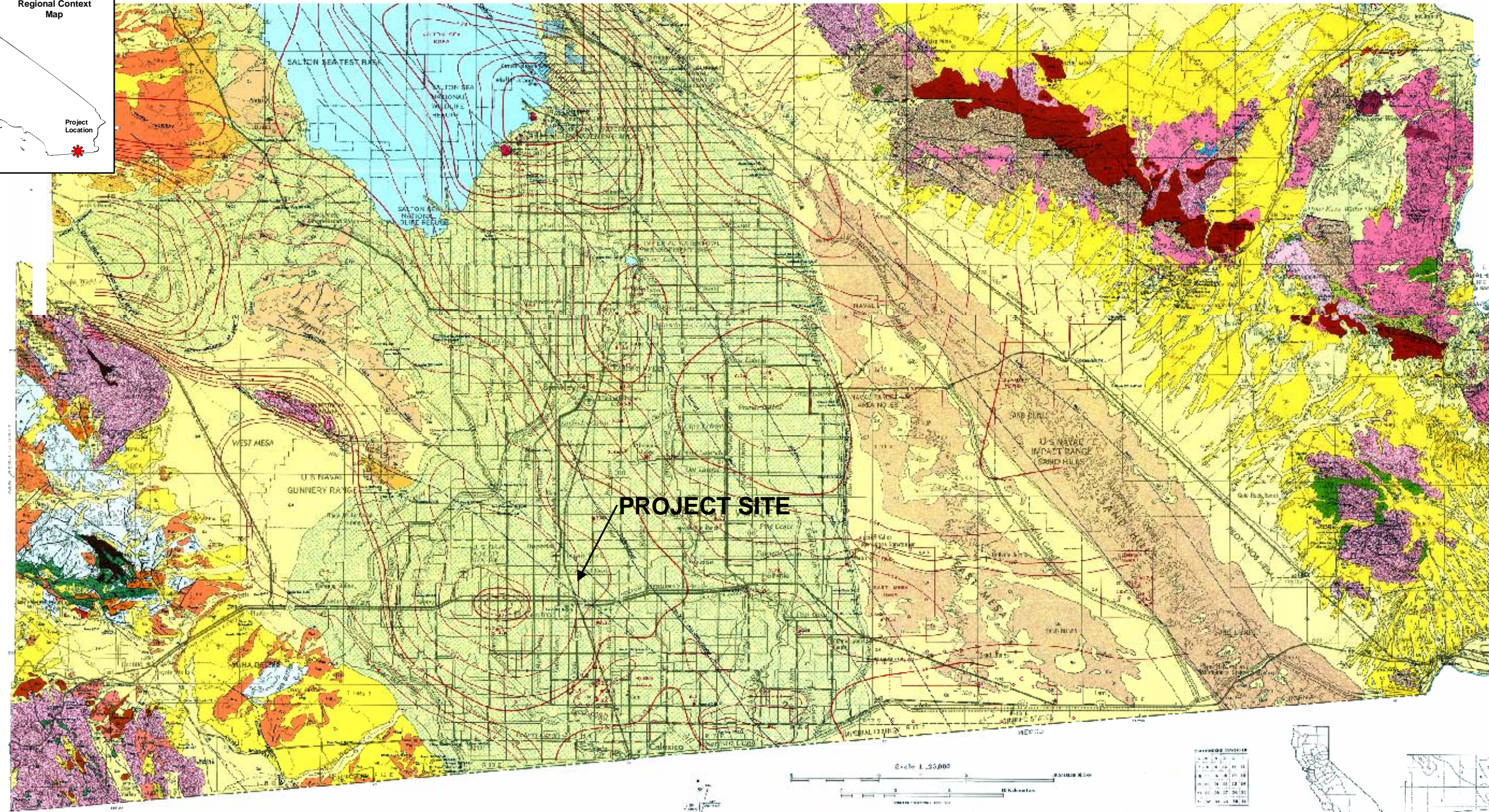
GEOLOGIC MAP OF IMPERIAL COUNTY, CALIFORNIA SHOWING UNITS AND SYMBOLS Compiled by Paul S. Moore 1989
