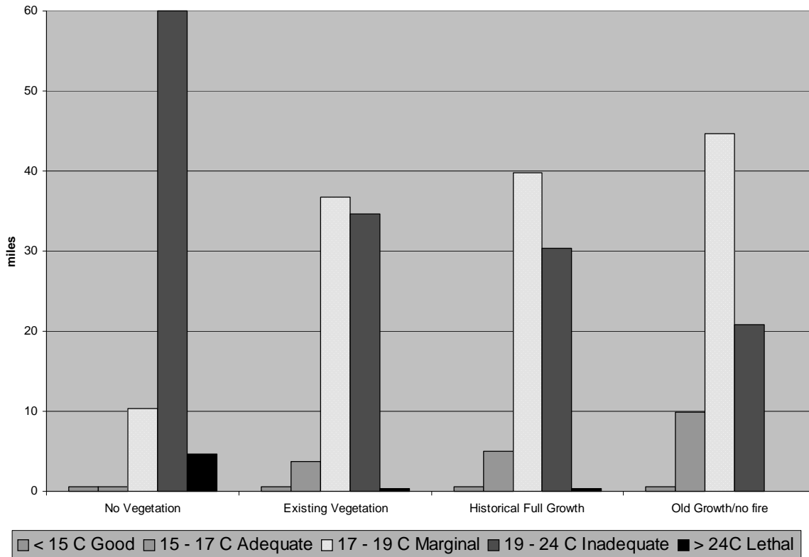
Figure 3-6: Quality of Stream Temperatures for steelhead for different vegetation scenarios area north of Yellowjacket Creek - in stream miles -
