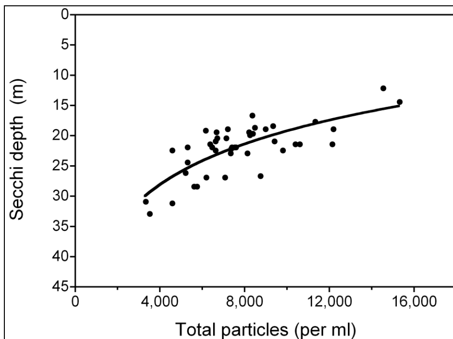
Figure 3-1. Relationship between in-lake particle number (< 16 µm) and Secchi depth with P-value = 0.001 and R^2 = 0.057 (modified from Swift 2004).
