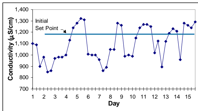
Figure 5. Rinse Water Conductivity Measurements Taken Before Installing a Conductivity Control System to Determine the Initial Set Point
