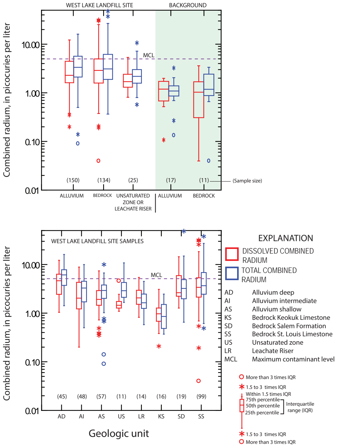
Figure 9. Box plots showing concentrations of dissolved and total combined radium in groundwater samples from monitoring wells in various geologic units at the West Lake Landfill site. Data from 2012-14.
