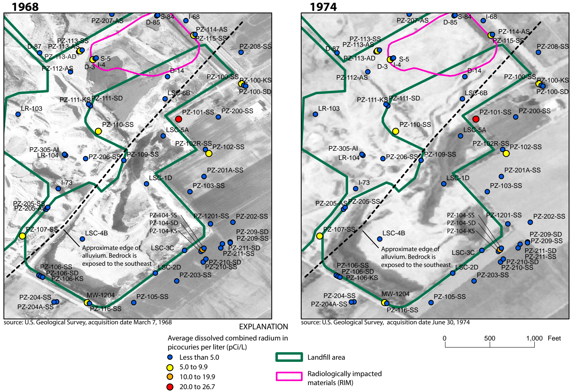
Figure 17. Average dissolved combined radium in monitoring wells near the North and South quarry areas at the West Lake Landfill site in relation to site features shown on 1968 and 1974 aerial photographs. Imagery obtained from U.S. Geological Survey (2014).
