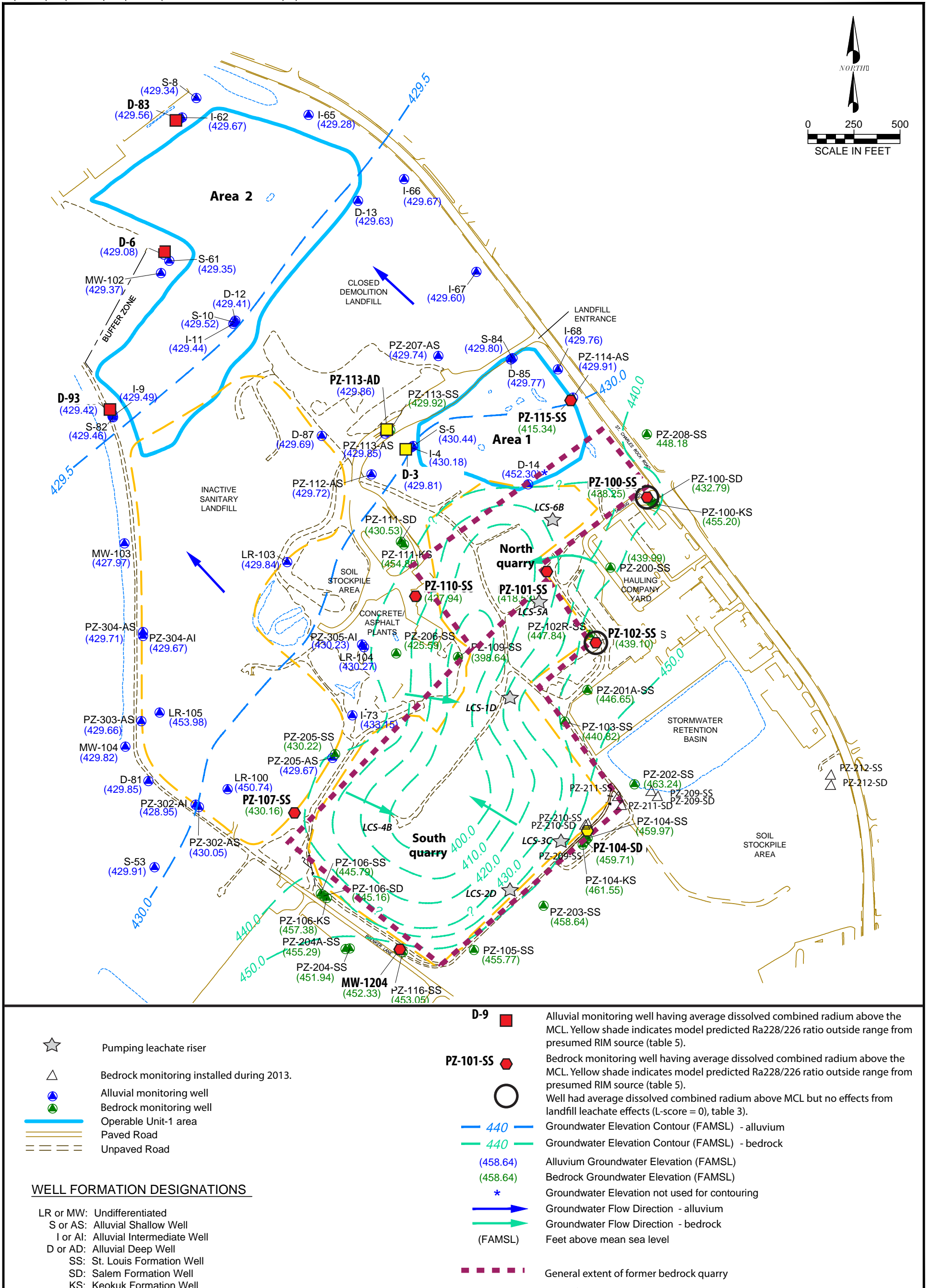
Figure 14. Monitoring wells with average dissolved combined radium above the maximum contaminant level (MCL) and degree of landfill leachate effects in those wells, and results of radium isotope mass balance in relation to water levels measured during July 2012.
