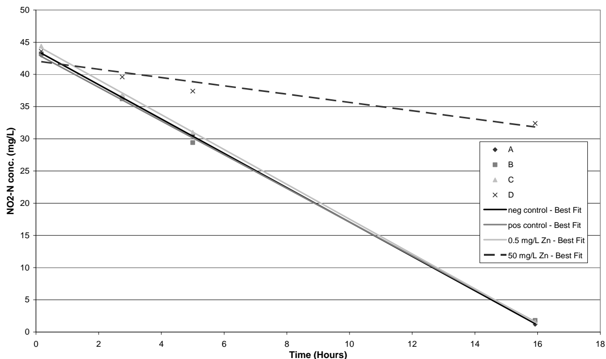
Figure 15. Plot of Nitrite concentration (mg/L) versus Time (hours) with linear regression shown.
