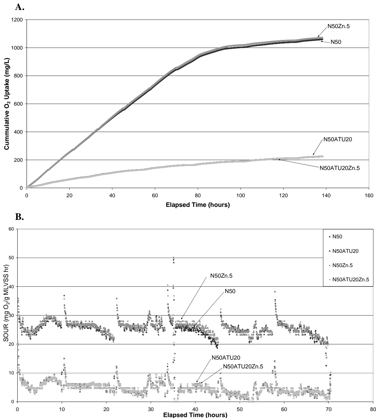
Figures 3A & 3B. Cumulative Oxygen Uptake (A) and SOUR(B) versus Time for Zinc at 0.5 mg/L (Replicate Experiment #1)
