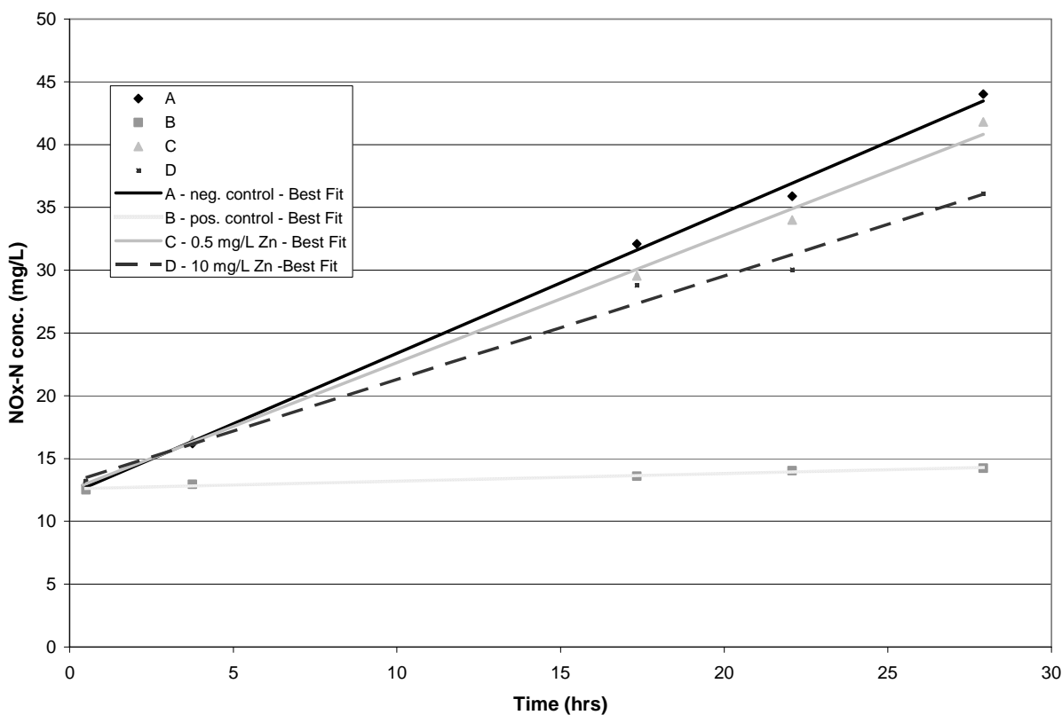
Figure 10. Concentration of \text{NO}_x\text{-N} (mg/L) verses Time (hours) with linear regression.
