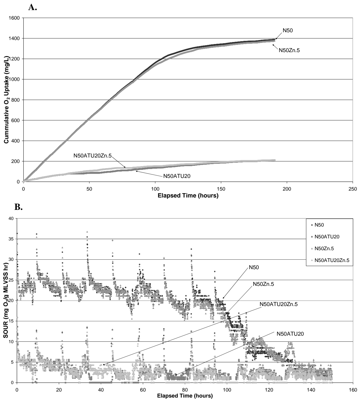
Figures 4A & 4B. Cumulative Oxygen Uptake (A) and SOUR (B) versus Time for Zinc at 0.5 mg/L (Replicate Experiment #2)
