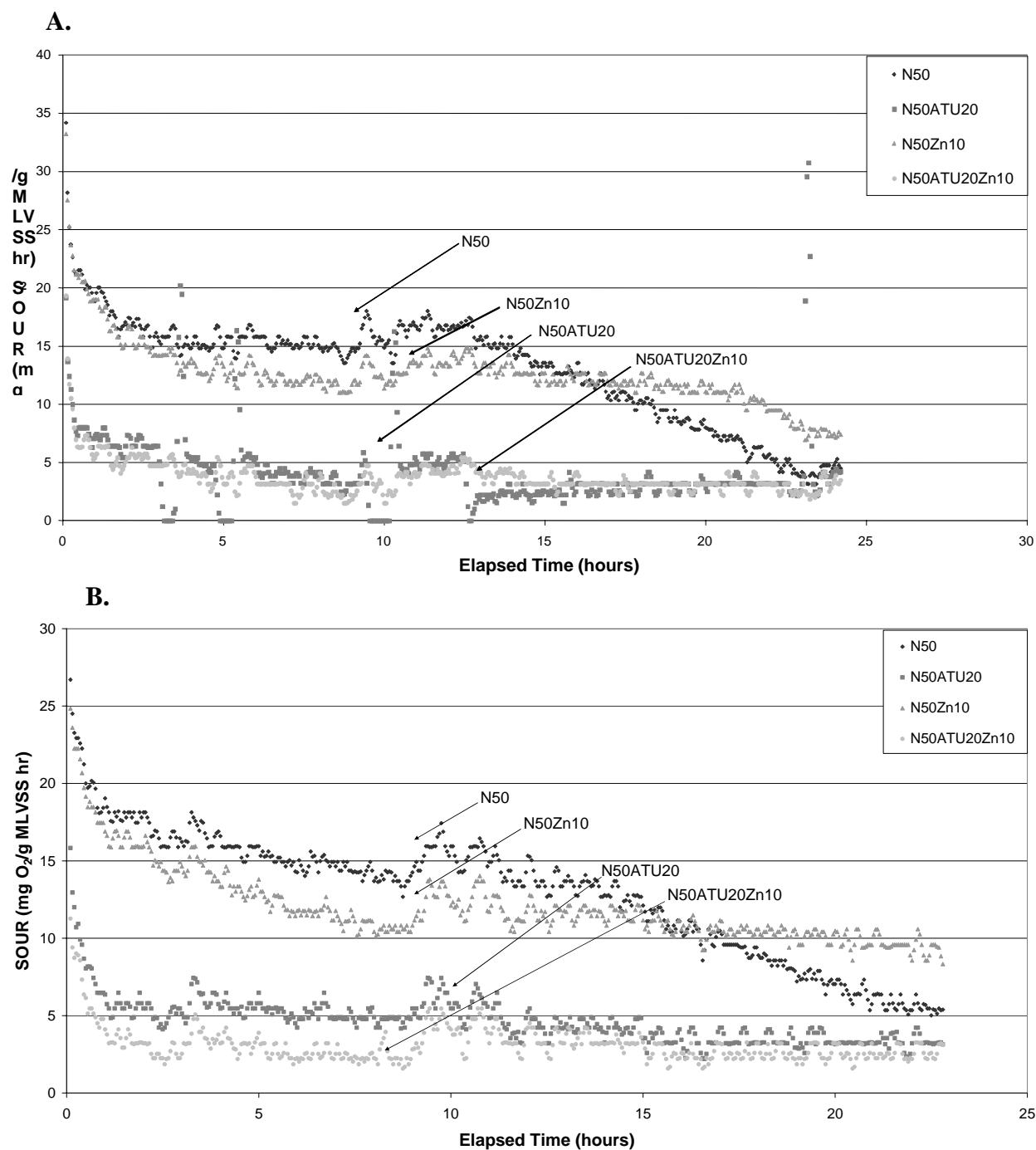
Figure 2. Specific Oxygen Uptake Rate versus Time for Zinc at 10 mg/L diluted with Secondary Effluent (A) or Tap Water (B)
