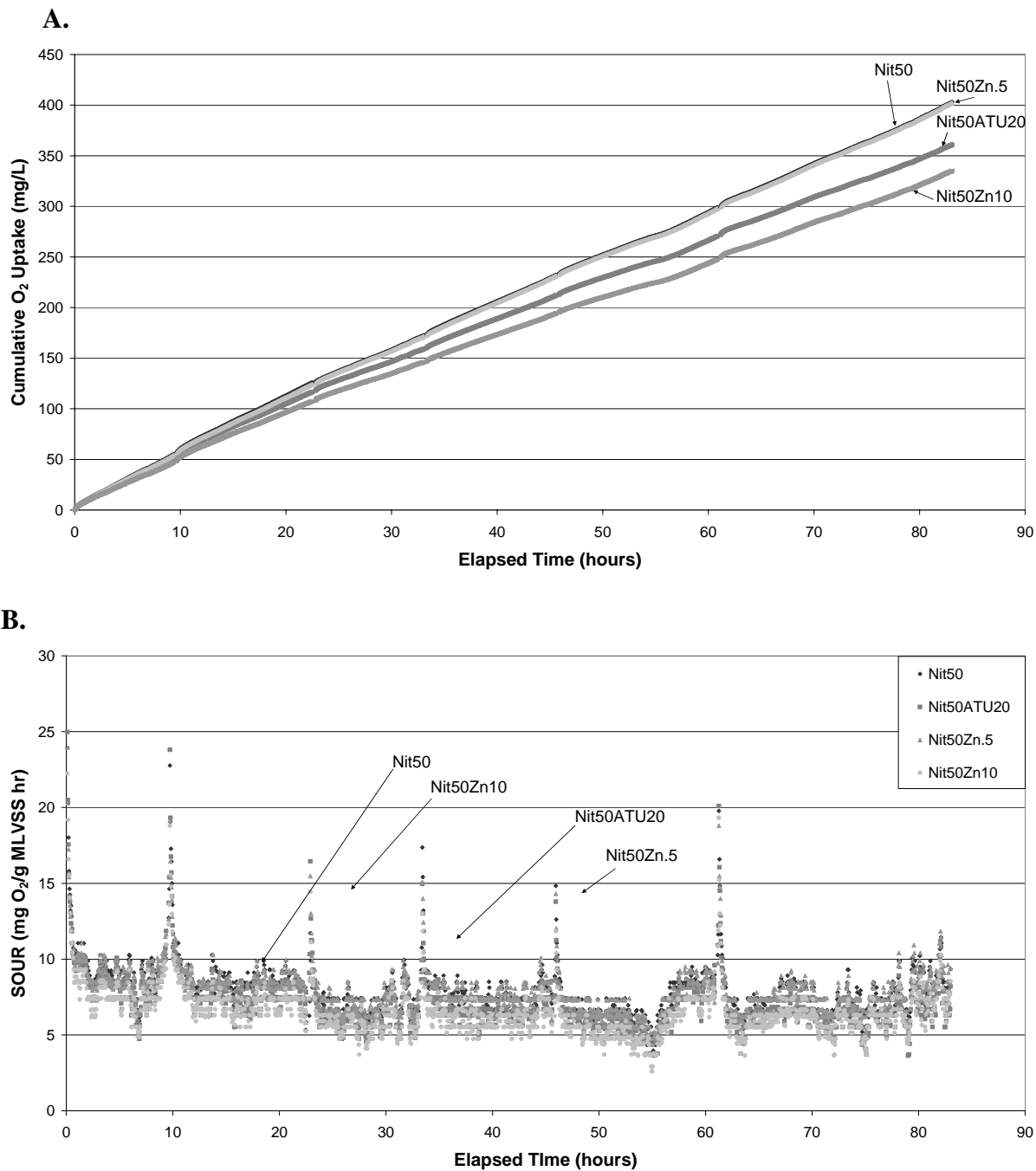
Figures 6A & 6B. Cumulative Oxygen Uptake (A) and SOUR (B) versus Time for the Experiment Assessing the Effect of Zn on NOB
