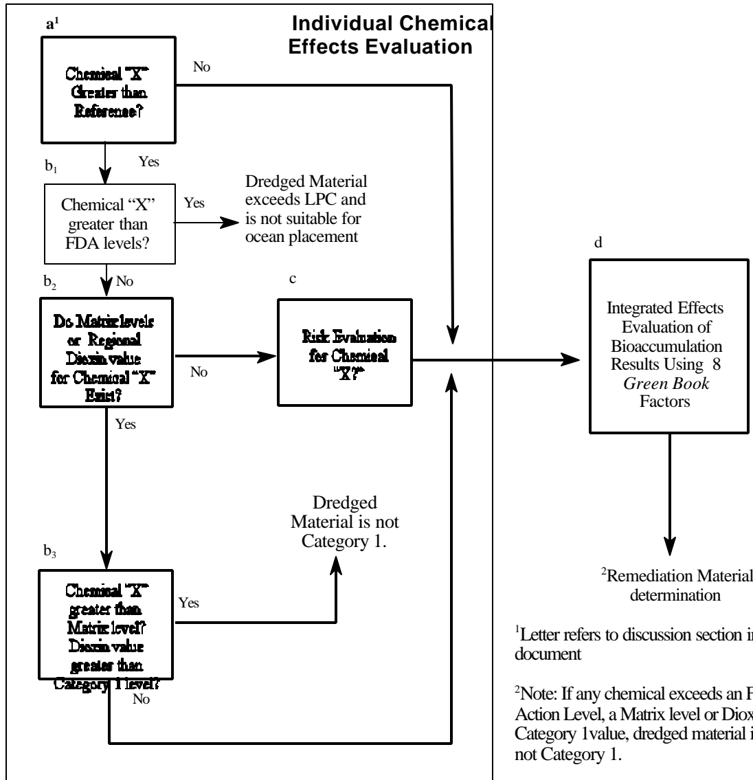
Figure 1 EPA Region 2/CENAN Framework for Evaluating Bioaccumulation Test Results for the Passenger Ship Terminal.
