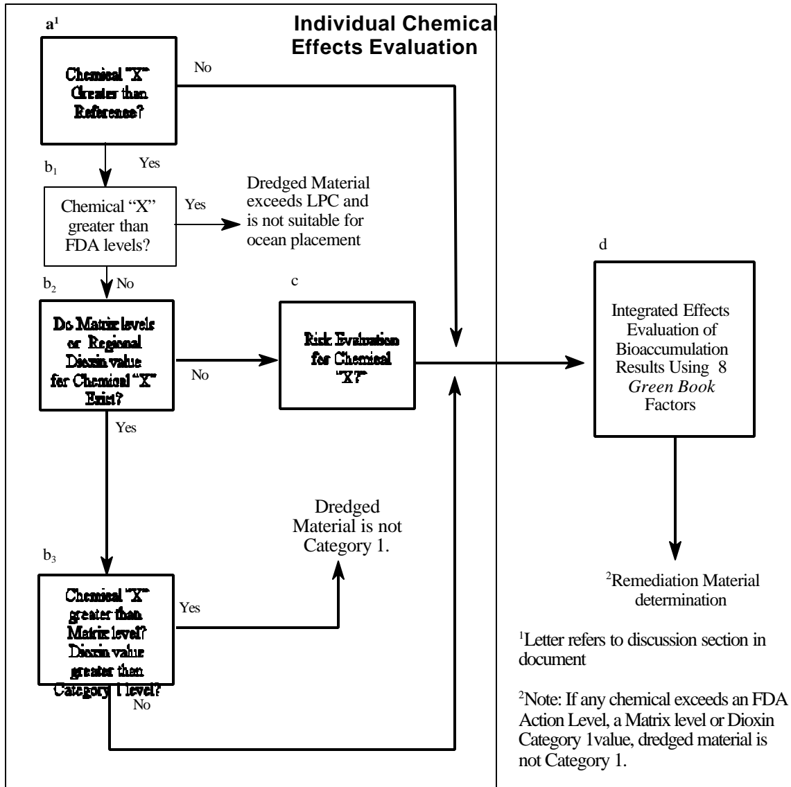
Figure 3 EPA Region 2/CENAN Framework for Evaluating Bioaccumulation Test Results for the National Parks Service, Ellis Island Ferry Slip.
