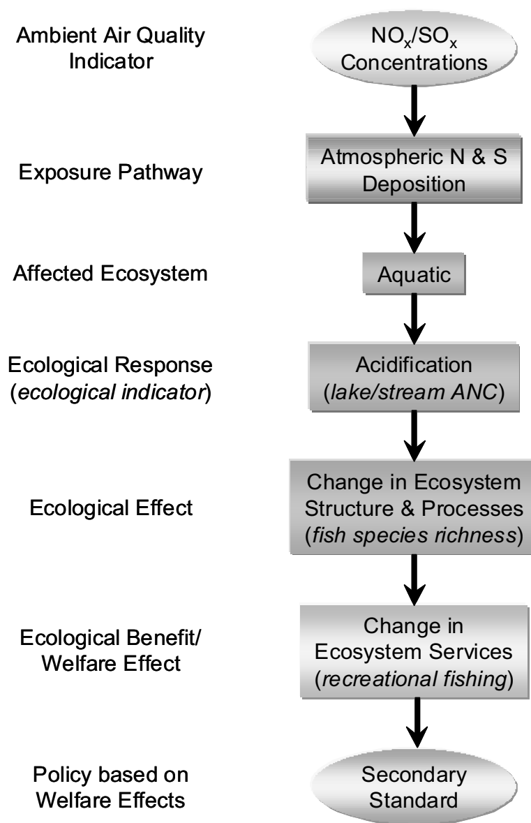
Figure D-1. Conceptual model showing the relationships among ambient air quality indicators and exposure pathways and the resulting impacts on ecosystems, ecological responses, ecological effects, and finally, on the quality of a particular activity (e.g., recreational fishing) known to influence public welfare.
