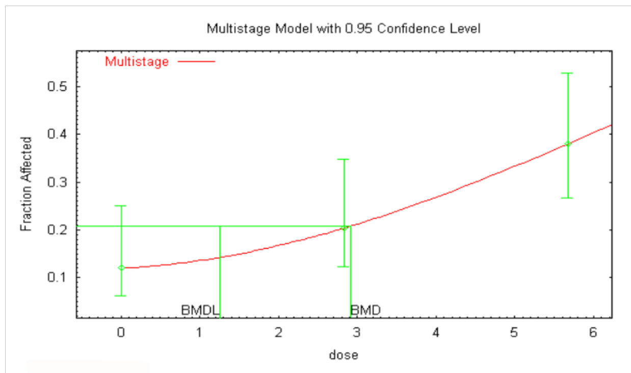
Figure A.4.1. Fitted 2 nd -degree multistage model, and data means and standard errors.
