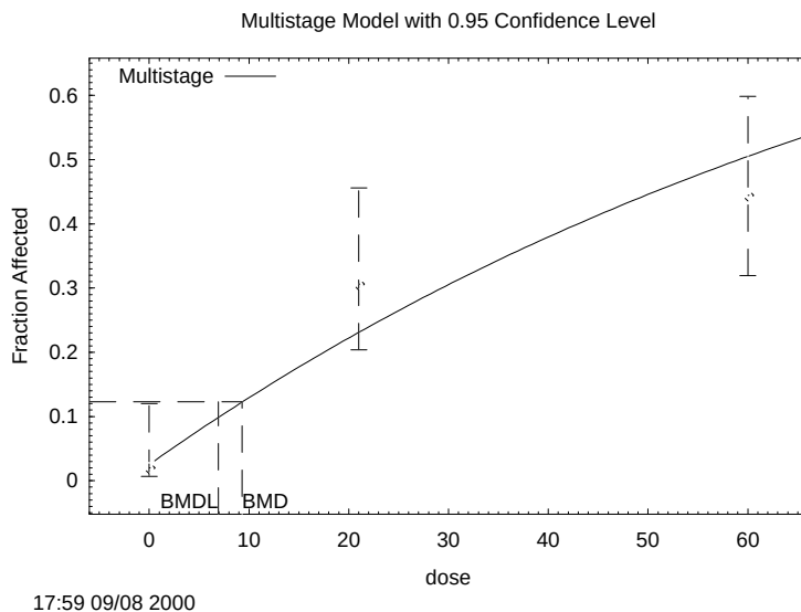
Figure A-2.3 Example data with 95% confidence limits, and second degree multistage model fit.
