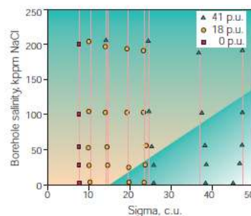
□ Processing accuracy. Benchmark measurements were made to assess the accuracy of the algorithm in computing formation and borehole sigma, porosity and borehole salinity. Sigma measured with the RST-A tool versus assigned database sigma ( left ) shows average errors are small—0.22 c.u. Sigma measured at the EUROPA facility in Aberdeen ( middle ) again shows excellent agreement with the assigned values. Comparison of RST-A tool sigma ( right ) versus borehole salinity shows that corrected sigma is independent of borehole salinity—vital for time-lapse surveys or log-inject-log operations. In the crossover region ( shaded area ), formation sigma approaches or even exceeds borehole sigma. Historically, pulsed neutron capture tools erroneously identify the borehole decay as formation sigma and formation decay as borehole sigma in this region. However, the RST dynamic parameterization method solves this long-standing problem, correctly distinguishing between formation and borehole sigma components.
