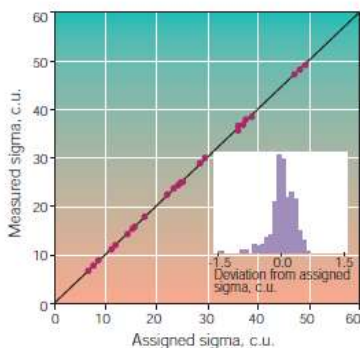
□ Processing accuracy. Benchmark measurements were made to assess the accuracy of the algorithm in computing formation and borehole sigma, porosity and borehole salinity. Sigma measured with the RST-A tool versus assigned database sigma ( left ) shows average errors are small—0.22 c.u. Sigma measured at the EUROPA facility in Aberdeen ( middle ) again shows excellent agreement with the assigned values. Comparison of RST-A tool sigma ( right ) versus borehole salinity shows that corrected sigma is independent of borehole salinity—vital for time-lapse surveys or log-inject-log operations. In the crossover region ( shaded area ), formation sigma approaches or even exceeds borehole sigma. Historically, pulsed neutron capture tools erroneously identify the borehole decay as formation sigma and formation decay as borehole sigma in this region. However, the RST dynamic parameterization method solves this long-standing problem, correctly distinguishing between formation and borehole sigma components.
