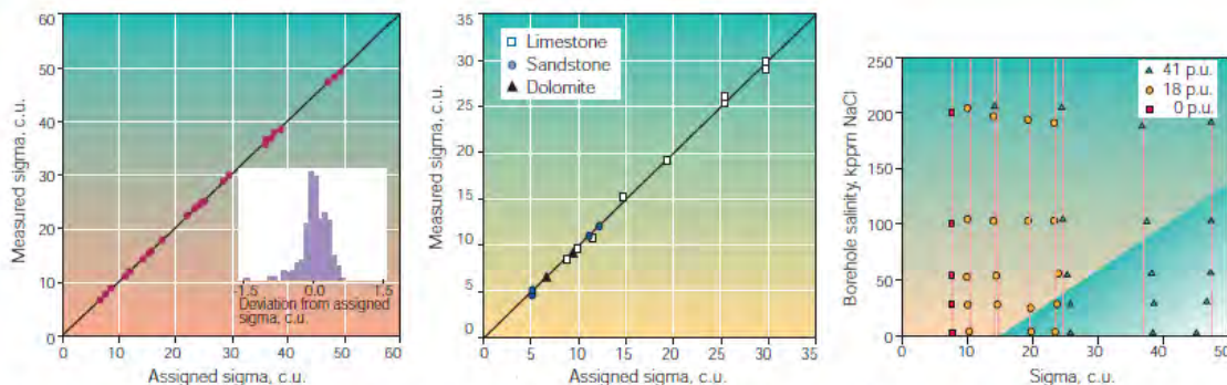
□ Processing accuracy. Benchmark measurements were made to assess the accuracy of the algorithm in computing formation and borehole sigma, porosity and borehole salinity. Sigma measured with the RST-A tool versus assigned database sigma ( left ) shows average errors are small—0.22 c.u. Sigma measured at the EUROPA facility in Aberdeen ( middle ) again shows excellent agreement with the assigned values. Comparison of RST-A tool sigma ( right ) versus borehole salinity shows that corrected sigma is independent of borehole salinity—vital for time-lapse surveys or log-inject-log operations. In the crossover region ( shaded area ), formation sigma approaches or even exceeds borehole sigma. Historically, pulsed neutron capture tools erroneously identify the borehole decay as formation sigma and formation decay as borehole sigma in this region. However, the RST dynamic parameterization method solves this long-standing problem, correctly distinguishing between formation and borehole sigma components.
