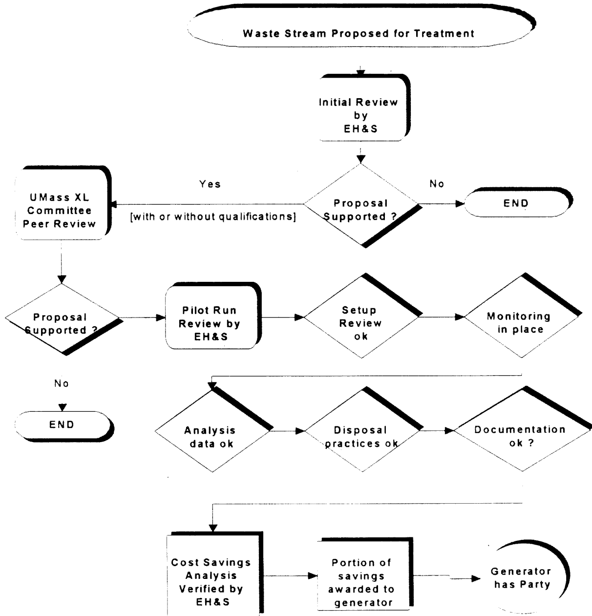
Project XL Preliminary Proposal Flow Chart for Small-Scale Hazardous Waste Treatment
